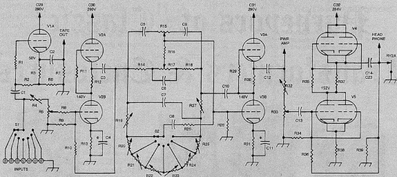
FIGURE 5: Power-supply schematic.
