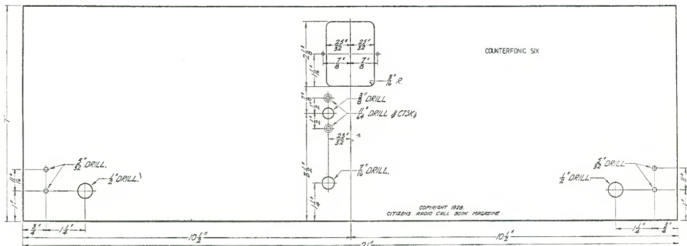
Figure 4. Front panel for this receiver may be made up from the specifications shown on the front panel sketch, although the front panels are available in drilled and engraved form, thus minimizing labor
