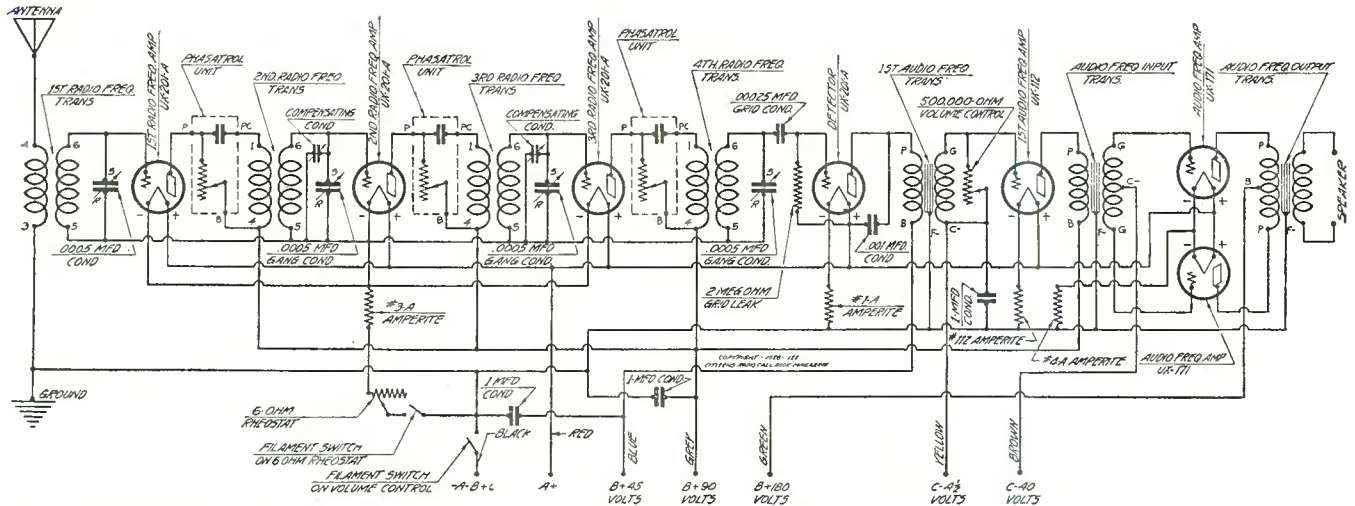
Figure 2. Electrical connections of the Phasatrol DeLuxe Seven may be found by consulting the schematic diagram given above
