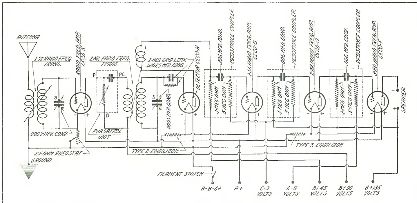
Figure 3. In this drawing are shown all of the electrical connections required for hooking up this receiver
