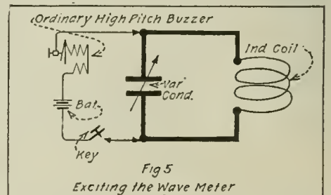
Hook-up for Exciting the Wave Meter so That It Will Emit Waves of Known Length.
