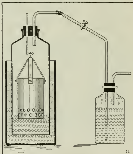
Sectional View of Gas Generator.
