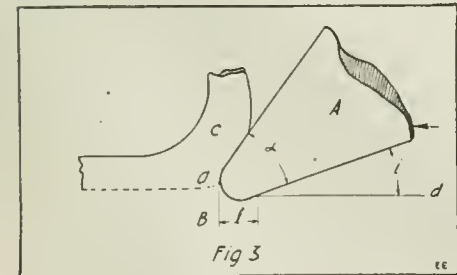
Further Illustrating the Similarity of a Chisel Cutting into a Piece of Metal to the Two Cutting Edges of a Twist Drill.
