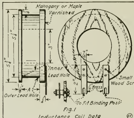
Details of Inductance Coils, Three of Which Are Used to Give the Wave Meter a Desirable Range.
