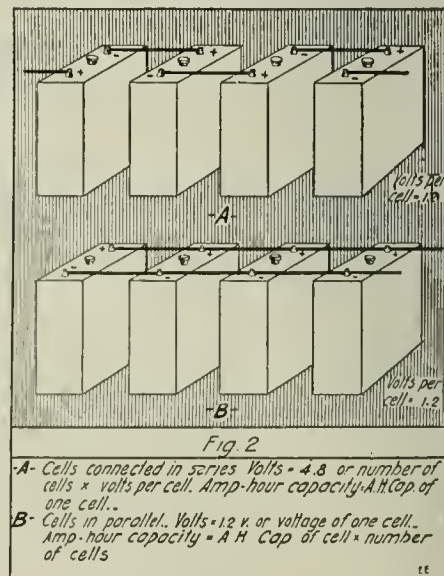
Diagram Showing Voltage and Amperage With Series and Parallel Connections of Battery Cells.
