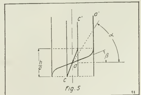
Diagram Used in Explaining the Value of the Angles of Grinding of Twist Drills.
