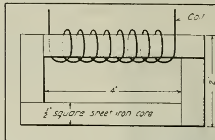
How Choke or "Ballast" Coil Is Made for Use in an A. C. Arc Lamp Circuit. This Takes the Place of the Resistance Coil in a D. C. Arc Lamp.
