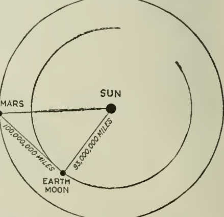
Fig 5. Relative Positions of Mars, Sun and Earth—Moon at the Time When the Earth Can Be Best Observed from Mars. The Earth as Well as the Moon in This Position Shows in the Form of a Crescent. (See Fig. 4.)
