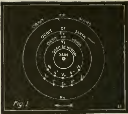
Fig 1. Diagram Showing Relative Positions of Mars and the Three Inner Planets, Earth, Venus, and Mercury, the Three Morning and Evening Stars of Mars. Assuming Mars to Be in the Position M 0 the Planets Are Best Seen When on the Near Side of Their Orbits, Positions E, E', E'' and E 3 for Earth and V, V', V'' and V 3 for Venus. At E 1 and E 2 Earth is Invisible from Mars, Being in Inferior and Superior Conjunction with the Sun Respectively. At E 1 and E 2 It is at its Eastern and Western Elongations Respectively and at E' and E'' It is at the Greatest Brilliance. When Venus is at its Greatest Brilliance V' and V'' and the Earth is in the Far Part of Its Orbit. Beyond E 1 and E 2 Venus Appears Brighter to the Martians Than Our Own Planet, but When the Earth is Near E' and E'' It Surpasses Venus in Brightness Because It is Then Considerably Nearer to Mars.
