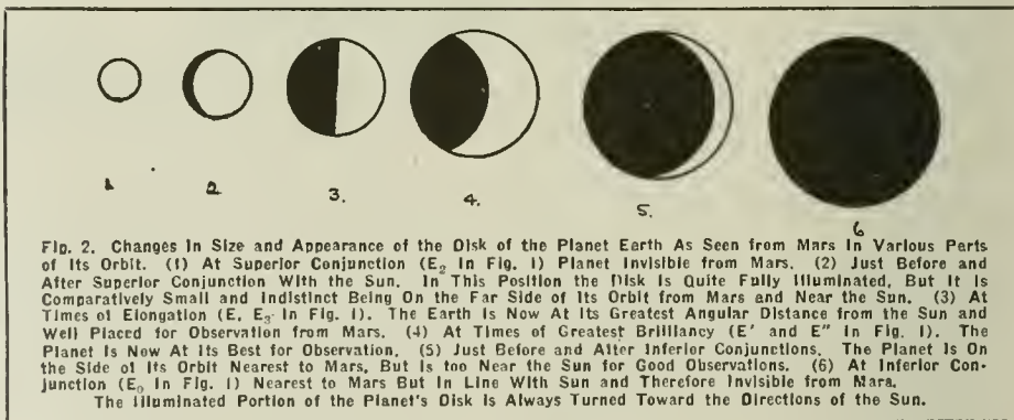
Fig 2. Changes in Size and Appearance of the Disk of the Planet Earth As Seen from Mars in Various Parts of Its Orbit. (1) At Superior Conjunction (E 2 in Fig. 1) Planet Invisible from Mars. (2) Just Before and After Superior Conjunction With the Sun. In This Position the Disk is Quite Fully Illuminated, But It is Comparatively Small and Indistinct Being on the Far Side of Its Orbit from Mars and Near the Sun. (3) At Times of Elongation (E, E 3 in Fig. 1). The Earth is Now at its Greatest Angular Distance from the Sun and Well Placed for Observation from Mars. (4) At Times of Greatest Brilliance (E' and E'') in Fig. 1). The Planet is Now at Its Best for Observation. (5) Just Before and After Inferior Conjunctions. The Planet is on the Side of Its Orbit Nearest to Mars, But is too Near the Sun for Good Observations. (6) At Inferior Conjunction (E 1 in Fig. 1) Nearest to Mars But in Line With Sun and Therefore Invisible from Mars. The Illuminated Portion of the Planet's Disk is Always Turned Toward the Directions of the Sun.
