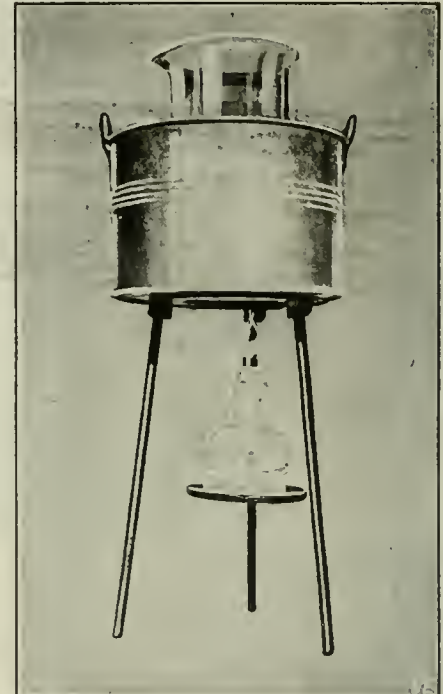
Fig. 2. Set-up of Simple Apparatus Utilized in Making the "Milk Test" for Butter.
