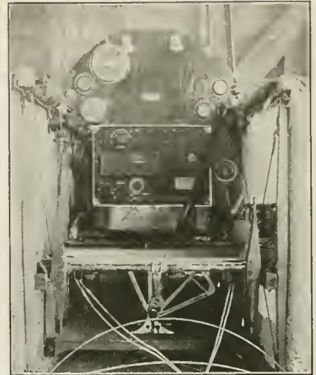
The Wireless Telephone Apparatus (Outlined in White Square) Installed in Cock-pit of Airplane. It Takes up But Little Room and Has Such a Small Weight as to Be Insignificant, Compared to the Lifting Power of the Plane.
