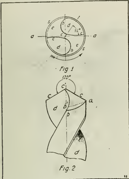
In the Present Article the Author Discusses the Theory of Twist Drills, the Shape of the Grooves, the Pitch of the Cutting Edges, Et Cetera. The Lips C-C May Be Considered as the Cutting Edges of Two Chisels, Which Turn about the Axis of the Drill.
