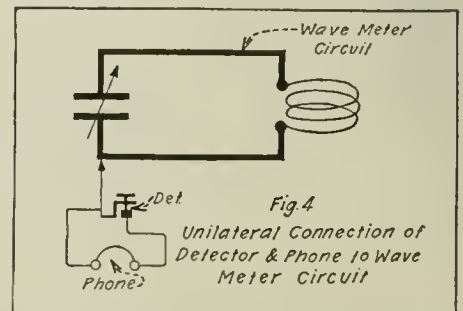
Usual Hook-up of Detector and 'Phones in Unilateral Fashion, Where There is Sufficient Energy to Actuate Detector Properly.
