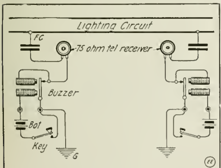
Simple Buzzer Telegraph for Use on Lighting or Power Circuits.
