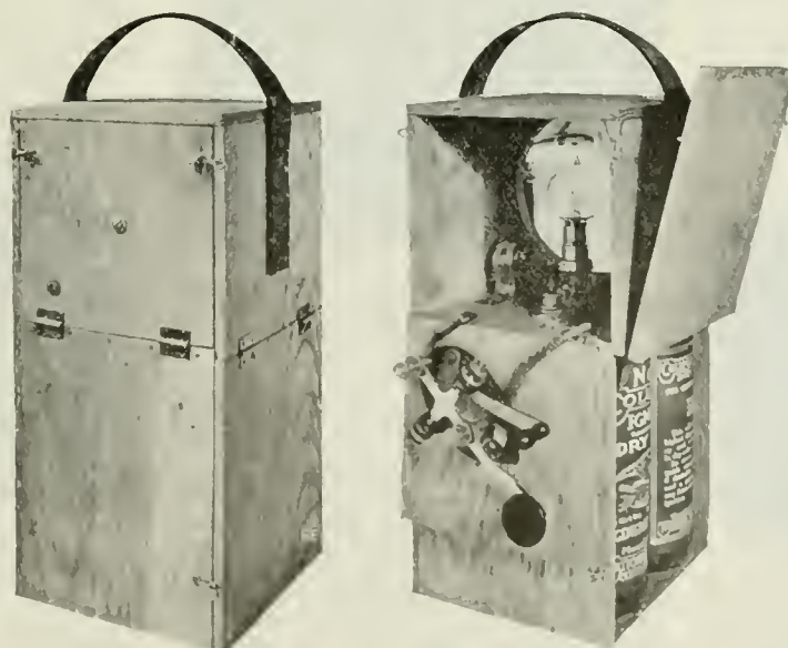
A Military Signal Projector Having a Range of 25 Miles. It is Fitted with 5-In. Mangin Mirror and 6-Volt 12-c.p. Mazda C Lamp. A Telegraph Key Controls the Lamp Circuit.
