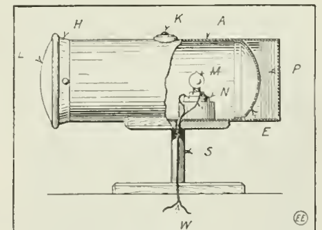
This Nifty Electrical Window Attraction Comprises a Large Dummy Flash-Light, the Lamp Within It Being Winked On and Off By a Flasher.
