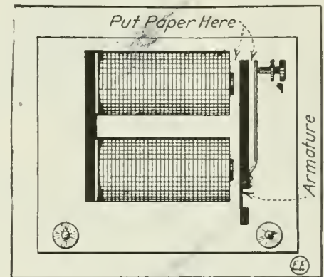
Any Buzzer Can Be Made to Give a High Tone By Placing Paper on Either Side of the Armature, As Shown.
