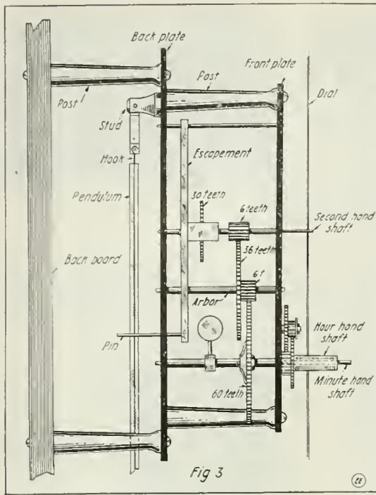
Side View of Complete Electric Clock Movement, Illustrating Suspension of Pallet Levers, Escape Wheel and Pendulum.
