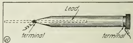
If You Carry a Metal Magazine Pencil You Are a Potential Electrician. Connect a Wire to the Case and Lead, and Presto! You Have An Adjustable Rheostat.
