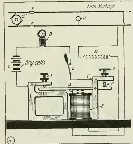
When the Line Voltage Fails the Relay Closes an Alarm Bell Circuit, the Bell Being Placed At Any Point Desired.
