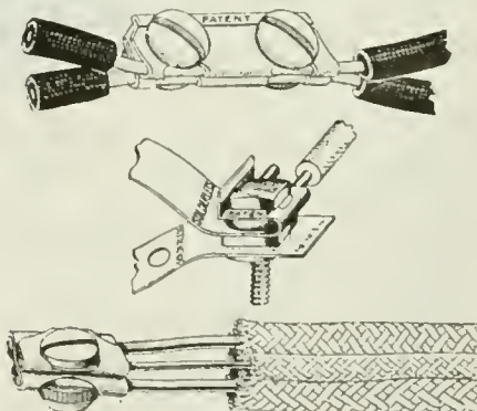
A Clever Wire Clamp Which Requires No Solder. Particularly Useful to Electrical Experimenters for Making Various Circuit Changes Quickly.
