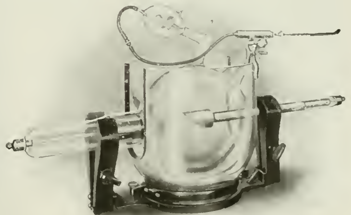
Hydrogen Thru a Mercury Valve. Vacuum Is Adjustable. Hydrogen Thru a Mercury Valve Vacuum Is Adjustable.
