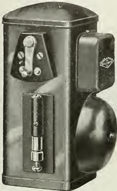
An Electric Fire Detector Which Can Be Left at Any Point Desired, Such as in the Kitchen, and as Soon as Blaze Occurs the Alarm Bell Rings. It Utilizes a Fine Mercury Column, Which Expands When Heated, Thus Closing the Bell Circuit. It Will Also Announce a Drop in Temperature.
