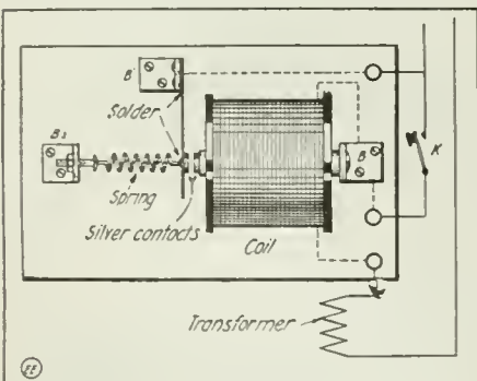
Due to the Fact that the Alternating Current from the Transformer Line Flows Thru the Key Magnet Coil, the Final "Break" of the Circuit Occurs at the Zero Part of the Cycle.
