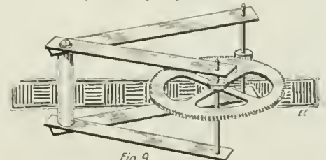
Handy Jig for Matching Up Gears and Determining Their Correct Spacing Between Arbor Centers Before Drilling the Main Frame.
