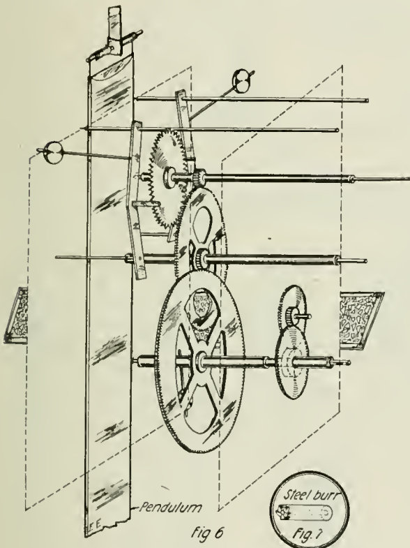
Phantom View of the Modified Clock Movement As Adapted to Be Driven by Electricity. Fig. 7 Shows Detail of Steel Burr for Milling Ends of Arbors.
