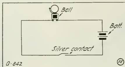
A Simple Yet Difficult Problem. It Is Required to Break This Circuit With a Minimum of Sparking and the Interrupter Is a Delicately Mounted One, Easily Vibrating With a Slight Jar.
