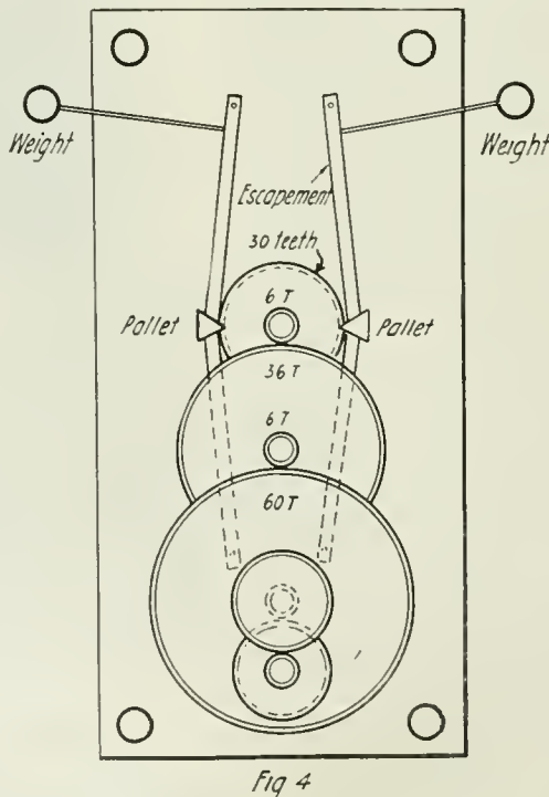
Here, "Bugs," We See the Arrangement of the Electric Clock Gear Train. It's Simple We Assure You.
