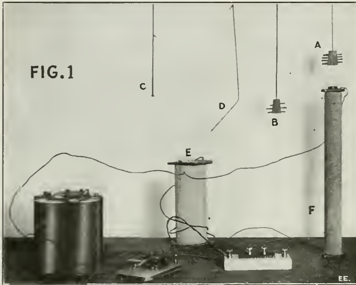
FIG. 1.—Apparatus Used by the Author for Demonstrating that Rotary Motion Is Created in Suspended Magnetic Objects When the Current in a Magnet Coil Below Them Is Suitably Interrupted.
