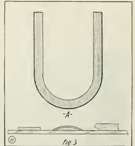
Demonstrating that There is an Outward Flow of Currents from the Center of a Magnet. To Make a "Magnetograph" Several Objects Are Placed on a Photograph Plate Beneath the "U"-Bend, and Left in the Dark for Several Weeks.
