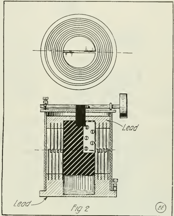
Fig. 2. Unique Variable Condenser, Suitable for Radio and Other Circuits. The Movable and Stationary Plates (Spirals of Brass Ribbon) Are Both Held by Molded Lead at Top and Bottom of the Condenser, As Shown. Oil Dielectric Can Be Used, Giving As High As Five Times the Capacity With Air.
