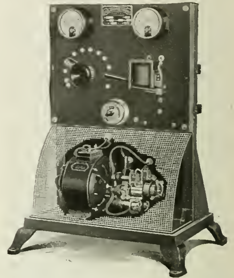
One of the Jobs We All Hate to Tackle Is Charging Storage Batteries. In This Simple Automatic Device a Motor Drives a Commutator in Such a Way that the Alternate + and - A. C. Pulses Are All Rectified or Converted Into Direct Current.
