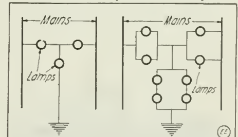
A Kick-Back Preventer Made From Lamps Properly Connected.
