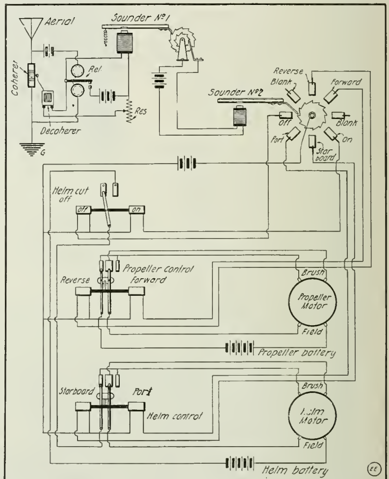
Lay-Out of Circuits, Including Coherer and Sensitive Relay. As Successfully Used in the Radio Control of the Model Boat Illustrated and Described in the Present Article.
