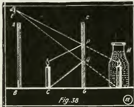
How a Person at "E" Can See a Candle, Invisible at "C", and Apparently Burning Inside a Bottle of Water at "M."
