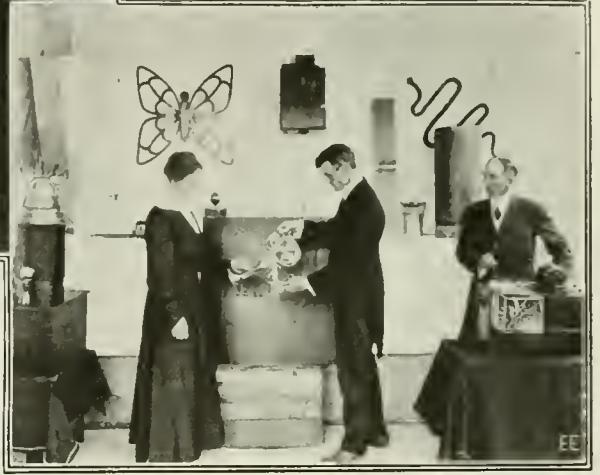
The Photograph Shows the Lighting of An Ordinary Candle by Means of a Stream of Water. In Connection With This Experiment, the Lecturer Becomes a Human Dynamo, Lighting Arc Lights by Holding the Carbons In His Hands and Handling 3,000,000 Volts of Electricity.
