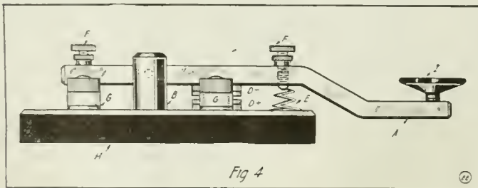
View of Assembled Radio Transmitting Key.
