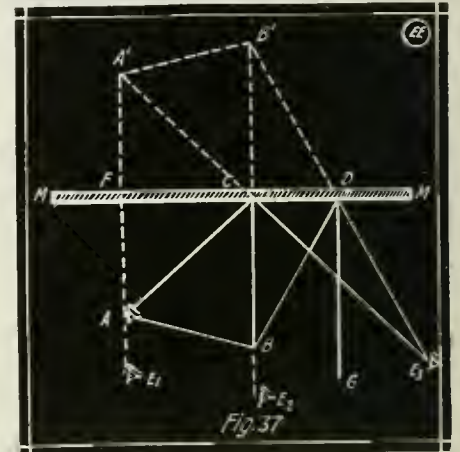
Analysis of the Principle of Mirrors. Each Point of An Image in a Plane Mirror Is As Far Behind the Mirror As the Corresponding Point of the Object Is In Front of the Mirror.
