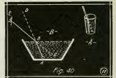
Due to the Change of Velocity of Light Rays Passing Thru a Denser Medium—Water In This Case—An Object Appears As Tho Bent or Misplaced.
