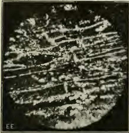
Fig. 1. Outcropping of Silver in Middle of Sulfide Strip. The Direction of the Electric Current Was Approximately Parallel to the Direction of the Lines of the Silver. This Picture Suggests the Possibilities of the Formation of Native Silver in the Earth.
