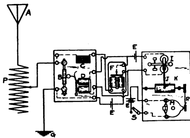
A-AERIAL E-BATTERY K-PEN L-CYLINDER S-SWITCH B-COHERER F-RELAY M-MOTOR R-PULLEY BAND C-CHOKE COIL I-SOUNDER P-TUNING COIL D-DECOHERER J-ARM
