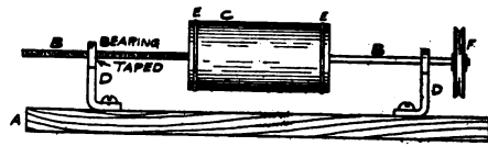
A-BASE D-BEARINGS B-BRASS ROD E-RUBBER BANDS C-CYLINDER F-PULLEY
