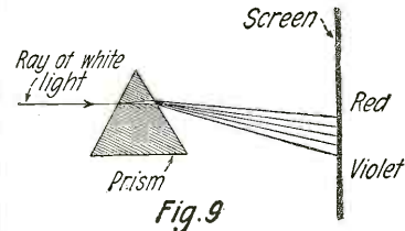
Showing How a Prism Refracts White Light and Resolves it Into Different Colors, Each Color Being Refracted a Different Amount on Account of Difference in Wave-lengths.
