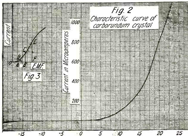
Characteristic Curve of a Carborundum Crystal Showing the Relative Current at Various Applied Potentials.
