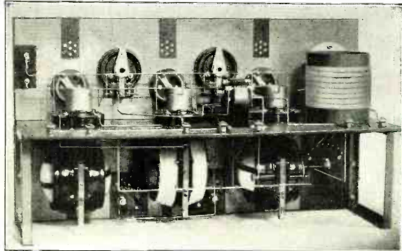
Here is a Real DX Receiver, Composed of a Two-Stage R. F. Amplifier and Regenerative Receiver. Note the Shielded Panel and Neat Wiring Arranged for Minimum Stray Capacity.
