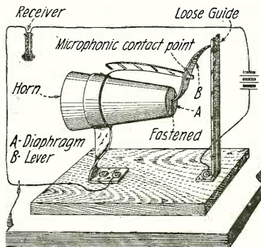
Fig. 3. A System of Contact Similar to That Used by Reis.
