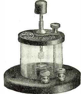
Pacent Crystal Detector
