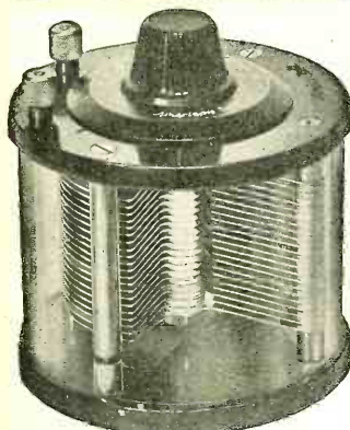
"Certified" American Bell Condenser
