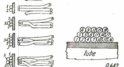
Method Used in Bank Winding. This is Fully Described in Answer to Question 642.
