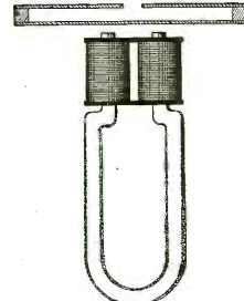
Fig. 13. A Receiver of the Magnetic Type Employing a Resonating Chamber in Conjunction with the Diaphragm.
