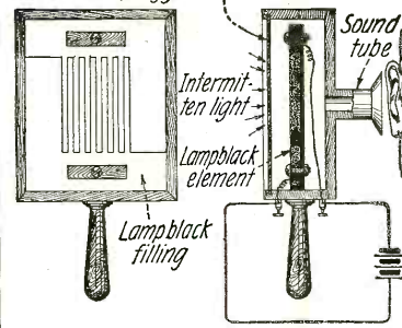
Figs. 17-18. Bell's Photophone. It Can Speak, Sing, See, Hear and Feel Electricity and Magnetism Aside from a Few Other Choice Accomplishments.
