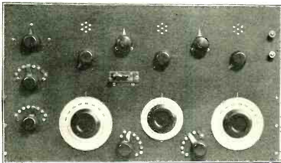
Here is a Real DX Receiver, Composed of a Two-Stage R. F. Amplifier and Regenerative Receiver. Note the Shielded Panel and Neat Wiring Arranged for Minimum Stray Capacity.
