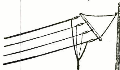
Showing the Distribution of R. F. Current in a Four Wire Flat Top Inverted "L" Antenna.
