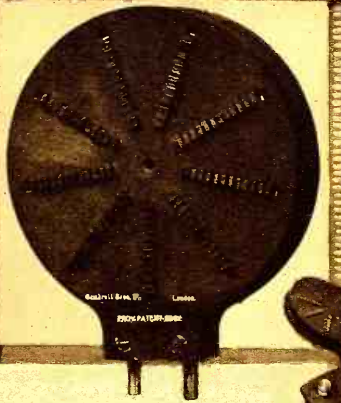
Left: A fixed inductance coil of the multi-layer type with plug attachment. An air space is left between each layer similar to the Morecroft inductance. Below: A small receiving set employing three of these coils.
