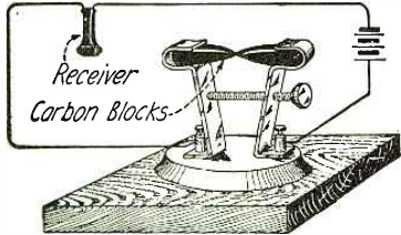
Fig. 22. Another Form of Carbon Microphone Provided with an Adjusting Screw.
