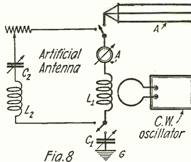
Fig. 8 System Used of the Measurement of Antenna Resistance.
