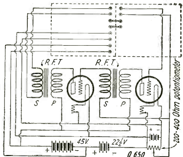
The Proper Way of Connecting Two Stages of Radio Frequency to a Westinghouse R.C. Receiver is Shown Above. It is Not Necessary to Disturb the Interior Wiring of the Set, All of the Connections Being Made Directly to the Binding Posts. A 45-Volt "B" Battery Is Used for All Four Amplifying Tubes.
