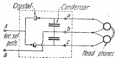
This Is a Good Stunt and Well Worth Trying. Both Halves of the Incoming Wave Are Made Use of.
