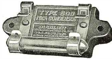
Dubilier Type 600 Condenser
