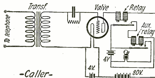
The Caller Circuit Used in Conjunction with the Main Receiver. The Bell is Arranged to Ring on the Wave-Length for Which the Receiver is Tuned.
