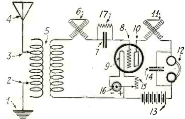
Fig. 2. The Circuit Hook-up of the Above Receiver. The Numbers Here Correspond to Those on the Photograph.
