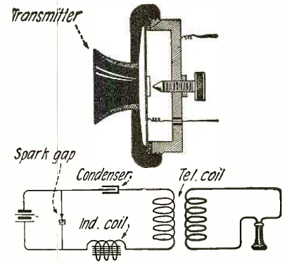
Fig. 12. In This Arrangement Upon Speaking Against the Diaphragm, Variations Are Set Up in the Length of the Gap, Thus Causing Corresponding Surges in the Coupled Circuit.
