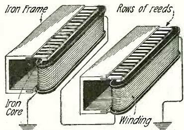
Fig. 5. Bell's Electric Harmonica, the Principle Being that of the Sympathetic Action of Vibrating Members.
