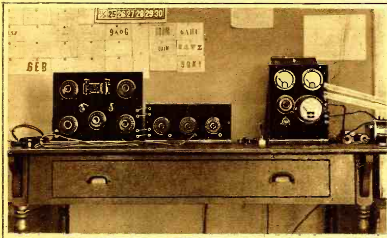
This Station is Neat in Appearance Due Particularly to the Absence of Unsightly Wiring. The Short- and Long-Wave Receiver is on the Extreme Left Followed by the Detector-Amplifier Unit. The 15-watt C.W. Transmitter on the Right Radiates 3 1/2 Amperes on 200 Meters.
