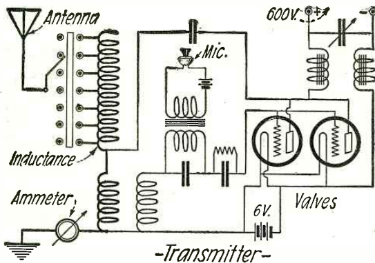
The Small Transmitter Developed in France Which Well Lends Itself to the Transmission of Voice Over Power Lines or Through the Air.
