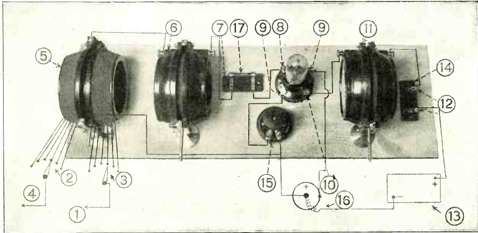
Fig. 1. Showing the Standard Layout for a Set Employing Two Variometers and a Variocoupler. The Wiring is Clearly Shown So That None Should Find Difficulty in Connecting Up a Similar Outfit. Each Numbered Instrument is Mentioned in This Article.
