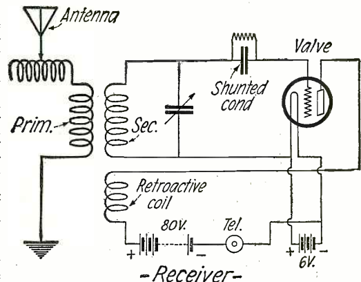
The Circuit of the Receiver. For Reception Over High Power Transmission Lines the Receiving Aerial Is Placed Parallel to Them.
