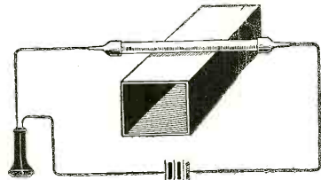
Fig. 19. One of Hughes' Microphones. The Glass Tube is Filled with Bronze Powder. Its Action is Similar to That of the Carbon Grain Type of Microphone.
