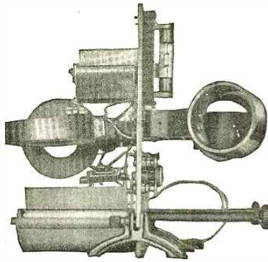
Front and Side Views of Mr. Groves' Super-Regenerator. The Two Honeycomb Coils Are Mounted on the Rear of the Panel Directly Behind the Main Inductances. It Will Be Noted That a Myers Tube is Used with This Set.
