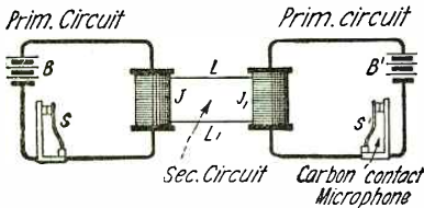
Fig. 23. A System Patented by Berliner in 1877 Using Carbon Contact Microphones, Batteries and Induction Coils, Similar to Systems in Use Today.
