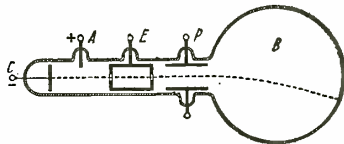
Fig. 38. Cathode Ray Tube and Bulb. C—Cathode or Negative Electrode. B—Highly Exhausted Bulb with Fluorescent Screen on its Spherical End. A—Anode. E—Baffle Plates. P—Deflecting Plates.
