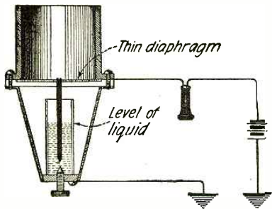
Fig. 6. A Receiver Produced by Gray. Vibration of the Diaphragm Caused Variations in the Distance Between Two Points Immersed in a High Resistance Liquid Varying the Battery Current in a Local Circuit.
