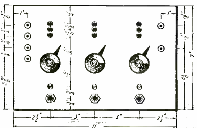
Dimensions for the Layout of the Panel.
