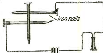
Fig. 20. The Hughe's Nail Microphone Its Function Resting on Imperfect Contact.
