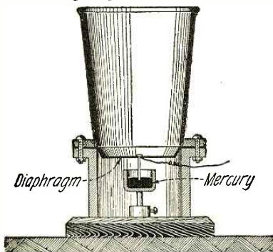
Fig. 7. Another Type of Transmitter Produced by Bell, the Action of Which Is Similar to the One Invented by Gray.
