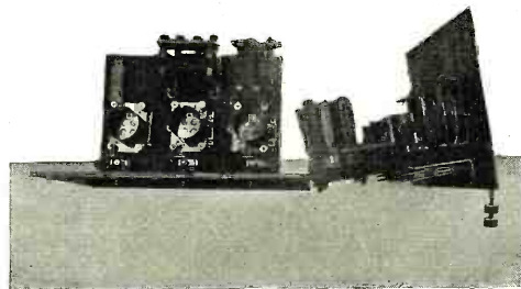
Interior View of the Detector-Amplifier Unit Clearly Showing the Arrangement of the Parts
