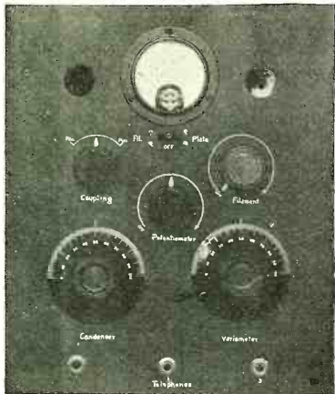
Front View of Mr. Norton's Super-Regenerative Receiver. This Set Incorporated the Use of a Potentiometer Which, However, is Not Necessary.
