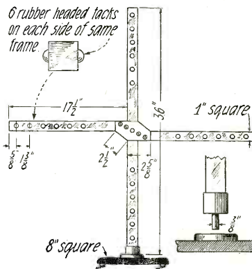
Further Details and Dimensions of the Portable Loop Series. Suitable Binding Posts Can Be Placed at the Bottom for Fastening the Wire.
