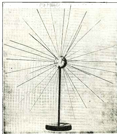
Fig. 43. A Golf Ball with Radial Wires in it to Represent an Electron with its Electrostatics.
