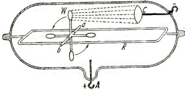
Fig. 36. Crook's Electron Mill. B—Highly Exhausted Bulb. C—Cathode or Negative Electrode. A—Anode or Positive Electrode. W—Little Rotor with Mica Vanes Which Rotates and Rolls Along Glass Rails R. Under Impulses of Electrons Radiated from Cathode.
