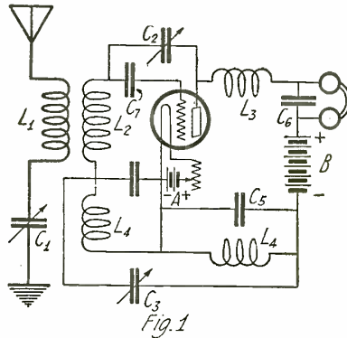
The Circuit of the Set Described in This Article. Capacity Feedback is Employed.
