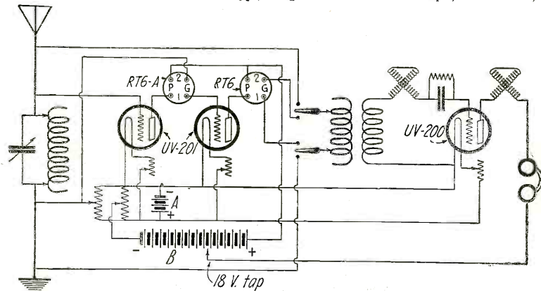
Hook-up of the DX Receiver. By Means of Two SPST Switches Only the Regenerative Set May Be Used. The Tubes May Be of Any Suitable Make, Such as Radiotron, Cunningham, etc.
