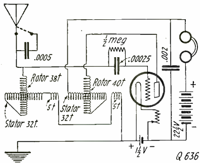
Diagram of the Aeriola, Sr. Receiver. Two Variometers Are Used, One as the Tuning Unit and the Other in the Plate Circuit.
