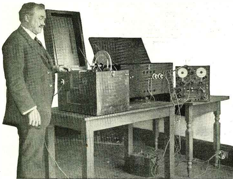
Mr. C. F. Jenkins and His Apparatus for the Transmission and Reception of Photographs by Radio. This Apparatus Copies Half-Tone Camera Studies from Flat Surfaces, Transmits Them, and at the Receiving End They Are Impressed on Common Photographic Plates.
