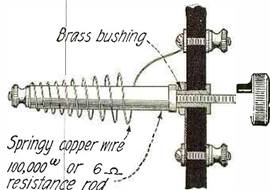
Here is a Unique Means of Varying a Resistance. This Makes a Very Effective Rheostat or Variable Grid Leak.
