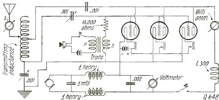
Here is Shown an Efficient 15-Watt Transmitter. The Colpitts Oscillator Circuit is Used and a Very Good Range Can Be Obtained.
