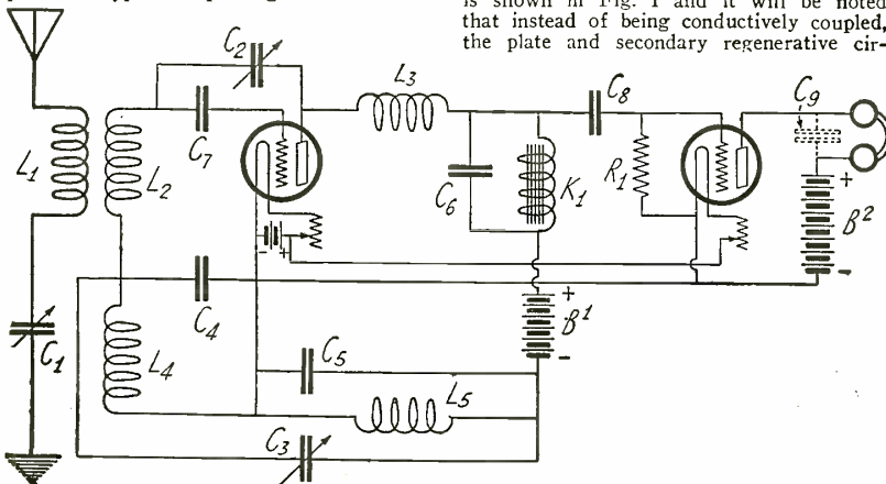
Feb. 2. The Same Circuit with the Addition of a One-Stage Choke Coil Audio Frequency Amplifier. Separate "B" Batteries Are Used for Each Tube.
