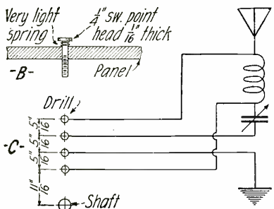
The Layout and Connections for the Series-Parallel Switch. Small Springs Underneath the Switch Points Provide the Necessary Friction Contact Against the Brass Strips.
