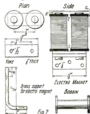
Details of the Electro-Magnets Used in the Selector.
