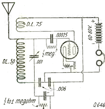
The New Flewelling Circuit. The Resistance Across the .006 Mfd. Condenser is Very Critical.
