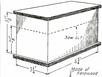
Details of the Cabinet Construction.
