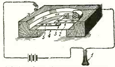
Fig. 2. The System of Contact Used in the Reis Speaking Phone, the Lower One Being Fastened to a Membrane Diaphragm.
