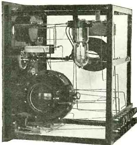
Rear View of the Receiver. The Leads from all the Instruments Connect to Separate Binding Posts so That Different Circuits May Be Tried. Note the Downward Suspension of the Tube Socket.
