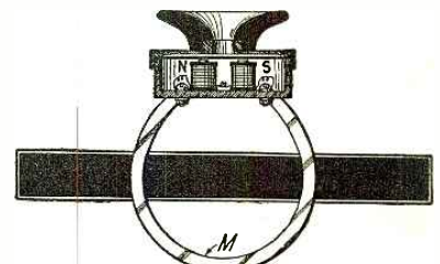
Fig. 11. A Modern Type of Adler's Phone in Which a Permanent Magnet Is Employed for Concentrating a Magnetic Flux Through the Diaphragm.
