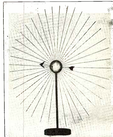
Another Illustration of an Electron in Motion.
