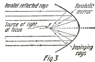
Showing How Source of Light at Focus of Parabolic Mirror Reflects Parallel Rays in One Direction.
