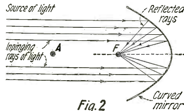
Light is More Intense at F Than at A (on Account of Concentrated Reflection at F) Even Though A is Nearer the Source of Light Than F.
