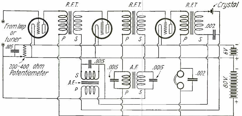
Here is the DeForest Reflex Circuit. Three Tubes Are Used for Five Stages of Amplification. A Crystal is Used for the Detector.
