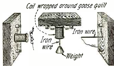
Figs. 8, 9, 10. Three Types of Phones Developed by Adler. Their Principles and Actions Are Very Interesting.
