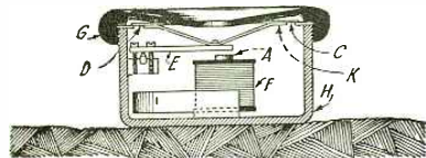
Fig. 15. S. G. Brown's Receiver Used Extensively Today in England. The Diaphragm is Made of Aluminum.
