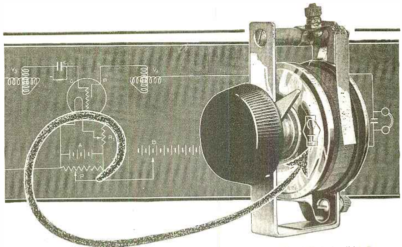
The C-H Radio "A" Battery Potentiometer.
