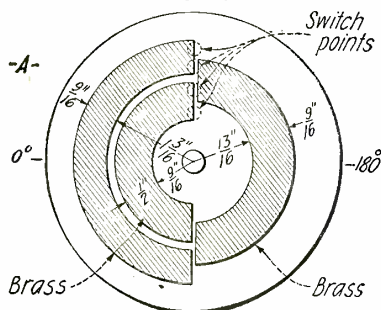
The Series-Parallel Switching Arrangement is Mounted Directly on the Rear of the Dial. This is a Very Good Scheme.
