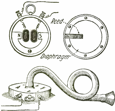
Fig. 14. The Gower Receiver. The First of the Watch Case Type. This Used a Magnet That Would Lift 11 Lbs.
