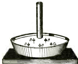
Fig. 39. Mayer's Magnet Experiment. Little Magnetized Needles Floating Vertically in Water were Caused to Arrange Themselves in a Pattern by a Magnet Held Over Them.
