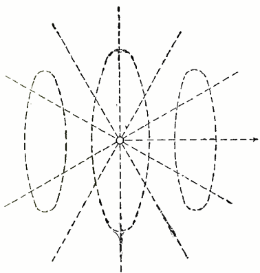
Fig. 41. Lines of Electric and Magnetic Force Around an Electron.
