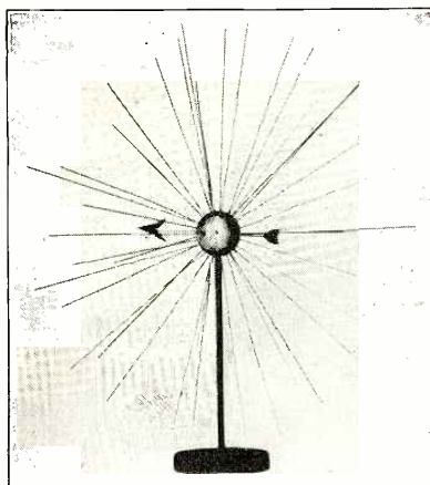
Fig. 44. A Golf Ball with Radial Wires in it to Represent an Electron in Motion. The Electrostatics Crowd Up Into the Equatorial Plane.
