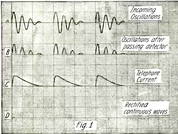
A Graph Illustrating the Original Energy Impressed Upon a Reception Circuit, its Character Upon Being Rectified, and the Consequent Telephone Current.
