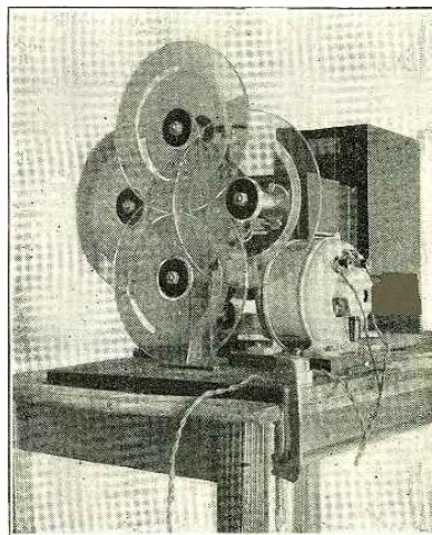
Part of the Receiving Apparatus. By Use of These Revolving Glass Rings, the Lights and Shadows of a Picture Are Built Up, Line by Line.
