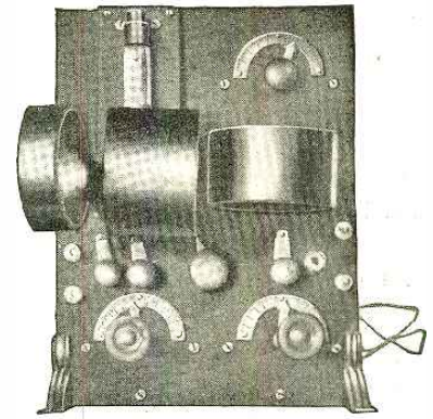
Front and Side Views of Mr. Groves' Super-Regenerator. The Two Honeycomb Coils Are Mounted on the Rear of the Panel Directly Behind the Main Inductances. It Will Be Noted That a Myers Tube is Used with This Set.
