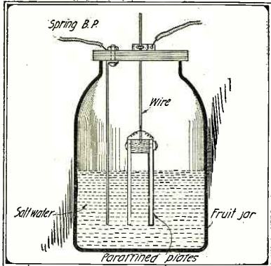
Simple Method of Constructing an Electrolytic Interrupter.
