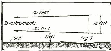
The Horizontal Loop of the Dimensions Shown Gave Fair Results.
