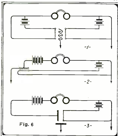
Hook-Ups Suggested for Trying Out the Tubes.
