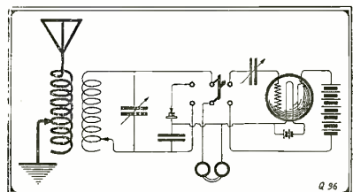
Hook-Up for Changing from Crystal to Audiotron.
