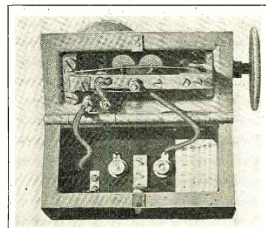
A German Buzzer Which Gives a Beautiful 600 Cycle Note.
