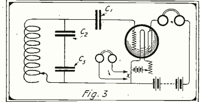
Fig. 3 Circuit Using Three Fixed Condensers.
