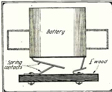
Method of Connecting the "B" Batteries.
