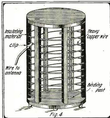
A Tuning Coil or Helix Used to Tune the Transmitting Circuit.
