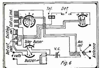
Showing the French Wave Meter Circuit.
