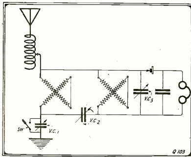
Special Hook-Up Using Two Variometers.
