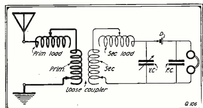
Showing the Use of a Primary and a Secondary Load.
