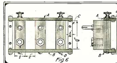
The Coil Mounting Is Constructed as Shown.
