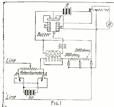
The Circuit Used in the Buzzer-Phone System.
