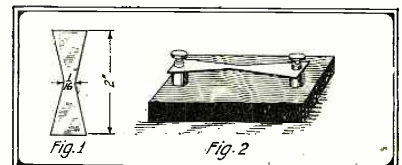
If You Want to Protect Your "B" Batteries Use a Fuse of This Type.
