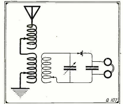
Method of Connecting 8,500 Meter Coupler.
