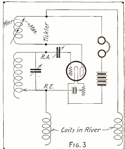
The Ordinary Tickler Circuit With the Coils Shunted Across the Phones and "B" Battery.
