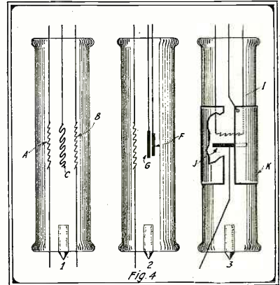
The Tubes After the Elements Have Been Inserted.
