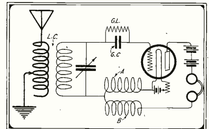
Using the Variometer in the Ordinary Regenerative Circuit.
