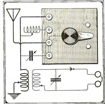
A Simple Method of Constructing a Wavelength Switch.
