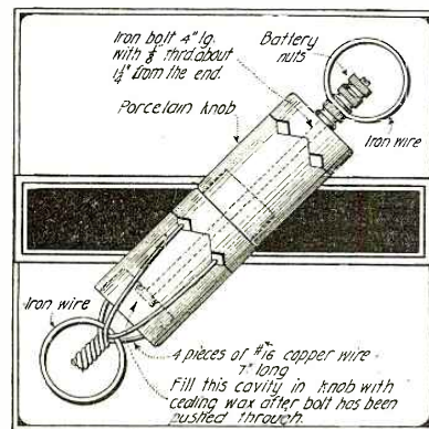
A Simple Insulator for a Receiving Antenna.
