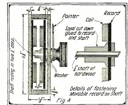
Showing the Manner of Assembling the Variometer.
