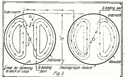
Fig. 3 Showing How the Coils Are Mounted on the Records.
