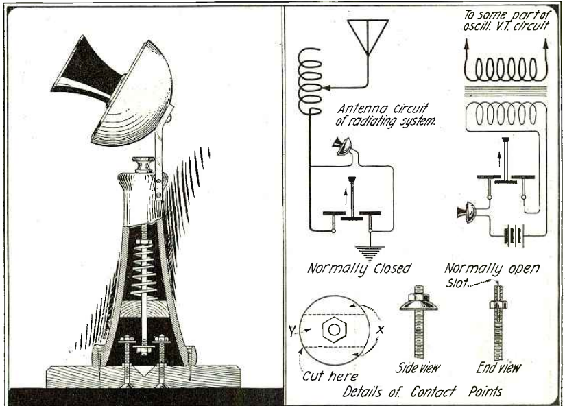
This Is a Clever Stunt for Mounting the Transmitter and Button Control. Note How the Device Is Used in the Circuit.
