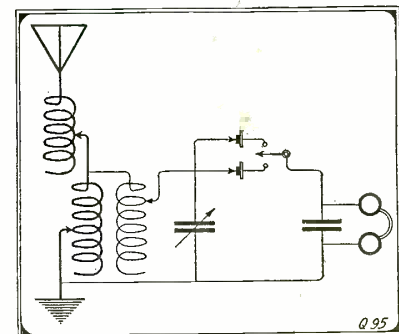
Hook-Up for Using Two Detectors.
