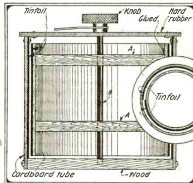
A Variable Condenser Easily Constructed.
