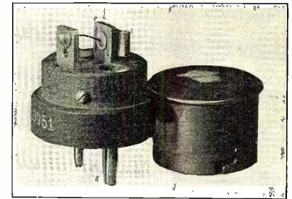
This is a Unit Crystal Detector Which is Very Rugged, Yet Efficient.
