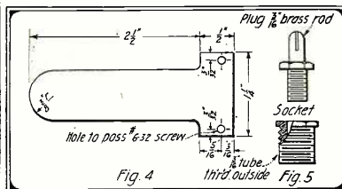
Details of the Coil Fastening Arrangement.
