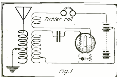
The Ordinary Tickler Circuit for Receiving Undamp Signals.
