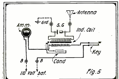
Here is the Circuit of the French Spark Transmitter.
