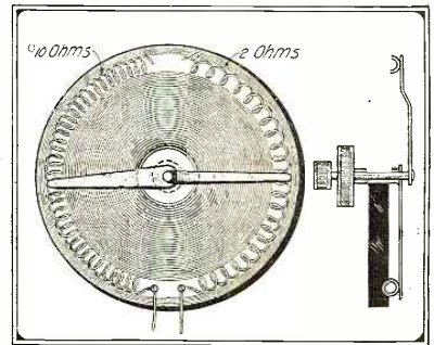
Type of Rheostat Necessary for a Tube Requiring Critical Adjustment.
