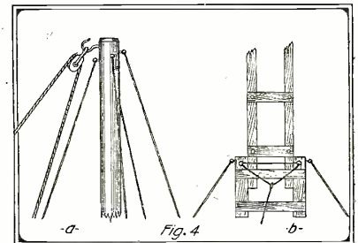
Method of Guying the Mast.
