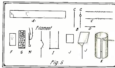
Details of the Element Construction.
