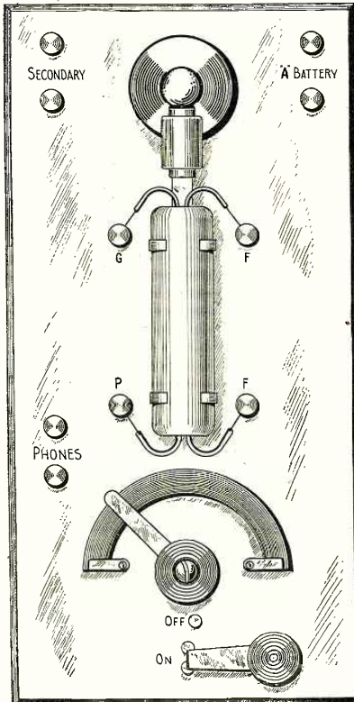
Front View of the Audion Cabinet.
