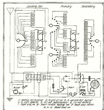
Wiring Diagram of the Prize Set.
