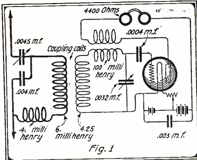
Tickler Circuit Used In Conducting these Experiments.
