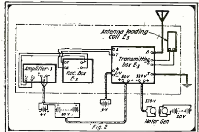
Method of Connecting the Transmitter, Receiver and Amplifier Sets.
