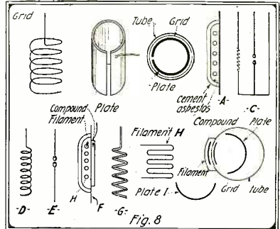
Additional Details of the Element Construction.
