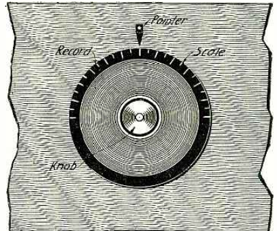
A Ten-Cent Phonograph Record Makes Up a Neat and Inexpensive Dial.
