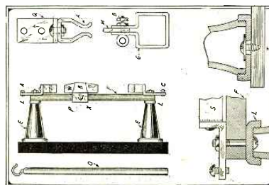
Constructional Details of the Antenna Switch.
