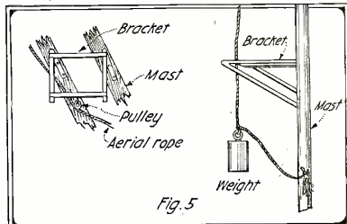
This Prevents the Antenna From Sagging.
