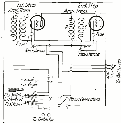
Wiring Diagram of the Amplifier.
