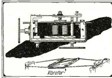
Constructional Details of the Buzzer.
