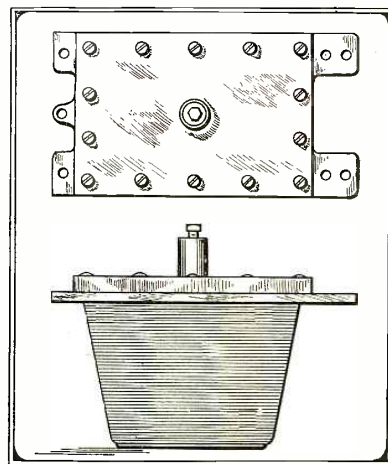
Drawing of the Condenser Showing the Method of Fastening Top.
