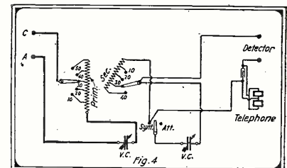
Showing Connections of the French Aero-Plane Set.
