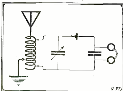
Simple Three-Slide Tuner Hook-Up.
