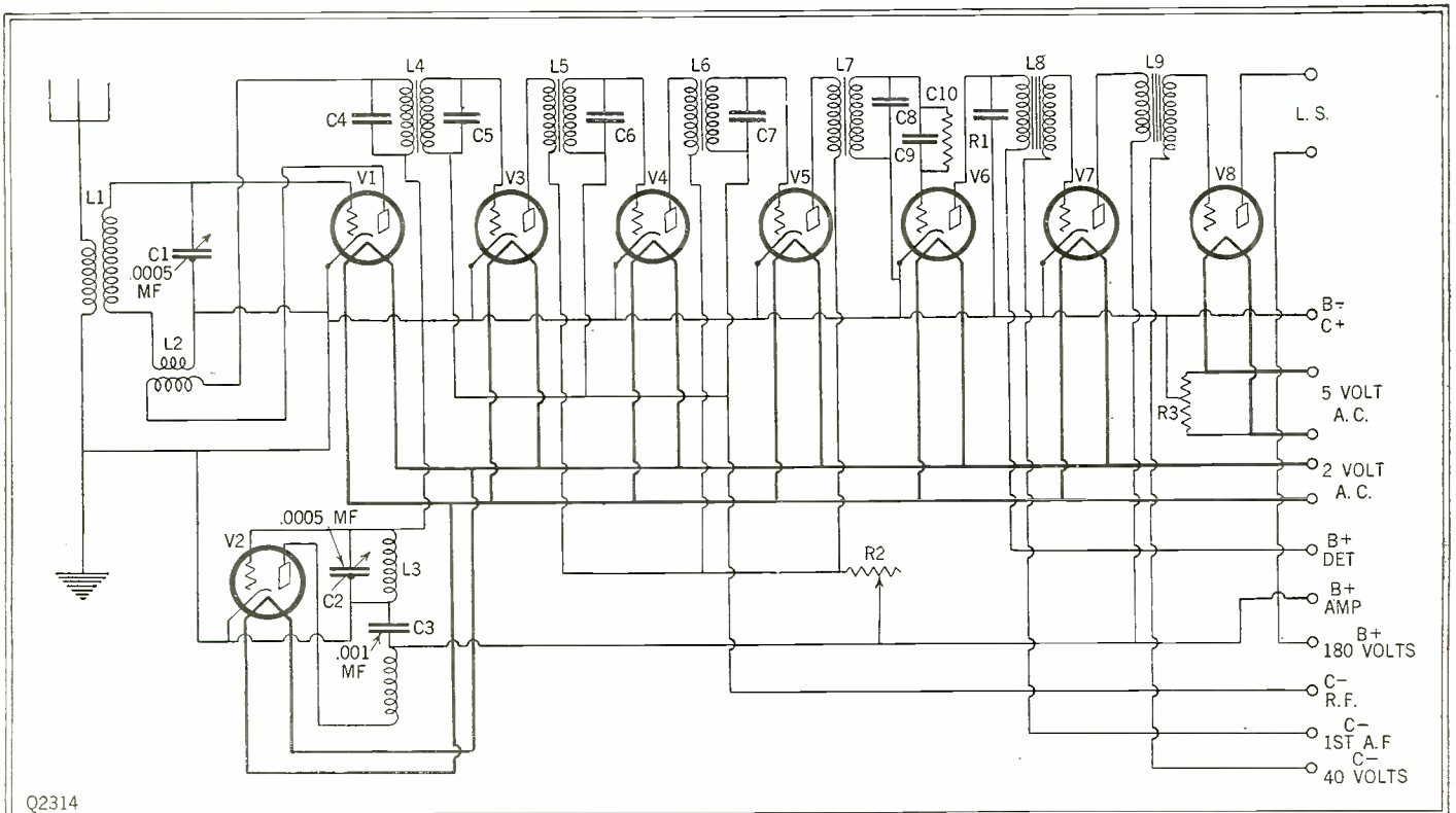
The Ultradyné L2 schematic circuit is shown above with the necessary changes to adapt it to the use of A.C. (227-type) tubes. Values
