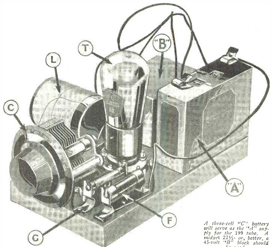
Below: A complete oscillator assembled on a board only; 8 inches long and 4 inches wide. "A" and "B," batteries; L, 75 turns No. 24 wire on 2 1/2-inch tube, tapped in center (See Fig. 1); C, .0005-mf. condenser; T, should be 199-type tube; F, filament ballast, instead of rheostat; G, grid condenser and leak, optional.
