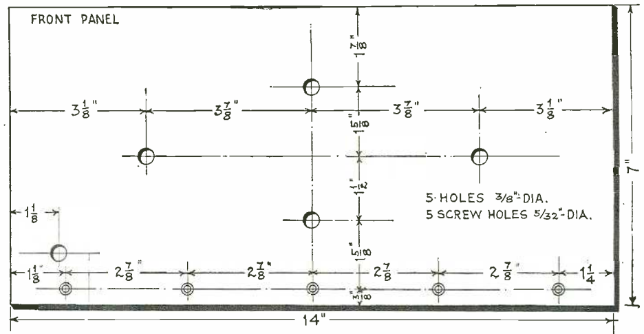
Fig. 5 Drilling diagram for the front panel of the Plugless receiver; below, that for the sub-panel for coils.
