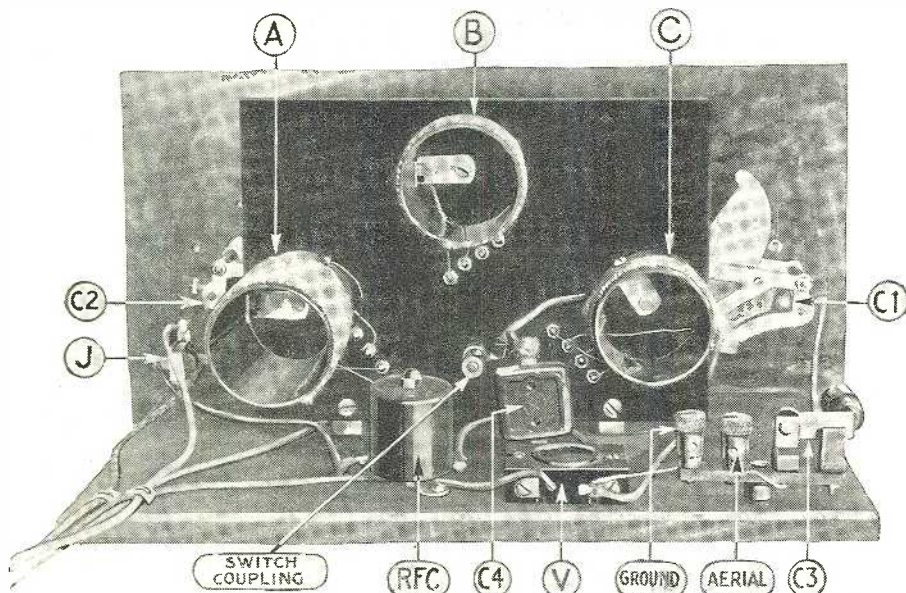
The black vertical panel in the center of this rear view of the Plugless Receiver carries the three coils, A, B, and C, which cover the three wavebands. The switch pivots on its coupling.
