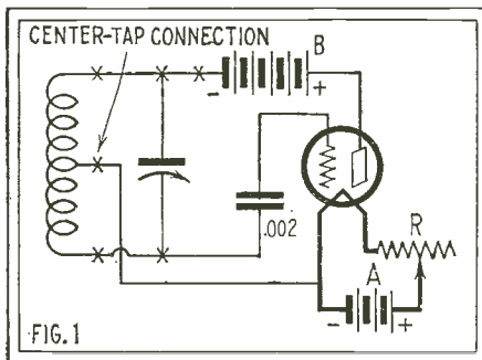
Schematic diagram of an easily-made oscillator. The grid condenser (.002) may be omitted. If it is used with a grid leak the oscillator will generate a modulated signal.
