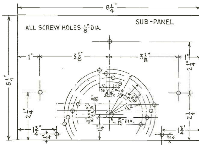
Fig. 6 A constructor designing his own might extend the number of coils beyond the three used here.
