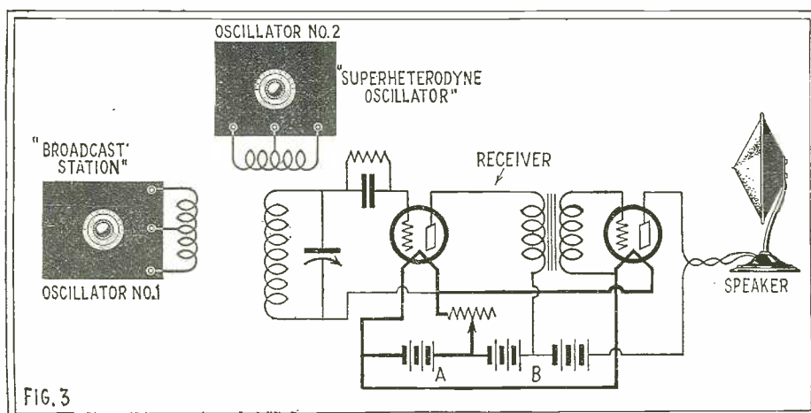
The effect of "heterodyning," or the generation of a third current by the mingling of two currents of different frequency, can be observed with this arrangement. It corresponds to a superheterodyne circuit.
