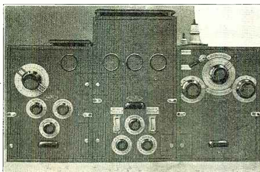
Fig. 1. Here is a 2-K.W. C.W. Transmitter Equipt With Four 500-Watt Tubes. The Three Cabinets From Left to Right Contain the Rectifier, the Power Tubes and the Wave-Length Control.
