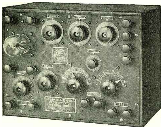
A Compact Receiving Set for the Reception of Undamp Waves Only Embodying Electro-Magnetic Field Control.
