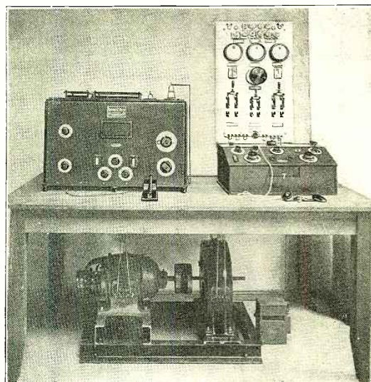
Fig. 2. A Complete 1 K.W. Undampd Wave Set. On the Right is the Receiver and Under the Table the H.T. D.C. Generator.
