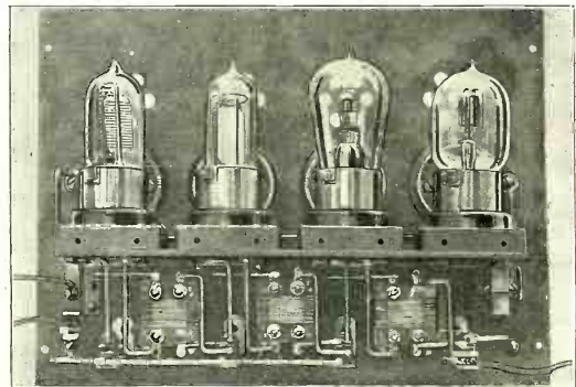
Back View of the Panel Supporting All the Parts. Note the Compactness and Neatness of the Work.
