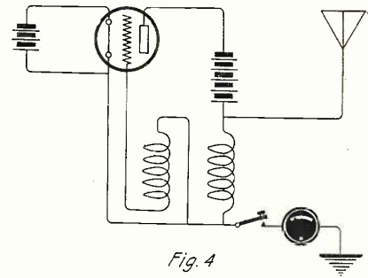
Fig. 4 The Elementary Circuit of a C.W. Transmitter.
