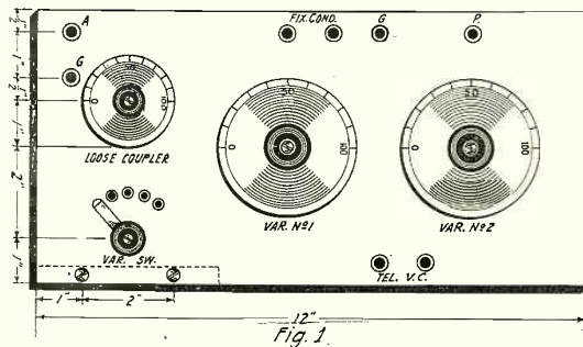
Front View of the Short Wave Receiver. The Arrangement of the Dials and Switch Gives to This Apparatus a Very Commercial-Like Appearance.
