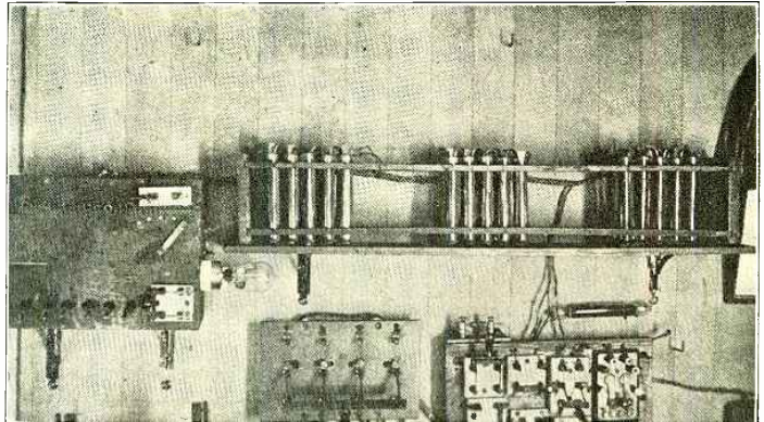
Photograph of the switchboard and storage "B" Battery built by Mr. Harry Boyce, Jr. This may easily be duplicated by the amateur to supply the H.T. to the V.T.'s of either the transmitter or receiver. It is a very economical way to obtain D.C. and get rid of the dry batteries.
