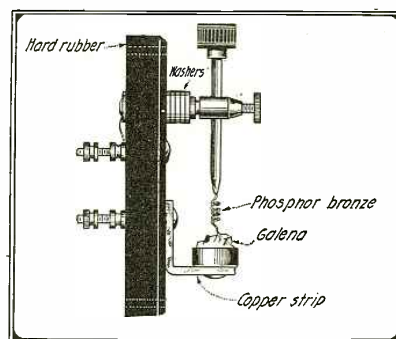
A Phosphor Bronze Wire is Soldered to Brass Rod for Contact with Crystal
