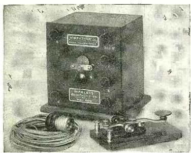
The VIBRATONE JR. is a high voltage buzzer type radio transmitting set which operates directly on any 110 volt circuit, either A.C. or D.C. It requires no spark gap, condenser, etc., but is complete, ready to operate, as shown. It fully complies with all Federal regulations, in regard to emitting a sharp-wave. Operates all day for less than 2 cents. Equipped with Mesco transmitting key. Guaranteed for one year, built to last indefinitely. Normal range up to five miles, but the above cards show what it has done.
