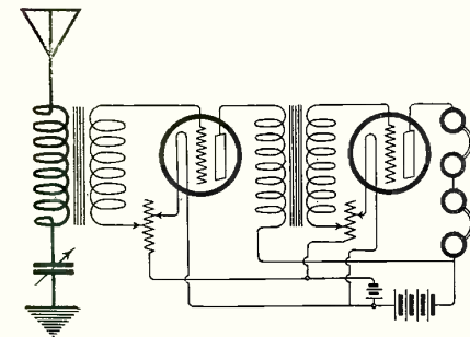
Fig. 2. Connecting the Aerial and Ground to the Primary of the Amplifying Transformer, Long Wave Stations Are Easily Picked Up.
