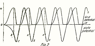
Fig. 2 Curves Showing the Variations of the Grid and Plate Potential in a V.T. Oscillator.
