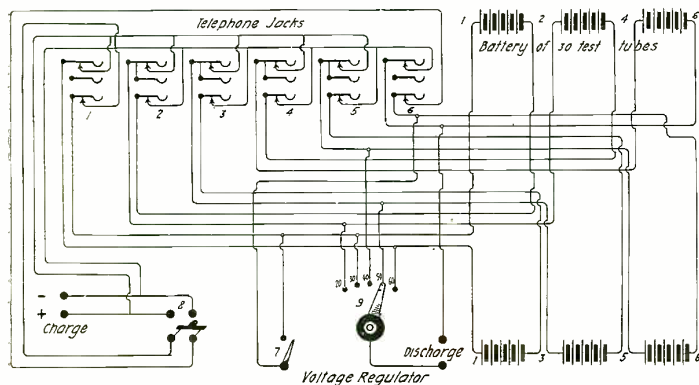
Complete diagram of the variable "B" battery made of test tubes. Note the voltage regulator and the clever system of jacks.
