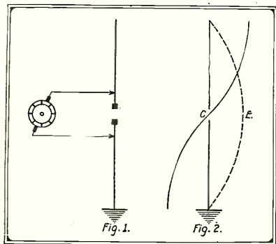
Fig. 1 Illustrates a Very Elementary Circuit of a Direct-Current Generator Supplying Current to an Arc, While Fig. 2 Shows a Vertical Oscillator with a Spark Gap in the Circuit.
