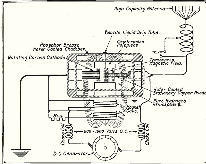
Elementary Circuit Diagram of a Continuous Wave Transmitter Employing the Arc. During Transmission the Arc is Constantly Radiating, and Telegraphing is Accomplish by Means of a Key Which Rapidly Changes the Emitted Wavelength.
