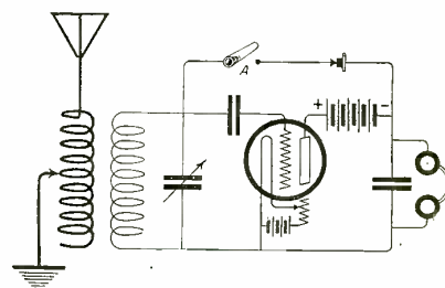
A Simple Way to Change From Audion to Crystal Detector; Only One Switch is Necessary.
