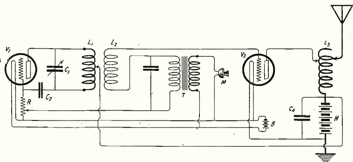
Fig. 2. In this circuit using only two tubes the output of the amplifier is controlled microphonically and gives a clear modulation. An experimental set of this type may easily be built by the amateur.
