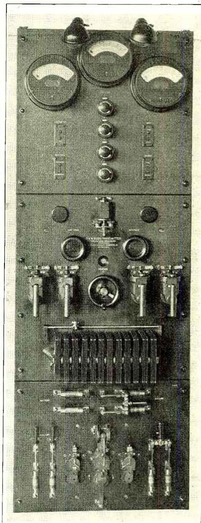
Front View of the New 2-K.W. Set. Note the New Quenched Gap Built in Sections and the General Arrangement of the Panel.
