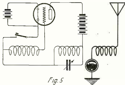
Fig. 5 Practical Circuit of an Undamped Wave Transmitter. The Aerial is Coupled to the Oscillating Circuit.
