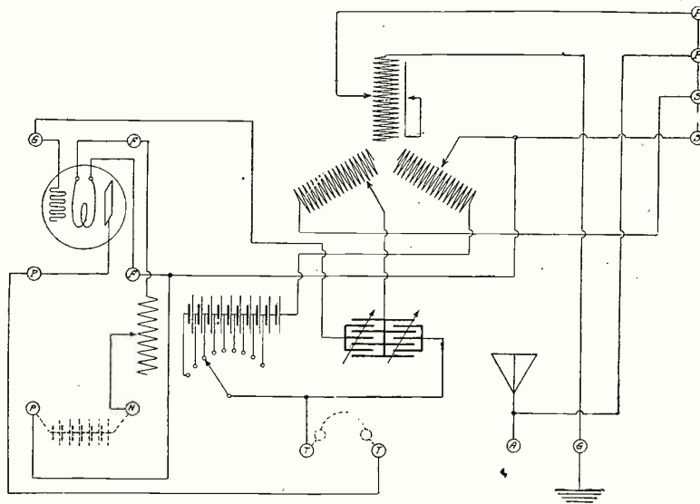
Fig. 1. General Layout and Wing Diagram of the True Undamp Wave Receptor Described by Mr. Mignon.
