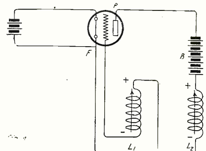
Fig. 4 The Typical Circuit for Producing High Frequency Undamped Oscillations With a V.T.
