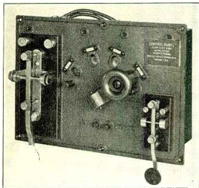
The Upper Photograph is a Rear View of the Transmitter, While the Lower One Shows the Control Panel From Which All Operations in the Set are Effected.
