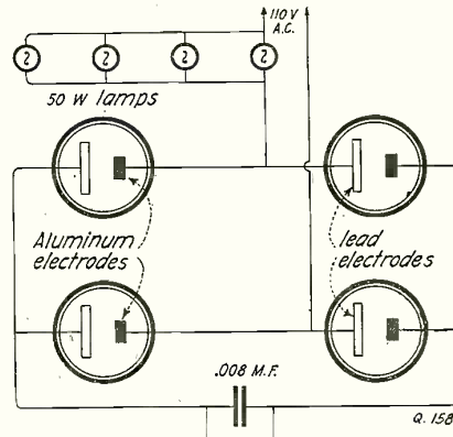
With This Electrolytic Rectifier D.C. is Obtained for Charging Batteries or Supplying the Plate of a V.T. Detector.
