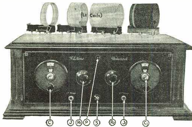
On the lid of the receiver are shown the L1 coils, (the secondary and tickler). The symbols indicating the different controls correspond to those of the other illustrations.
