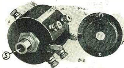
View of the amplifier control switch. The loud-speaker plug fits directly in the hollow shaft, S, and makes the proper connections to springs within the switch case.
