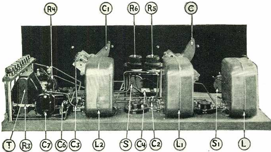
A rear view of the completed set. R5 and R6 are the rheostats controlling the detector tube and the three audio-frequency amplifier tubes. After being once correctly adjusted they need not be touched again. R3 and C7 are the grid leak and grid condenser, respectively. The detector tube socket is directly behind C7. C4 is a radio-frequency by-pass condenser.
