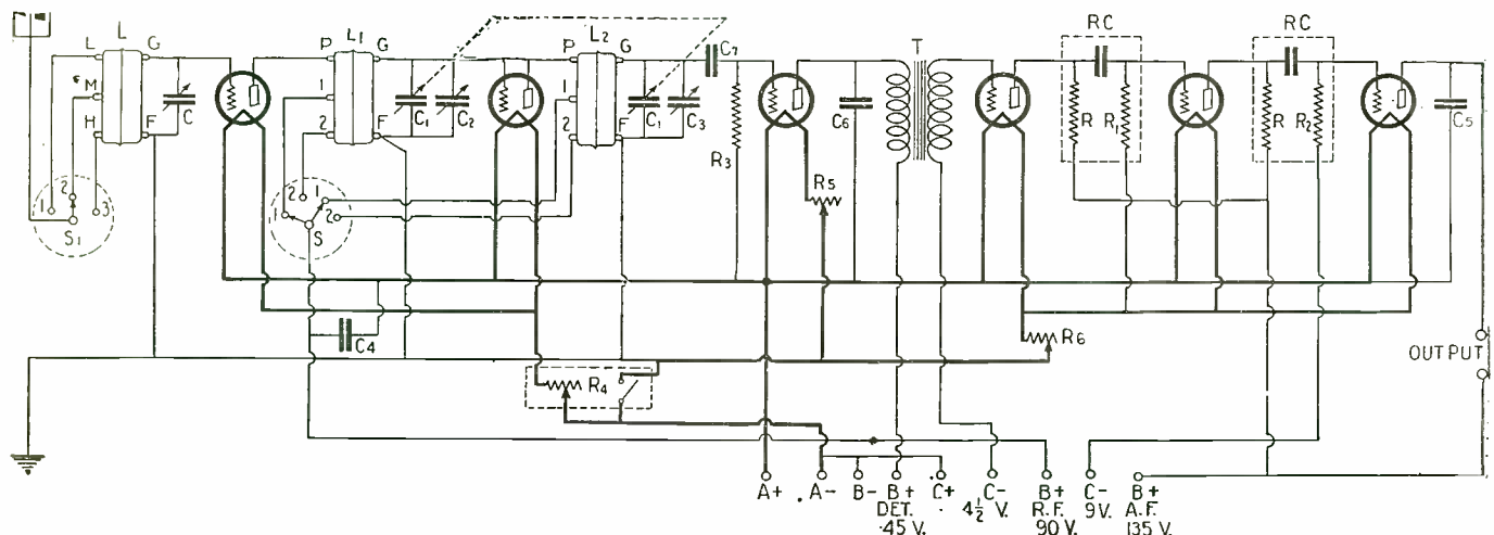
The complete schematic wiring diagram of the Quadraformer VI. Receiver. Note that the switch S controls both the R.F. transformers at once. Switch S1 controls the aerial coupler. The combination rheostat and filament switch is shown at R4.
