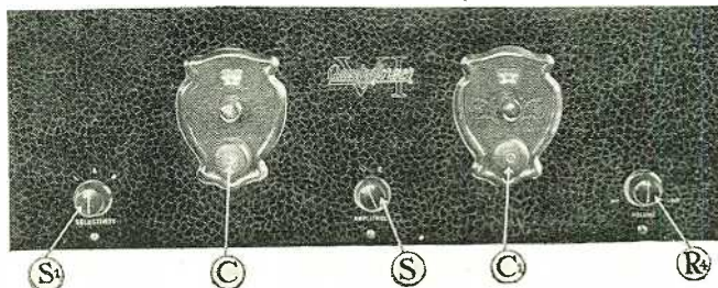
A panel view of the Quadraformer receiver. C and C1 are the main tuning controls. S and S1 are the selectivity controls, which can be adjusted to suit local and distance reception requirements. R4 is the combined rheostat (for the two R.F. tubes) and filament switch. When the knob has been rotated fully to the left the whole set is turned off.
