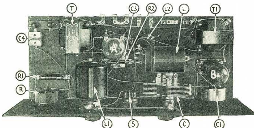
A top view of the DX-2 receiver. C3 and R2 are the grid condenser and grid leak respectively; S is the filament switch and C1 the variable condenser employed for controlling regeneration.
