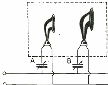
Better reproduction can be had by using two loud speakers, connected in parallel, and tuned by high-capacity condensers.
