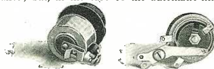
Fig. 8. Left: A variable resistance of the graphite-powder-compression type which has a range of resistance from zero to 5 million ohms. Due to these wide limits and large current carrying capacity, it can be employed in almost any place where a fixed or variable resistance is called for.
