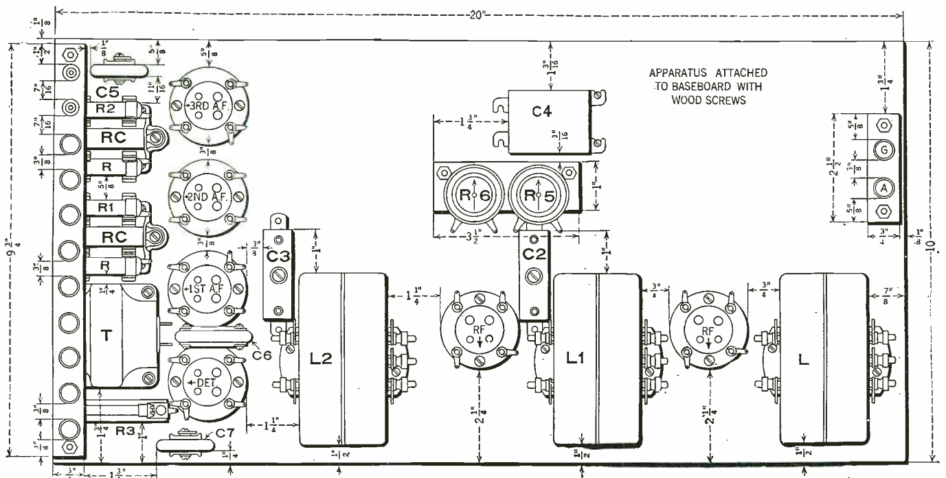
Layout of the apparatus on the wooden baseboard. The correct spacing between parts is given in each case and it is suggested that this be followed; though, if desirable, the layout can be altered slightly without consequent ill effects in operation.
