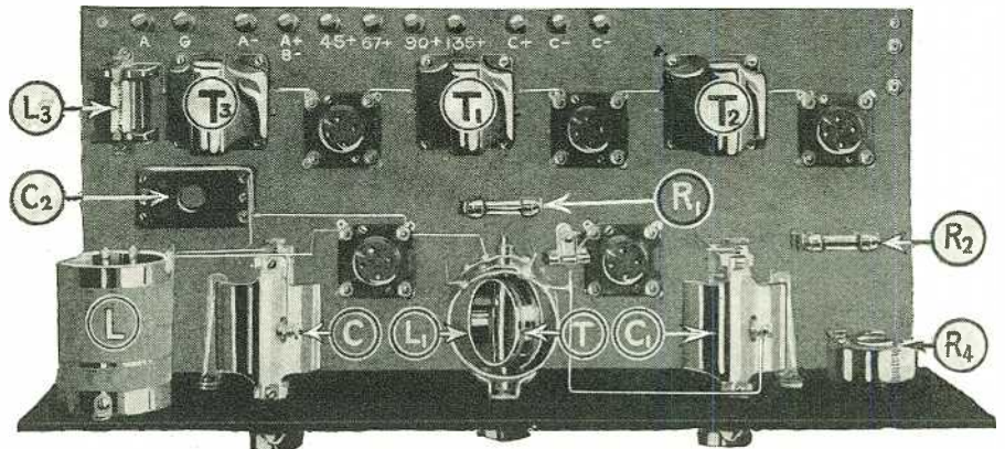
(Q. 2201). Another interior view of the Samson T.C. receiver, showing clearly the layout of the parts, designated in the other illustrations and list of apparatus.
