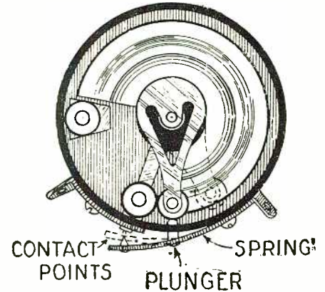
Back view of the resistor-switch, showing the arrangement of the flexible spring plunger, rotating arm and contact points. Illustrations courtesy Central Radio Laboratories.
