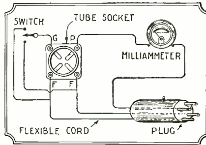
Hook-up of the tube-checker, showing how the grid is connected to either side of the filament to obtain positive or negative bias. Note that the grid tip of the plug is dead.
