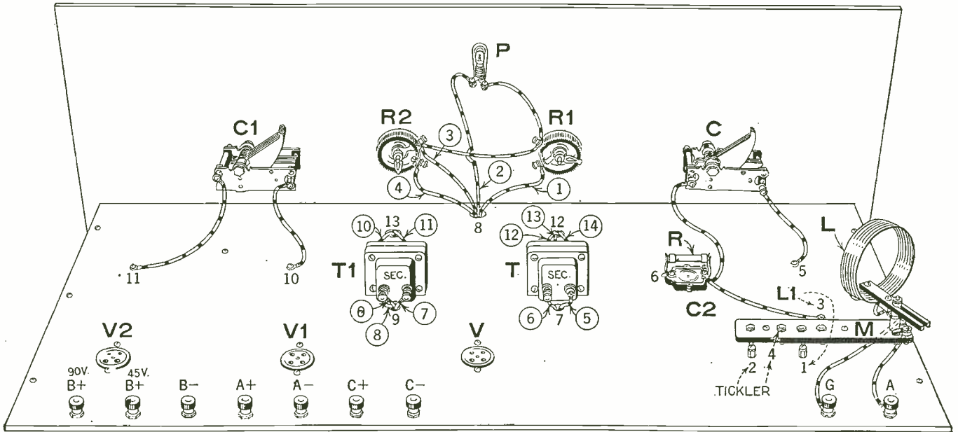
The wiring on the upper side of the sub-panel. The numbers in circles designate the connecting wires and the numbers not enclosed indicate holes through the sub-panel, through which the connecting wires pass.
