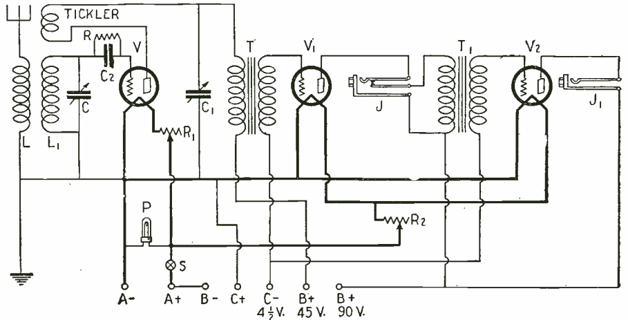
The schematic wiring diagram of the Pilotone three-tube regenerative receiver. The symbols are the same as those on the other illustrations designating the parts.
