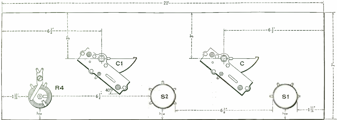
Constructional panel layout of apparatus, including all the necessary dimensions and spacing between parts. It should be kept in mind that C1 is a tandem variable condenser and a clear space must be provided on the sub-base over which it extends.
