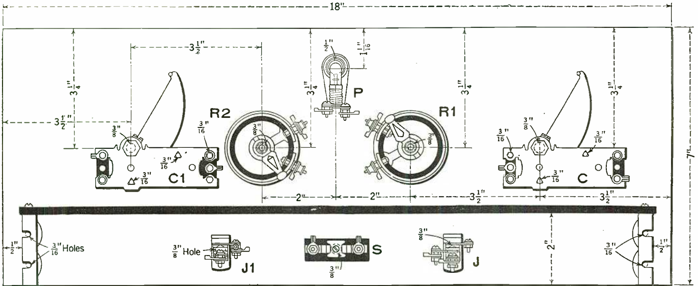
The layout of the panel, showing the size of the holes which are drilled in the panel, together with their locations.
