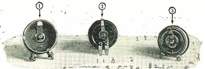
Fig. 2. Three midget-type rheostats which are particularly useful in small compact sets. They have all the advantages of the larger types. (Courtesy of: 1, Leslie F. Miter Co.; 2, Amsco Products, Inc.; 3, Carter Radio Co.)
