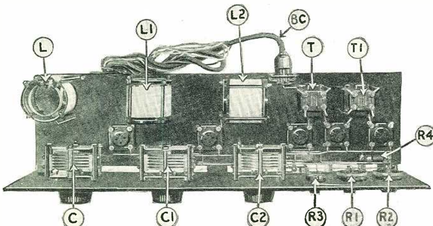
A top view of the Aero-Dyne receiver. The parts here carry the same designations as in the other illustrations and the list of apparatus, given elsewhere.
