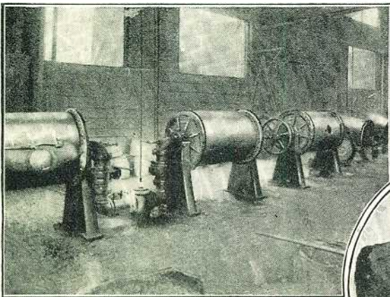
One of the batteries of electric furnaces, each capable of maintaining a temperature of 5200 degrees Fahrenheit, used in the melting of silica sand, and the amalgamation with it of reducing materials and several alloys used in manufacturing silite, the new metallic glass-like rectifying element, which takes the place of precious metals by its resistance to acid.
