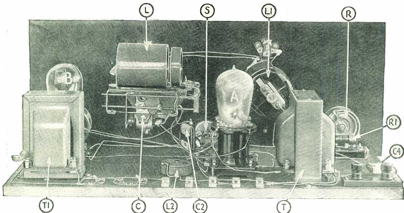
A rear view of the DX-2 Multivalve receiver. A is the new vacuum tube, which is actually three tubes in one, with a single 5-volt ¼-ampere filament. B is the semi-power amplifier tube. R is the rheostat governing the filament current supplied to tube A, and R1 is an automatic filament control, used in conjunction with tube B. L1 is a variometer, which tunes the antenna circuit; and L-C the auto-coupler, which comprises a variable condenser and an automatically-coupled R.F. transformer. C2 is a radio-frequency by-pass condenser, and C4 the fixed antenna series condenser. L2 is a radio-frequency choke. T and T1 are the AF transformers.
