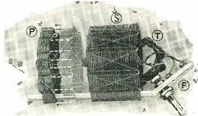
P is the primary, S the secondary, T the tickler and F the frame of this three-circuit tuner. The primary and secondary may be moved back and forth, as indicated by the dotted lines near the primary, so that different degrees of coupling may be employed for different conditions of reception.
