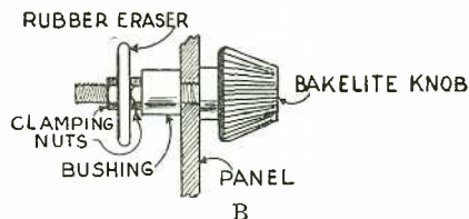
The vernier knob and shaft, to which is attached the rubber eraser.
