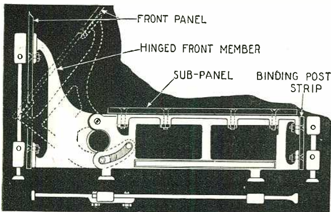
The dotted lines show how the front panel of a receiver may be fixed at an angle by means of the adjustable bracket. The positions of the sub-panel and the binding-post strip are also clearly indicated.
