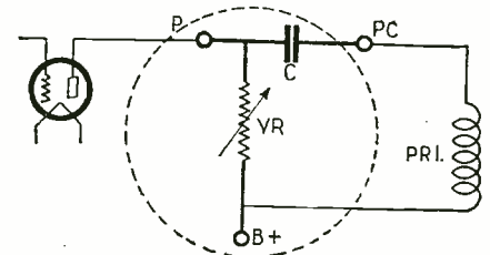
This diagram shows how the phase-shifting instrument, consisting of the fixed condenser, C, and the variable resistance, VR, is connected in the plate circuit of an R.F. amplifier stage. The posts marked P, PC, and B+ represent its three external connections.
