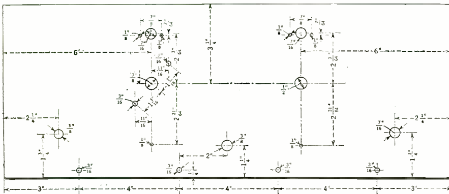
Layout of drilling for the panel of the DX-2 receiver.
