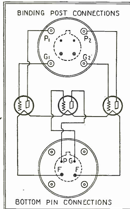
FIG. 1 Details of the three-in-one "Multi-valve" tube, showing its internal construction and, at the right, the connections to the tube-base prongs and to the special binding posts. Illustration courtesy of Cleartron Vacuum Tube Co.
