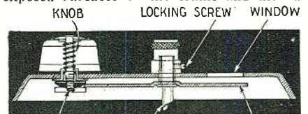
Cross-section view of the vernier dial, showing the internal construction.
