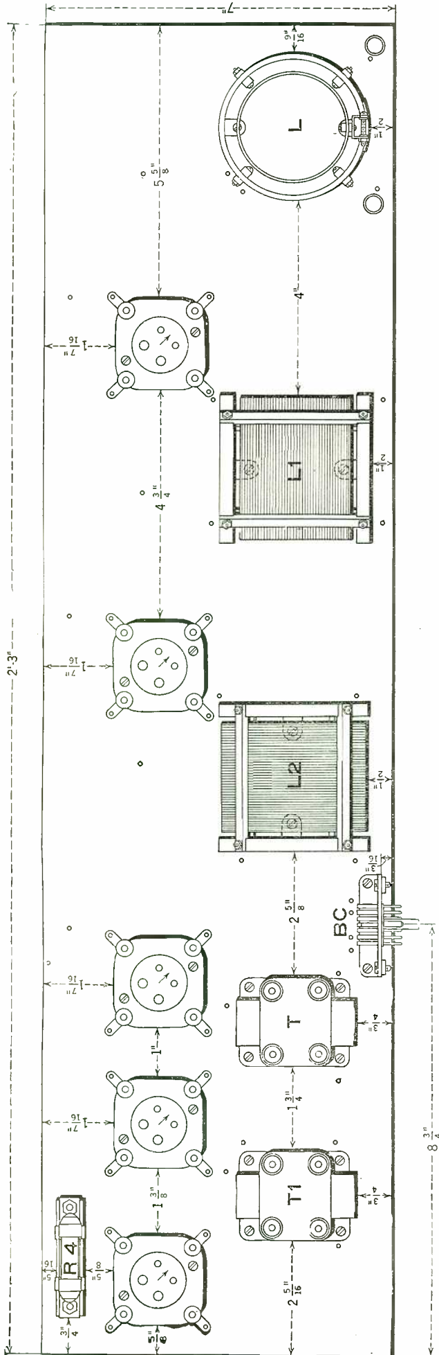
Above: Layout of apparatus on the sub-base or sub-panel. Note the small holes near some of the apparatus. These are provided for passing the wires through to the underside of the sub-base. In mounting the sockets be sure to have the arrows pointing in the same direction as indicated. The primary terminals of both transformers, T and T1, should face to the right, or towards the coil, L2.
