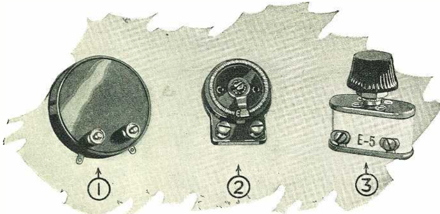
Fig. 7. Three variable high resistances with high current-carrying capacity. These are employed primarily as voltage controls, in both D.C. and A.C. "B" battery eliminators, but have many other uses in connection with a radio set. They are similar in design to those shown in Fig. 6, but have large-surface resistance elements.
