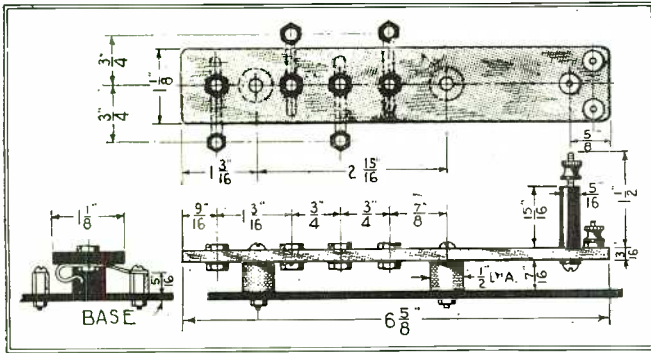
The layout of the panel, showing the size of the holes which are drilled in the panel, together with their locations.
