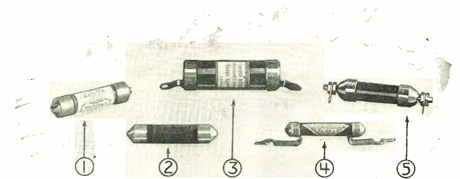
Fig. 10. A group of heavy-duty resistors which are employed principally as voltage adjustors in D.C. and A.C. "B" eliminators, but are useful also as current-by-pass and current-shunt units. Nos. 1 and 2 employ a carbon compound as the resistance; 3 is a lavite resistance unit. The resistance shown at 4 is made of carborundum; No. 5 is formed of a graphite compound which is fused into glass.
