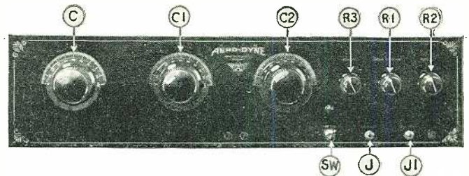
A panel view of the Aero-Dyne receiver. C, C1, and C2 are the tuning controls; R3 is the oscillation control; SW the filament switch; and J and J1 are the two output jacks of the A.F. amplifier.
