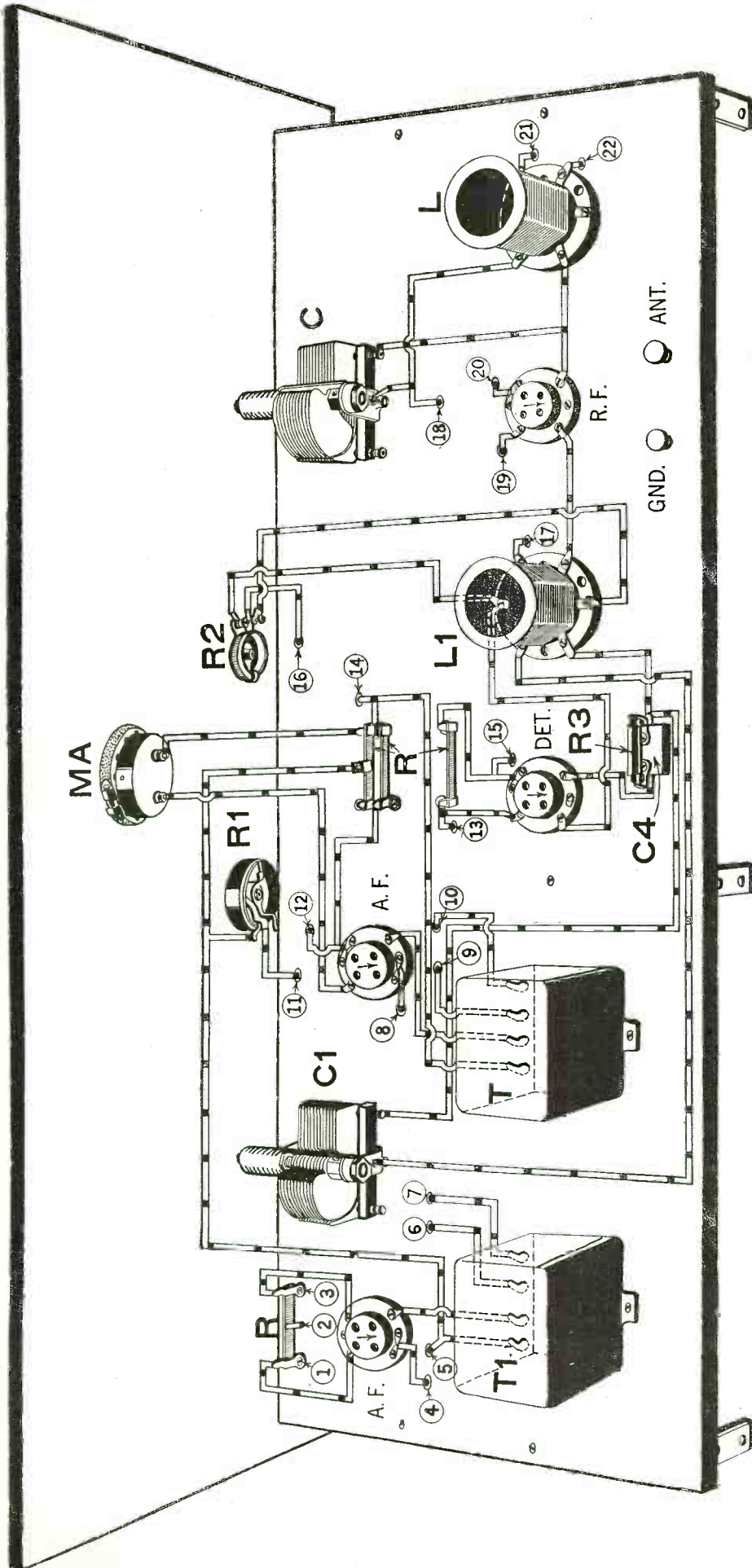
Left: Perspective layout and wiring of the receiver unit of the RADIO NEWS Batteryless set. Those wires which pass through holes in the sub-base connect to apparatus underneath. The continuation of the wiring on the under side of the sub-base is shown above. All of the wires that pass through holes are numbered alike in both views.
