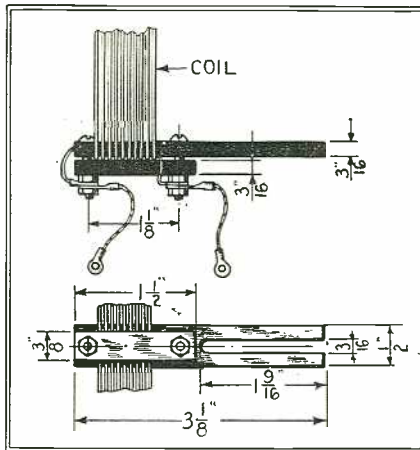
This is a detail drawing for constructing the antenna coil, L. This inductance is mounted on the bakelite post shown in the drawing of the mounting on page 975. The slot shown here, in the bottom view of this coil, is placed in the screw and clamped in position by the nut, as can be seen from the illustration below.
