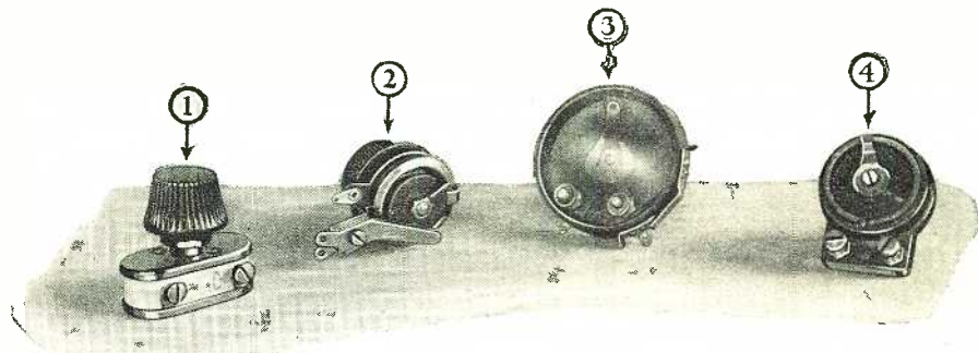
Fig. 6. A group of variable high resistances which can be employed as volume controls, regeneration controls, oscillation controls and in connection with resistance-coupled audio amplifiers. Number 1 is the carbon-disc-compression type. The rest are of the graphite-compound type, with frictionless contacts. Note that No. 2 has an automatic switch connected to it. This closes upon the turning of the control knob. No. 3 incorporates a similar device.
