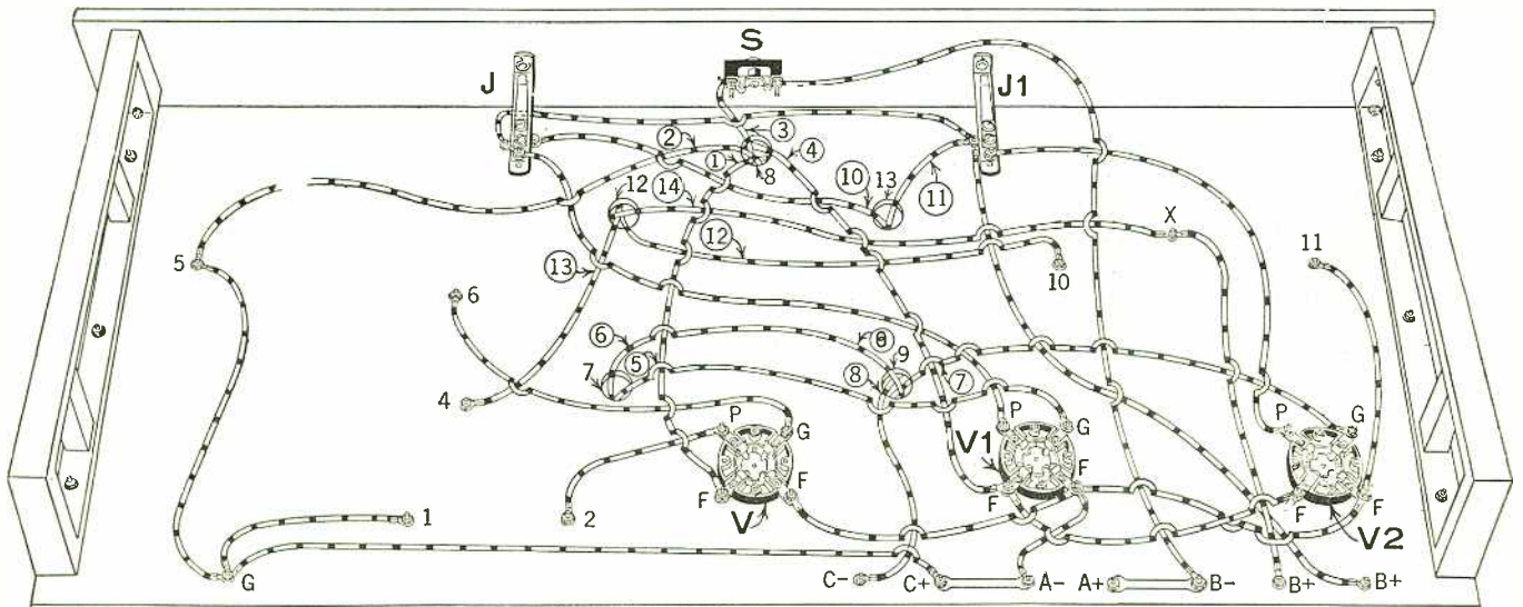
The wiring beneath the sub-panel. S, is the filament switch; J and J1 are the jacks. The wires here shown correspond in numbering to the wires shown in the drawing at the top of the page.
