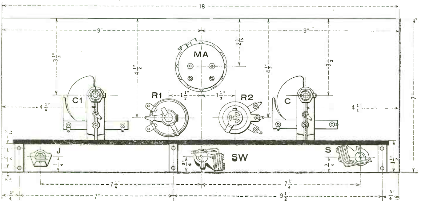
Below is shown the constructional layout of the panel for the receiver. All the necessary dimensions are given. The constructional layouts for both sub-bases, as well as the drilling layouts, are given on the opposite page. In all the illustrations and sketches the apparatus is similarly marked.
