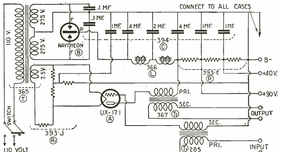
The schematic wiring diagram of the combined "B" battery eliminator and power amplifier. The parts carry the same lettering as in the other illustrations.
