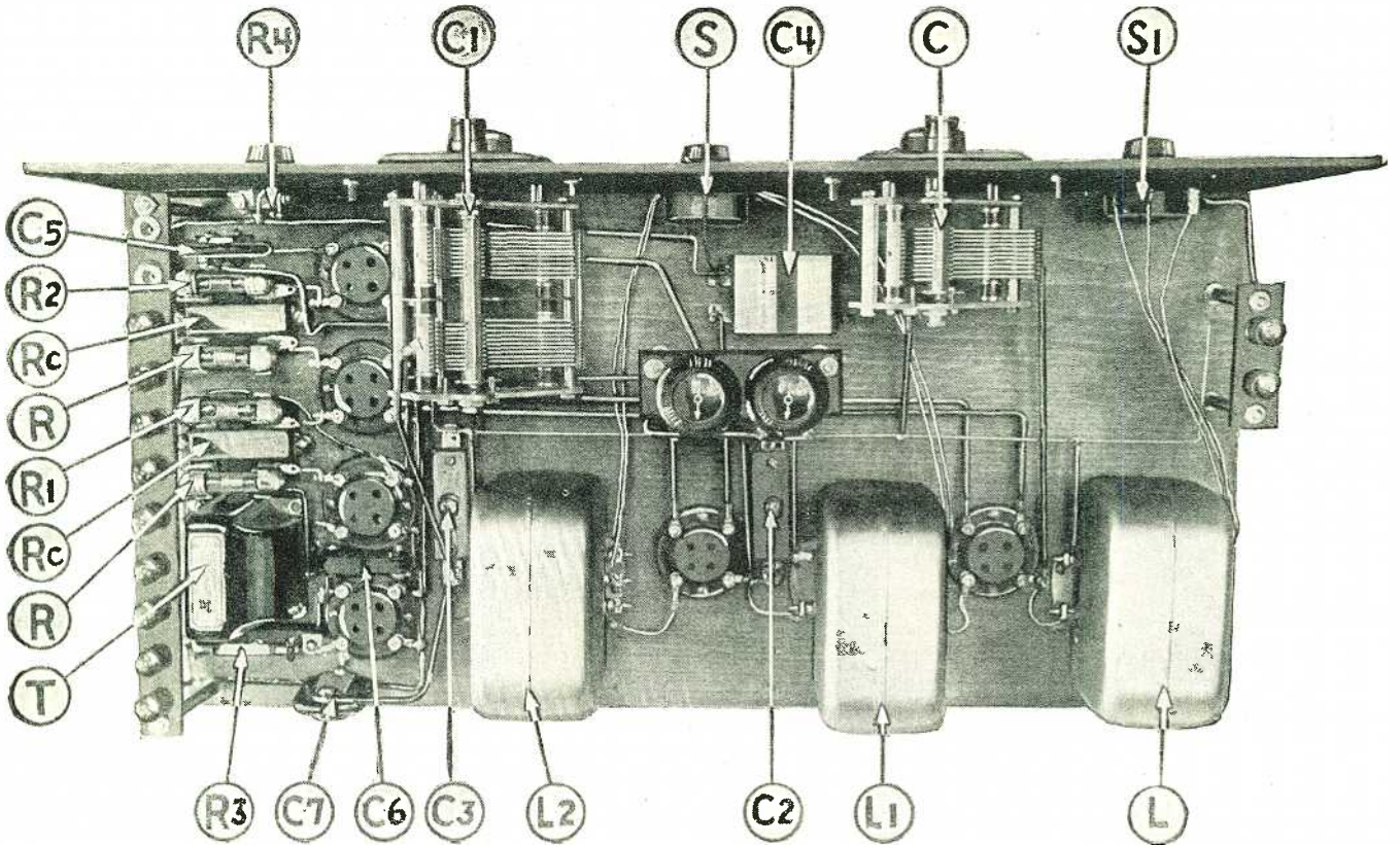
A top view of the Quadraformer VI Receiver. L, L1 and L2 are the shielded quadraformers, details of which are given in the sketch on page 987. S and S1 are the special switches which control the selectivity and, partially, the sensitivity of the set. C2 and C3 are adjustable condensers of the neutralizing type, which are employed to make up for any discrepancy in capacity between the two tandem condensers, and thus to equalize the dial readings. After they are once adjusted they need not be touched again. It will be noted that the audio-frequency amplifier comprises one transformer-coupled and two resistance-coupled stages; a very excellent combination which provides plenty of volume and quality reproduction. T is the A.F. transformer and RC are resistor couplers.
