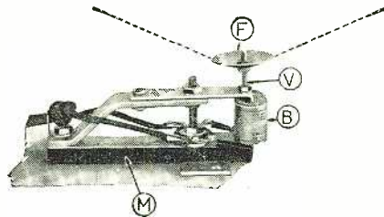
General view of the loud-speaker unit. M is the permanent magnet, B the bobbin, V the vibrating armature and driving screw, F the small metal cone for holding the large paper cone in place. The position of the paper cone is indicated by the dotted lines.
