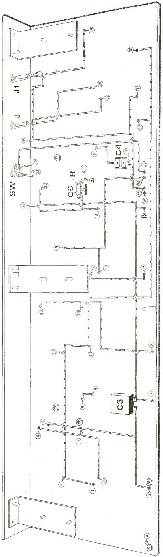
A perspective layout and wiring diagram of the Aero-Dvne receiver. The only portion of the wiring that might present some difficulty is that in the vicinity of the variable resistances, R3, where the leads pass down between the panel and the sub-base. However, if the lower drawing is consulted, the wires can be traced through the numbers in circles which are identical, for each lead, above and below the sub-base.
