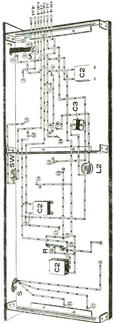
Left: Perspective layout and wiring of the receiver unit of the RADIO NEWS Batteryless set. Those wires which pass through holes in the sub-base connect to apparatus underneath. The continuation of the wiring on the under side of the sub-base is shown above. All of the wires that pass through holes are numbered alike in both views.
