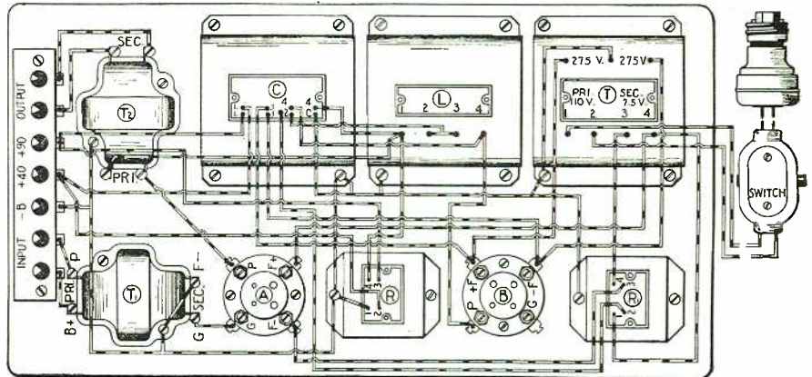
The layout of apparatus and wiring diagram of the complete "B" eliminator and power amplifier. The lettering on the parts corresponds to that on the parts in the illustration below.
