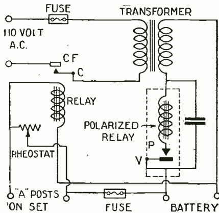
Hook-up of the charger, showing the general arrangement of the A.C. and D.C. circuits.
