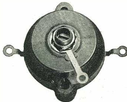
The phase-shifting device in assembled form. Adjustment of the resistance is obtained by means of the center screw, the head of which is visible in the above illustration.
