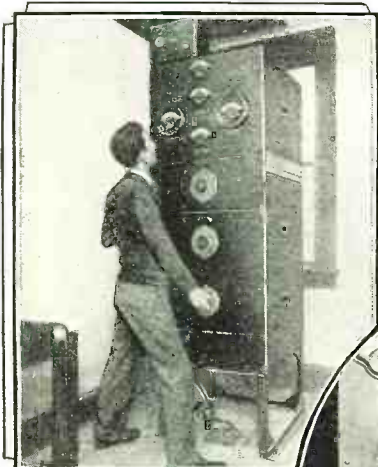
One of WRNY's operators is shown making a preliminary adjustment upon the transmitter. The wavelength of this is varied by the condenser and variable capacitor controls shown.
