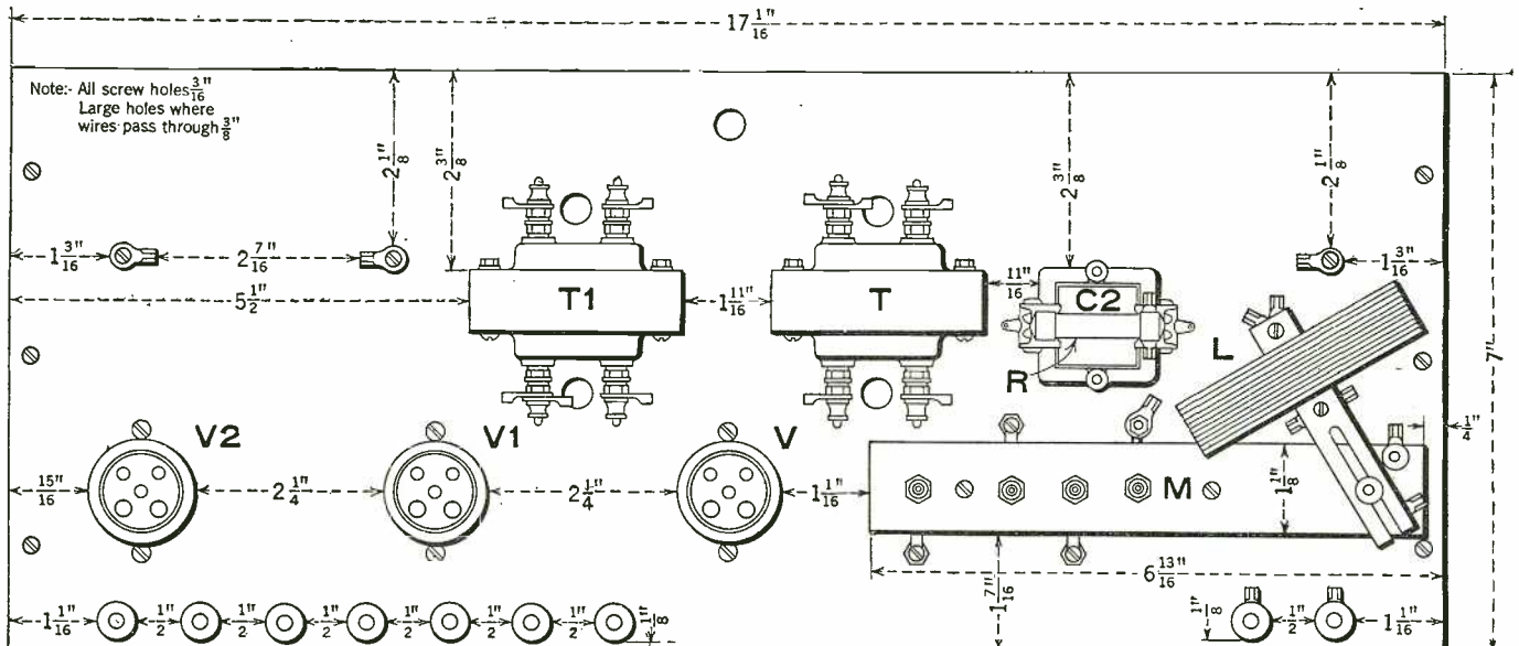
The arrangement of the apparatus on the sub-panel. The holes in the sub-panel can be located by placing the parts and then center-punching the centers for drilling.
