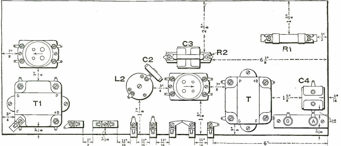
Layout of the apparatus on the base board and all the necessary dimensions. Take note of the fact that the two tube sockets are mounted in opposite directions; that is, the arrow on one points to the left and on the other to the right.
