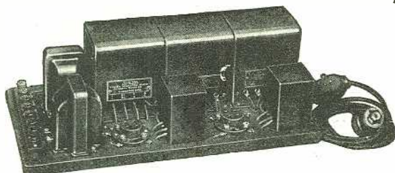
Showing GENERAL RADIO Type 395 Kit Fully Assembled
