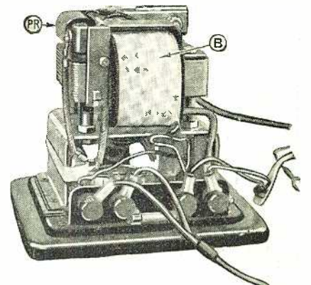
The charger with the case removed. The bobbin, B, holds the transformer windings. PR is the polarized relay. The primary circuit relay is hidden beneath the bobbin and is not visible in this view.
