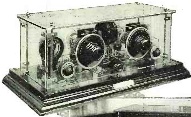
At the left is shown a receiver which employs plug-in inductances. This type of set is very popular in Great Britain because of the wide range of broadcast wavelengths used throughout Europe.
