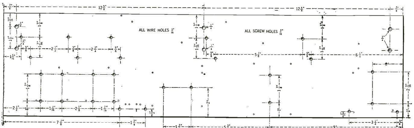
Drilling layout of the sub-base. The small holes indicated are for passing the connecting wires through the sub-base.
