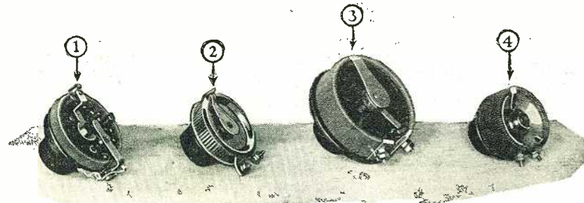
Fig. 3. A group of power rheostats designed to control the filament current to a number of tubes. They are similar to regular types of rheostats but are wound with much heavier wire. The rheostat marked 2 has resistance wire in the form of a ribbon. (Courtesy of: 1, Yaxley Mfg. Co.; 2, Central Radio Laboratories; 3, General Radio Co.; 4, Herbert H. Frost, Inc.)
