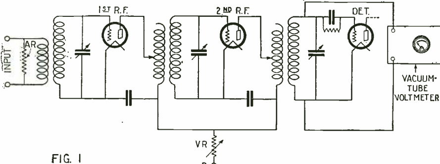
This experimental set-up, described in the text, was used to determine the best ratio of plate control to size of primary, in obtaining maximum amplification. The vacuum-tube voltmeter measures the output of the R.F. system (detector input), and the input to the receiver (antenna stage), is measured by the current-resistance-attenuation method.
