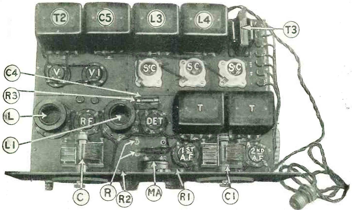
A top view of the RADIO NEWS Batteryless Receiver. There are actually two sub-bases, as will be seen on close inspection, that in front being the sub-base for the receiver, while the power unit is mounted at the rear. The power unit is comprised of a power transformer T2, a filter condenser bank C5, two filter chokes L3 and L4, a filament ("bell-ringing") transformer T3, two tube sockets V and VI and three lamp sockets SC. The receiver is composed of an antenna coil L, a radio-frequency transformer L1, two variable condensers C and C1, fixed filament-resistances R, a rheostat R1, a potentiometer R2, a milliammeter MA, a grid condenser and leak R3-C4, and two A.F. transformers T and T1.
