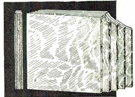
The five laminations of the new wood-panel are arranged so that their respective grains cross each other at angles, instead of running parallel. This arrangement offsets tendencies of the various layers to warp.
