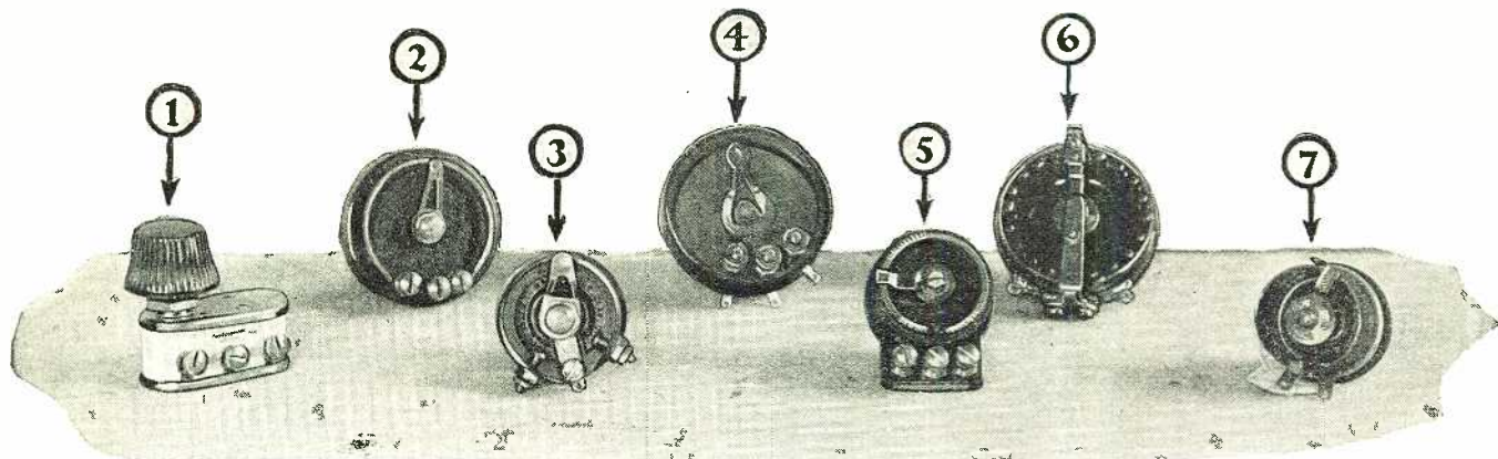
Fig. 5. A number of different types of potentiometers are shown in the above illustration. No. 1 is of the carbon-compression type; 2, 3, 6 and 7 are of the usual wire-wound type. Nos. 4 and 5 employ special graphite-treated elements and non-frictional contacts. These last two come in several resistance ranges, some being as high as 500,000 ohms, and can be employed for any number of purposes.
