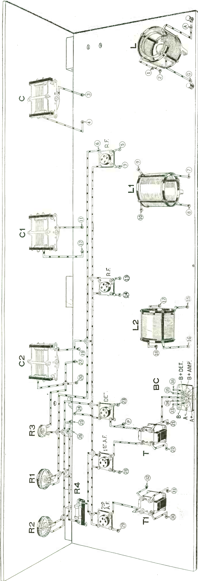
A perspective layout and wiring diagram of the Aero-Dvne receiver. The only portion of the wiring that might present some difficulty is that in the vicinity of the variable resistances, R3, where the leads pass down between the panel and the sub-base. However, if the lower drawing is consulted, the wires can be traced through the numbers in circles which are identical, for each lead, above and below the sub-base.
