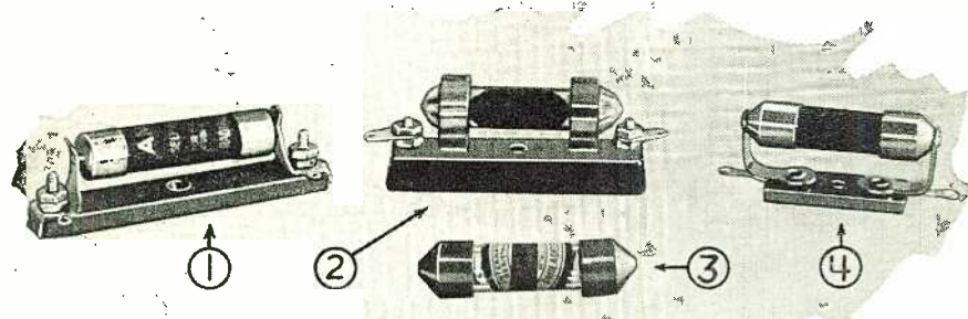
Fig. 4. These automatic filament controls can take the place of rheostats in almost any radio set. They control one or more tubes at a time and come in all standard resistance-ranges required for tube operation.
