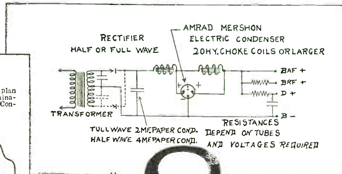
Circuit for building B eliminator using a Mershon Condenser as principle capacity.
