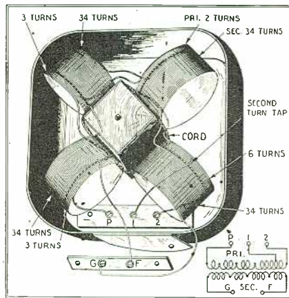
Constructional details of the "Quadraformer" coils. The four coils are made up by winding them on a cardboard tube, slipped off, tied to the wooden block and wired in series as shown. All coils are wound with No. 24 D.C.C. wire.
