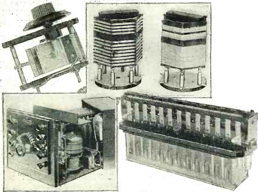
The variable condenser at the upper left is operated by a cam regulating the overlap of two plates. At the right are two types of plug-in inductances of a low-loss construction. Below, at left, an English battery eliminator; and at the right a "B" battery with switches changing the internal connection for charging purposes, as explained in the text.
