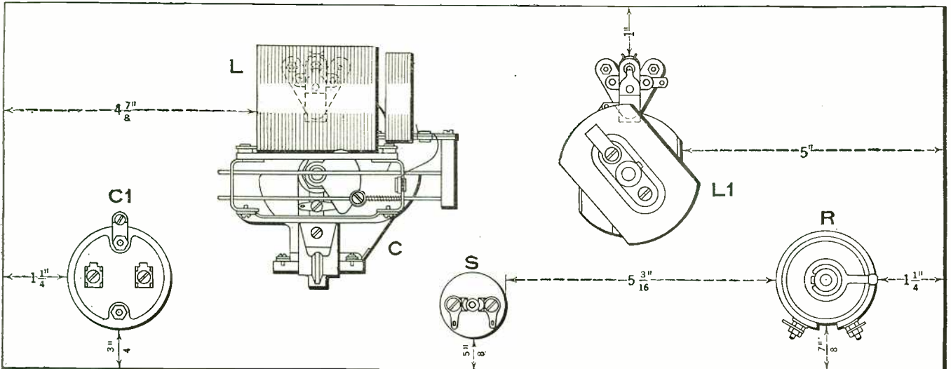
Panel layout of apparatus. There is a double bracket for mounting the variometer L1. The holes for this are shown in the lower sketch.
