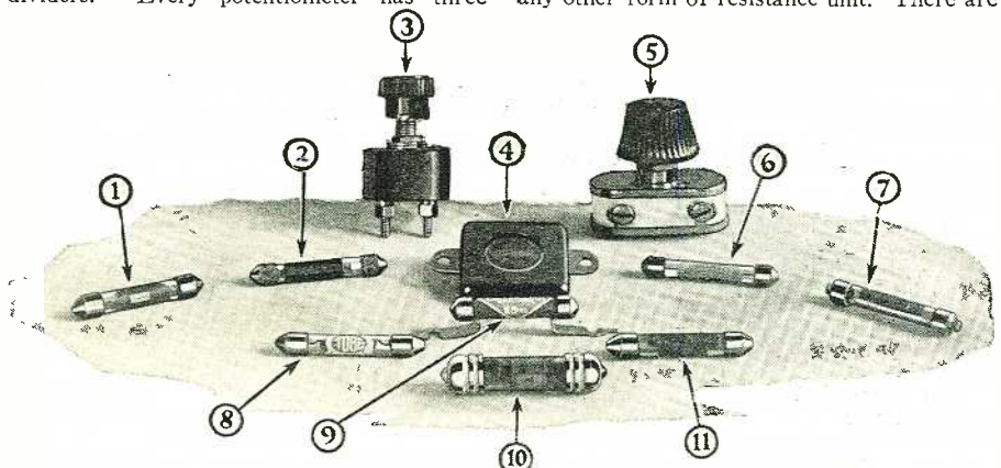
Fig. 9. Above are shown a number of fixed and variable resistors designed for use as grid leaks in connection with vacuum-tube detectors, and as plate and grid resistors in radio- and audio-frequency resistance-coupled amplifiers. Nos. 3 and 5 are variable grid leaks. 3 has a range up to five million ohms, and 5 to 10 million ohms. The fixed resistors shown in the foreground are all of the new type, and can be relied upon to retain their stated values under practically all conditions. (Courtesy of: 1, Dubilier Condenser & Radio Corp.; 2, Leslie F. Muter Co.; 3, Martin-Copeland Co.; 4, Micamold Radio Corp.; 5, Allen-Bradley Co.; 6, International Resistance Co.; 7, Electrad, Inc.; 8, Tobe Deutschmann Co.; 9, The Carborundum Co.; 10, Ansco Products, Inc.; 11, Daven Radio Corp.)
