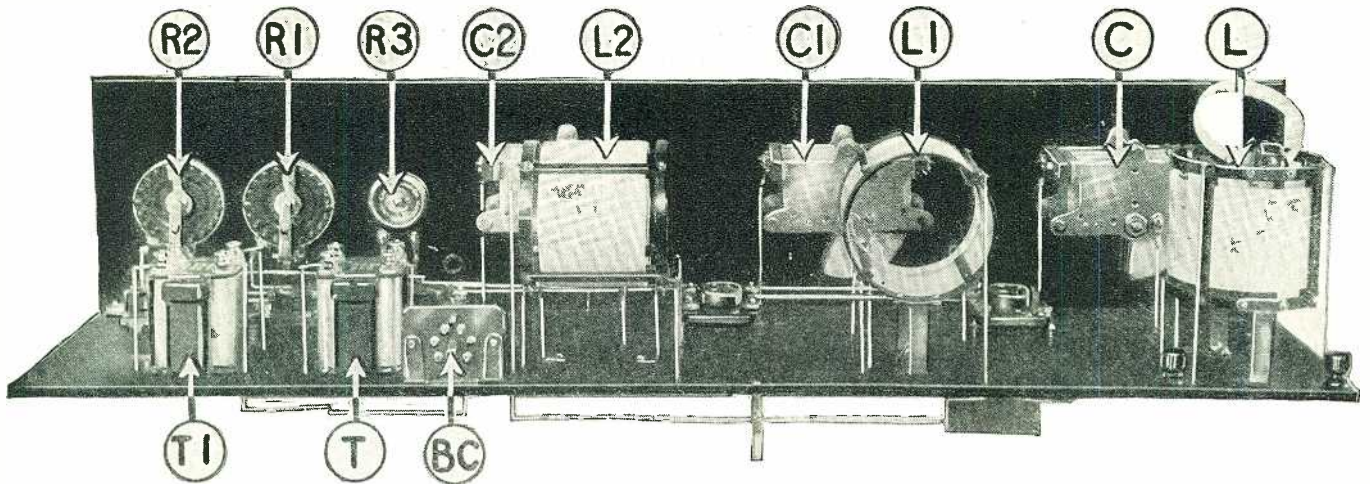
A rear view of the Aero-Dyne receiver. L is the aerial coupler; L1 and L2 are the R.F. transformers; C, C1, and C2 the tuning condensers; R3 is the variable resistance, common to the R.F. tube plate circuits; R1 and R2 are the filament rheostats; T and T1 the A.F. transformers; and BC is the battery-cable receptacle.
