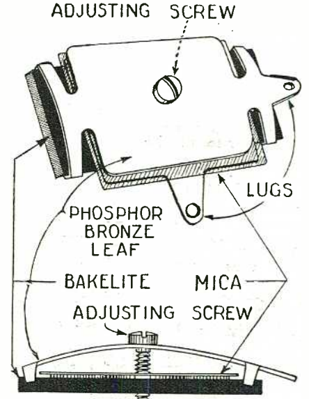
These perspective and side views of the midget condenser show its simple construction plainly. Illustration courtesy the Hammarlund Mfg. Co.
