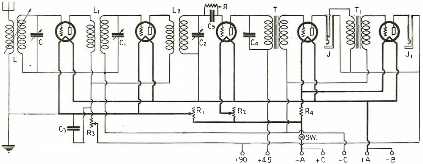
The schematic circuit diagram of the completed Aero-Dyne receiver. The author stresses the fact that the circuit in itself is not unique, but its application in obtaining maximum amplification is its real point of superiority.
