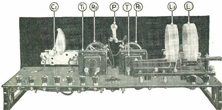
A rear view of the receiver. C1 is the condenser controlling regeneration; T and T1 are the A.F. transformers; R1 and R2, rheostats; P is the pilot light, and L and L1, the "wound-on-air" inductances, are the antenna coil, and secondary with fixed tickler, respectively.
