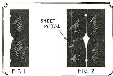
Details of a metal template employed for engraving dial indicators on panels.
