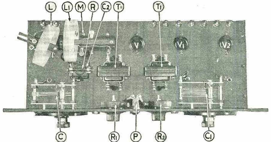
Looking down on the sub-panel. C is the tuning condenser; M, the coil mounting; V, V1, and V2 are the detector and two A.F. tubes; C2 and R, grid condenser and leak respectively.
