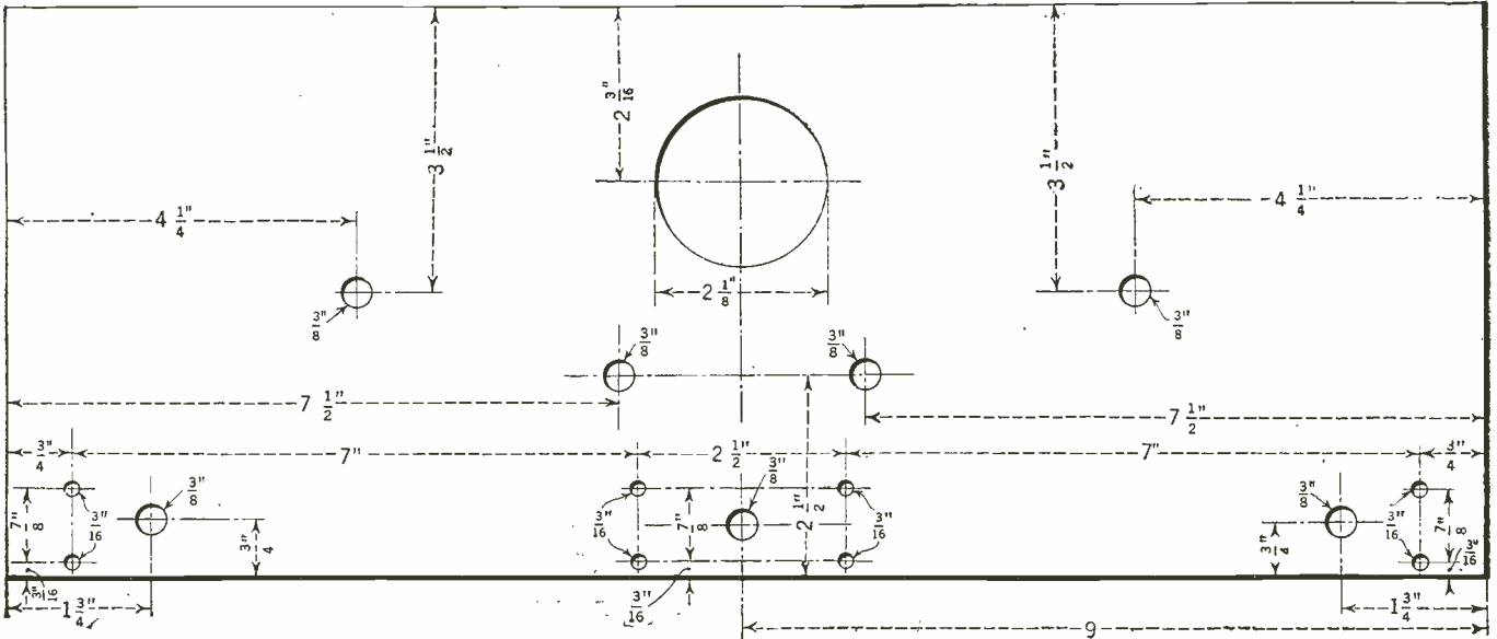
Above: Layout and drilling details for the panel of the RADIO NEWS Batteryless Receiver.
