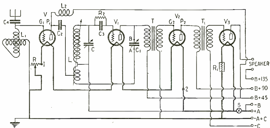
The schematic wiring diagram of the DX-2 receiver. V, V1 and V2 are contained in tube A, above illustrated. 1 and 2 mark the filament terminals.
