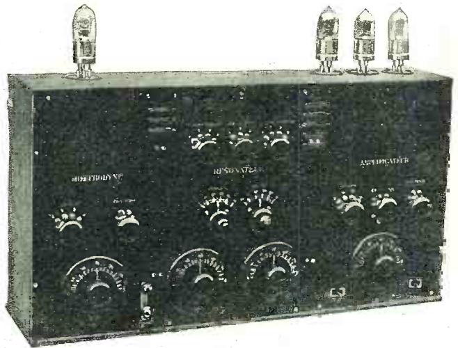
At the upper left is shown a French receiver, which embodies several novel features. The loud speaker has a specially-treated diaphragm and the loop antenna a double frame, on which there are two sets of windings. At the right is shown a French press-dispatch set, used in newspaper work, which is a typical example of the method of mounting the vacuum tubes. Notice the number of controls.
