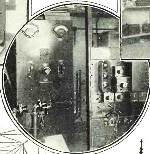
Above, at the left, appears the control panel for the motor-generator set, which furnishes power for the transmitting tubes; while at the right is a close-up view of the speech-amplifier panel.
