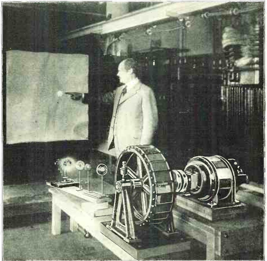
Fig. 2. Dr. Alexanderson in his laboratory indicating the seven light-spots, which are used in the method proposed by him for television. In the foreground is the drum on which are mounted the mirrors, with the motor for rotating it. A system of lenses may be seen, together with an arc light.
