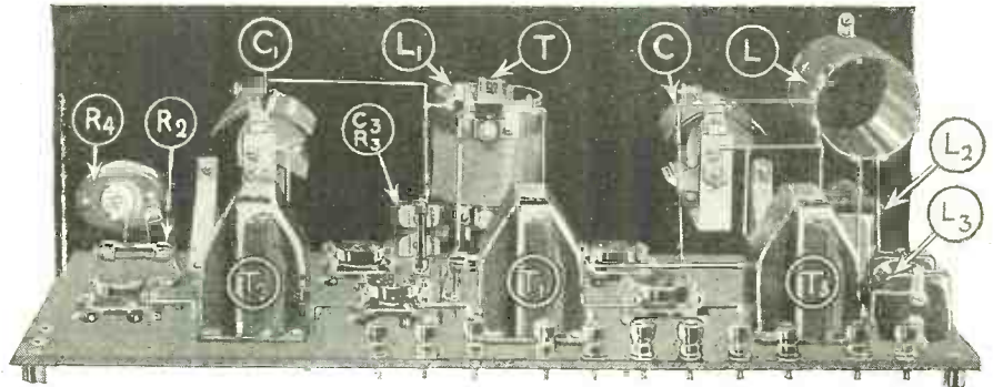
(Q. 2201). A top view of the Samson Dual T.C. receiver. A power tube is employed in the last audio stage to enhance the quality of reproduction obtained. A 500,000-ohm variable resistance to obtain volume control is also incorporated, and is indicated as R-4 in this view.
