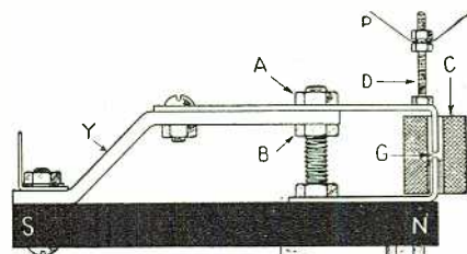
Side view of the loud-speaker unit, showing the details of driving mechanism.
