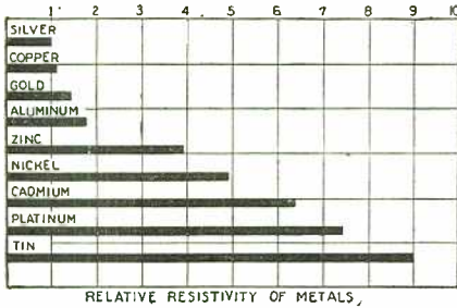
RELATIVE RESISTIVITY OF METALS,
