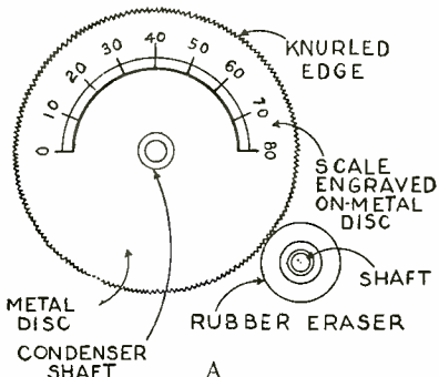
Details of the vernier knob and dial. A rubber eraser is used as the friction contact.
