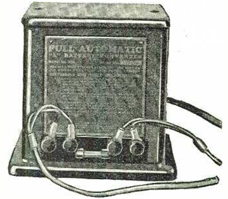
The complete automatic "A" battery charger. It is about seven inches high, five wide and four deep, and is made almost entirely of steel. Illustrations courtesy Apco Mfg. Co.
