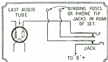
Simple jack-wiring arrangement to cut out automatically the loud speaker when the phones are plugged into the last stage.
