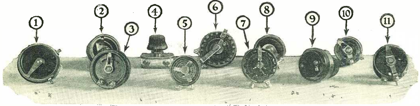
Fig. 1. A large group of rheostats of the more usual type, which are made in resistance values ranging from 1 ohm to 100 ohms. The one shown at No. 4 is of the carbon disc compression type. No. 5 has the resistance wire wound on a metal core which is insulated with an enamel coating. It will be noted that Nos. 6 and 7 have the resistance units supported so that a large air space is available for cooling purposes. Rheostat 9 is entirely enclosed in a combination metal-and-insulation case.
