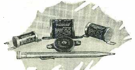
Three of the new rolled condensers are shown in this illustration, along with one of the piled type (in the center behind the pencil). The left hand condenser has a capacity of .25 mf., the center and right hand ones .5 mf. each. The piled-type condenser (circular) is Size .00025-mf. Compare the sizes of the condensers with that of the pocket pencil.
