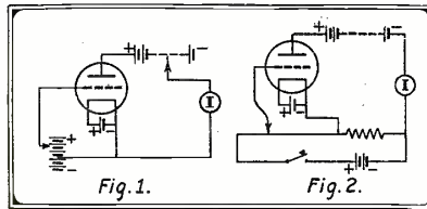
Two Methods of Determining Space Charge Valves.
