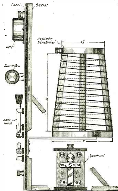
Side View of the Transmitter Showing the Oscillating Circuit and the Frame Holding the Panel.
