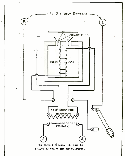
Diagram of the New Telemegafone, Showing the Functioning Principle of This Instrument. Note the Coil Fixed to the Diaphragm.
