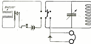
Diagram of the Wave-Meter Which May Be Used to Tune Both Transmitter and Receiver.
