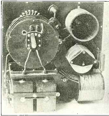
Fig. 2. Inside View of the Complete Portable Set Designed and Built by Mr. D. R. Clemons. Everything is Fixt on the Front Panel in a Very Clever Way.
