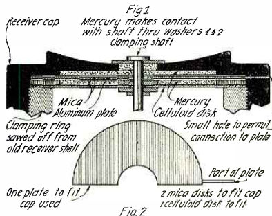
A Variable Condenser of this Type, Built in an Old Receiver Cap Saves Space and Has Great Capacity as Mica is Used for a Dielectric.
