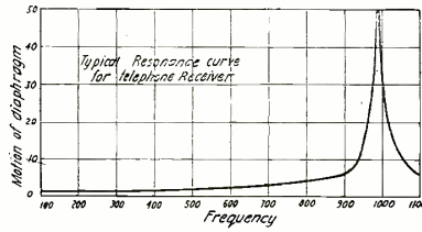
Resonance Curve of a Telephone Receiver, the Vertical Dimensions Representing the Amplitude of the Vibrations and the Horizontal Dimensions, the Frequency.
