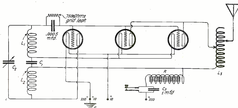
Diagram of Chief Operator Daggett's Transmitter. One V.T. is Used as an Oscillator, While the Two Others are Used to Amplify the Oscillations of the Master Oscillator. This Hook-up is one of the Best Actually Known for C.W. Transmission.
