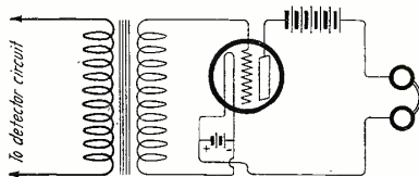
Fig. 1 Hook-up of a One Tube Audio Frequency Amplifier. If Other Stages of Amplification Are Added the Primary of the Second Amplifying Transformer is Connected in Place of the Fones.
