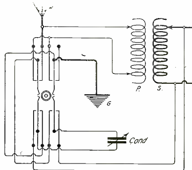
If You Own Only One Variable, Hook it Up Like This and You Can Switch it in Any Circuit.
