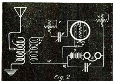
In This Regenerative Hook-up Variometers are Used to Tune the Grid and Plate Circuits.
