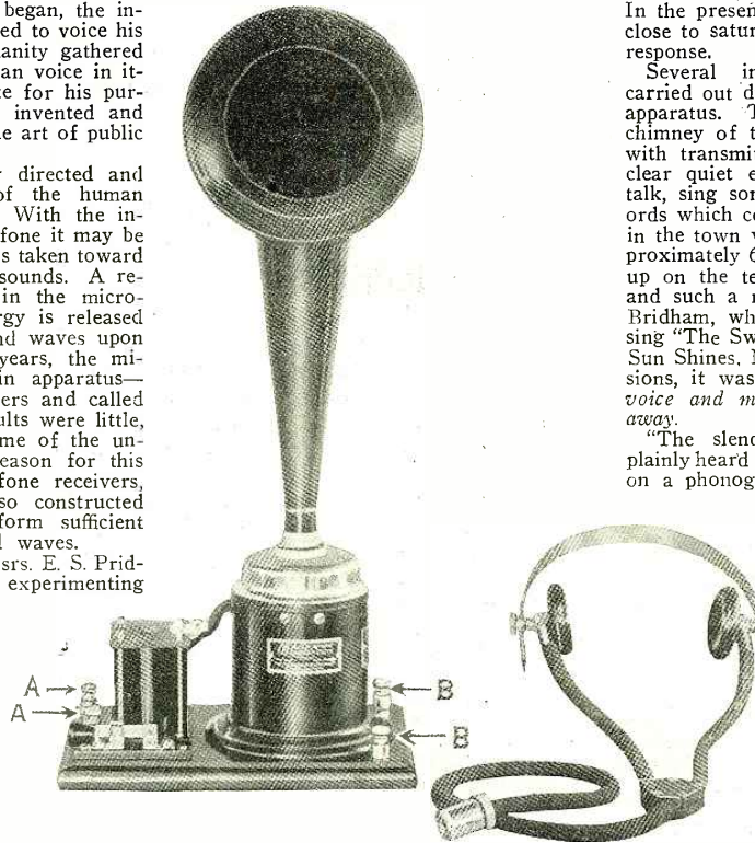
Fig. 3. Photograph of the New Loud Talking Machine Which Amplifies Weak Signals to Such a Volume That They Can Be Heard by a Whole Audience a Great Distance From the Receiver.
