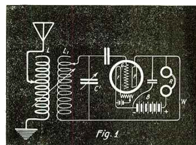
Here is the Well Known Ultra Audion Circuit Which is the Simplest Regenerative Hook-up.
