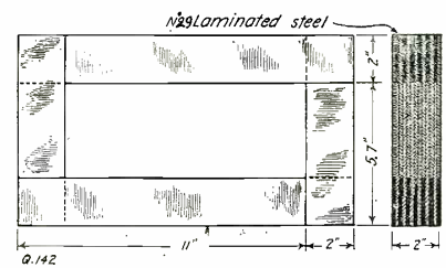
Diagram of the Iron Core for a 1 KW. Transformer. Note the Arrangement of Steel Strips Which Are Made of No. 29 Laminated Steel.
