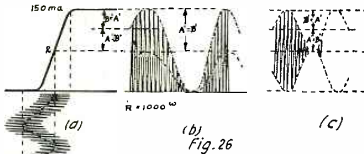
With the Grid Bias Set So That the Radio Grid Oscillations Are Suppress in the Plate Circuit the Peak Value of the Radio Oscillation Just Reaches the Saturation Part of the Curve.
