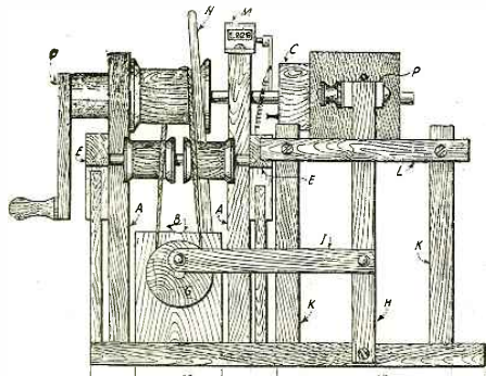
Front View of the Winding Machine. Note the Clever System Allowing the Spacing Between Turns to be Changed.
