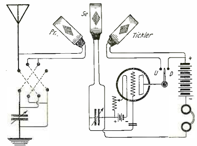
The Standard Hook-up for an Audion With 3 Honeycomb Coils. With This Set Spark Signals May Be Received as Well as Undamp Waves.
