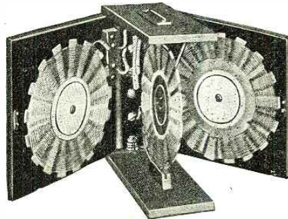
Illustration shows front of cabinet removed Formica Insulation Thru'out Patent Pending Dimensions, 4½ x 5 x 1¼
