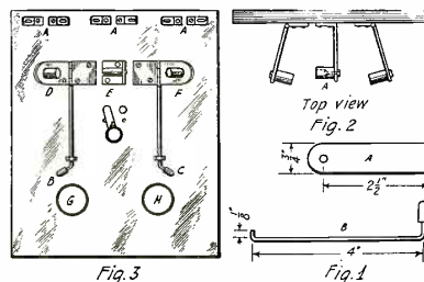
A Clever Idea for Mounting the Home Made Honeycomb Coils or Others That are Sold Without Plugs.
