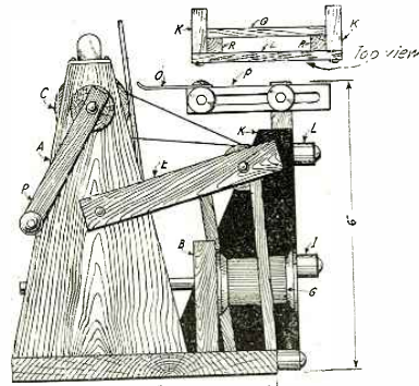
Side View of the Machine, Showing the Needle by Means of Which the Wire is Applied on the Coil, and Which is Moved Away as the Diameter of the Coil Grows.
