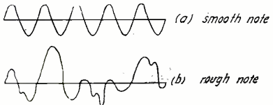
Type of Oscillations Obtained with a Rotary Gap When (a) Well and (b) Badly, Adjusted.
