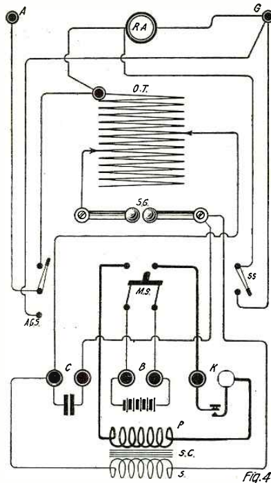
Wiring of the Panel; for the Sake of Cleanness, the Vibrator of the Spark Coil is Omitted.
