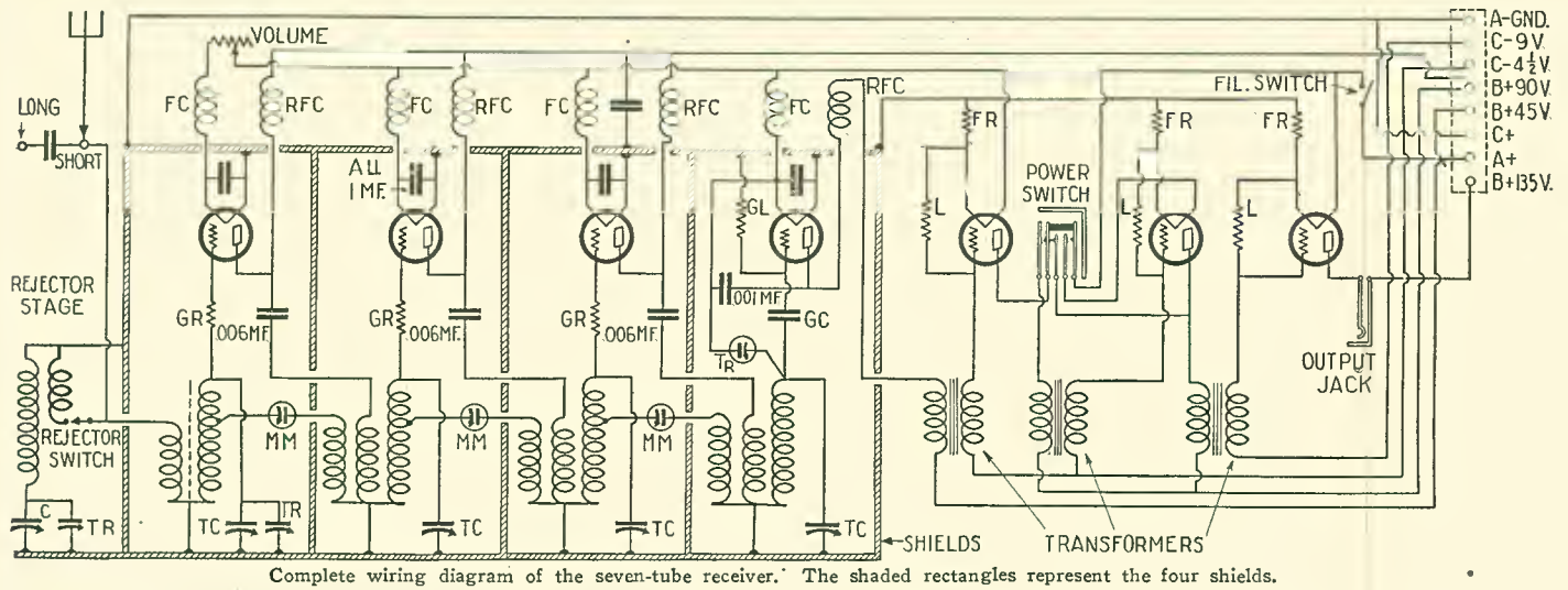
Complete wiring diagram of the seven-tube receiver. The shaded rectangles represent the four shields.
