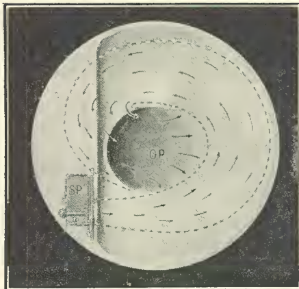
Phantom view of the operating section of the loud speaking, showing the loud-speaking unit, SP, and the opening, OP, through which the signals emerge. The arrows indicate the direction of the sound.
