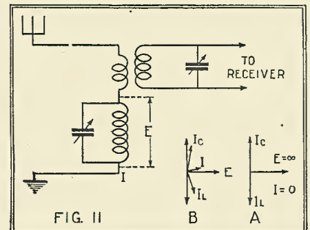
A diagrammatic illustration of the functioning of the type of wavetraps shown in Fig. 2.
