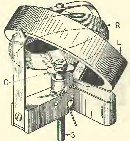
A variable inductance employing a metal ring as the principal control factor. The coil L is also tapped, so that it can cover wide inductance ranges.
