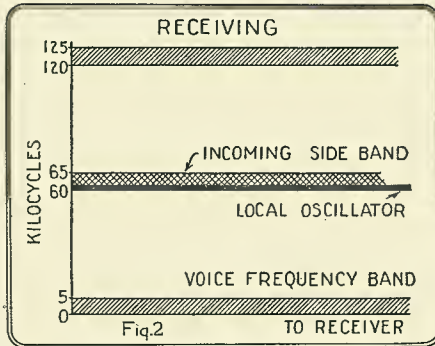
The "beating" of the incoming side band with a locally-generated wave of 60 kc. reduces the frequency to audibility.
