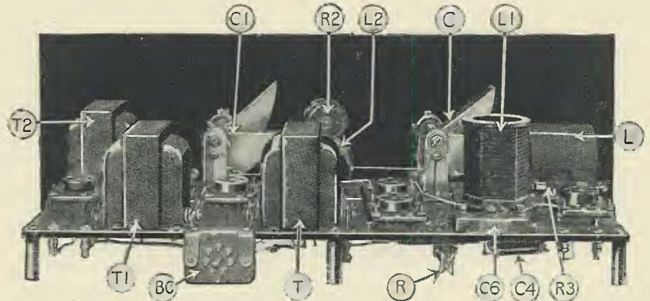
A rear view of the Ultra-5 receiver. The parts are: L, antenna coupler; LI, long wave R.F. transformer; L2, oscillator coupler; C, tuning condenser; C1, oscillator condenser; C4, by-pass condenser; C6, coupling condenser; R, grid leak; R2, volume control; R3, automatic filament control; T, T1, A.F. transformers; T2, output choke, and BC, the battery cable receptacle.
