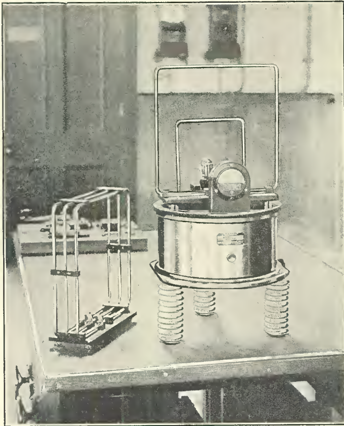
The wave-meter of the short-wave station at Bodmin, for checking the accuracy of the transmitter's wave. The coil of a radio compass, used with the meter, is shown at the left. © Herbert Photos, Inc.
