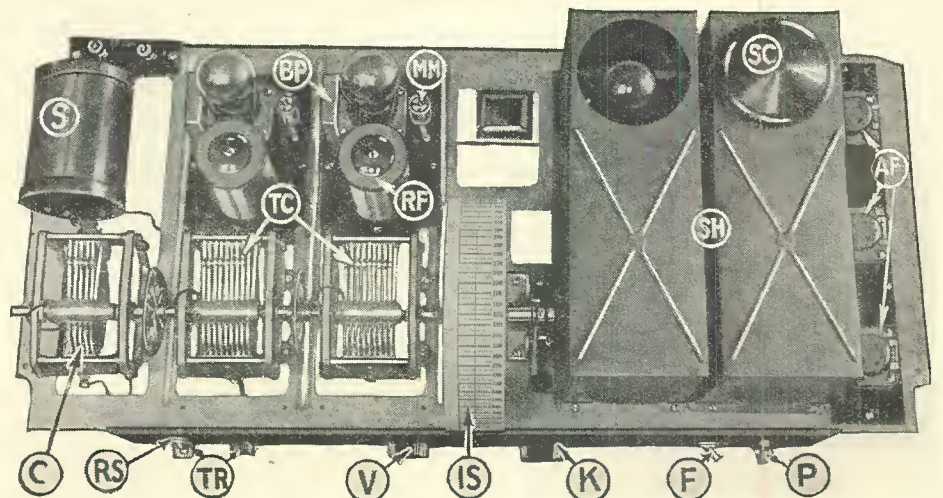
Top view of the receiver chassis. The copper shields of the first two R. F. stages have been removed to expose the instruments.
