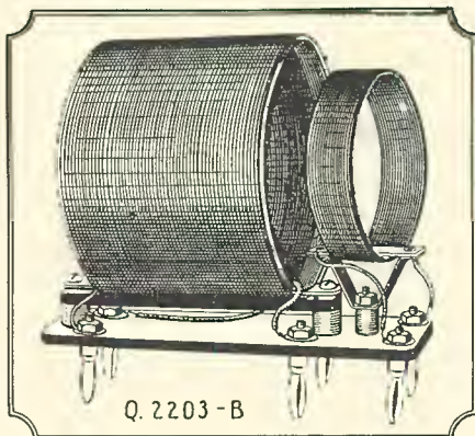
The appearance when completed of the coil L 1 , which is used in the Henry-Lyford receiver. L 2 is very similar in construction, except that the third or semi-variable winding at right is omitted. Plug-in mountings are used so that coils of various inductances may be employed.
