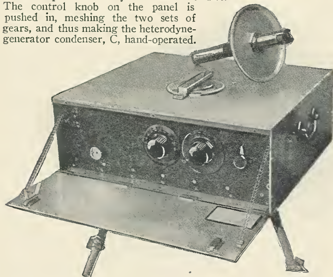
Fig. 7. In order to set the index of the direction finder on the true north use is made of a magnetic compass, here shown in place of the loop antenna.
