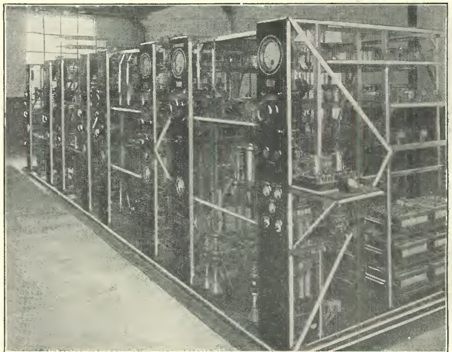
Four amplifier panels in the Bodmin station for transmitting by the radio beam system. © Herbert Photos, Inc.
