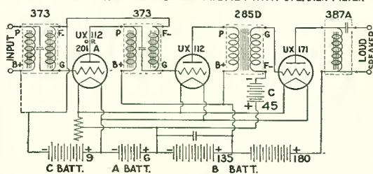
SCHEMATIC DIAGRAM FOR COMBINATION 2 STAGE DOUBLE IMPEDANCE COUPLED AND 1 STAGE TRANSFORMER COUPLED AMPLIFIER WITH SPEAKER FILTER
