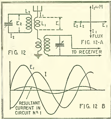
Illustrating the operation of the wavetrap circuit shown in Fig. 1.
