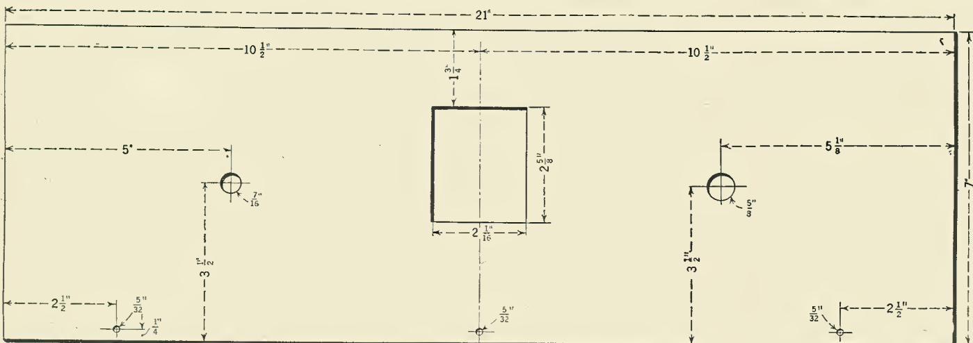
Details for the panel drilling. There are very few holes, as the gang condenser unit is mounted on the wooden baseboard. Actually, the only instruments mounted on the panel are the volume control and the filament switch.
