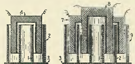
Tuned R.F. transformers, the inductance of which is varied by sliding the coils along the surfaces of metal tubes.
