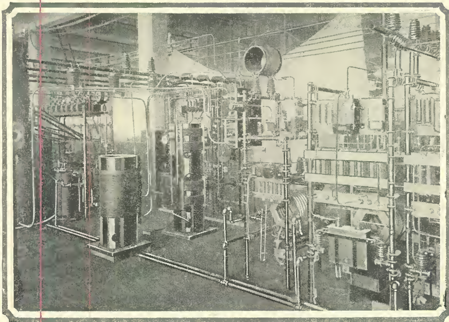
An idea of the wiring of the 80-kw. transmitter may be had from this illustration. Note that tubing is used, for the most part, instead of busbar.
