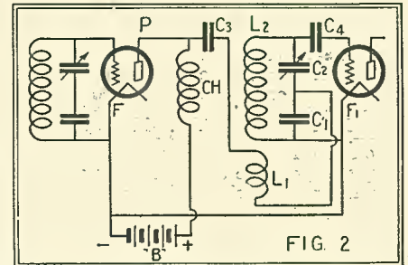
A circuit embodying the Loftin-White principle. It is non-reactive and provides constant electrical coupling at all broadcast frequencies. Note that the primary L_1 is "floating."
