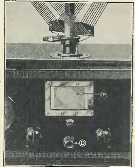
Close-up of a typical loop receiver, showing the "direction finder" attachment completely installed. The loop is turned by means of the knob D. P is the pointer on the map.
