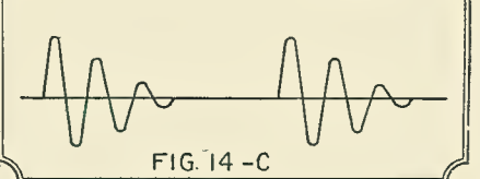
Illustrating Fig. 14-B the transient and steady electrical states of the trap circuit of Fig. 14-A, shown above, and the effect of spark interference, Fig. 14-C.
