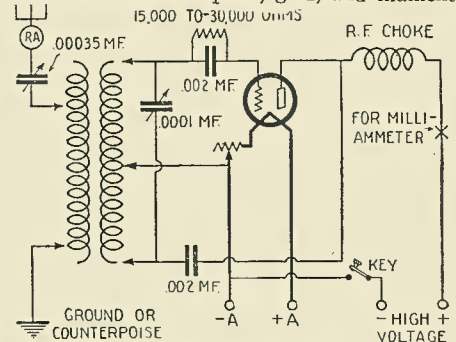
Fig. 2. The schematic circuit diagram of a short-wave transmitter employing a single vacuum tube. This is known as the Hartley circuit.
