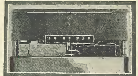
Fig. 4. The rear of the cabinet, showing the two-volt "A" battery and the 90-volt "B" battery.
