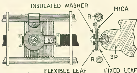
Detailed drawing of the "vernier" condenser mechanism.
