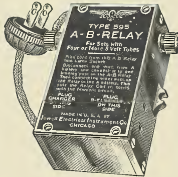
A-B Relay
