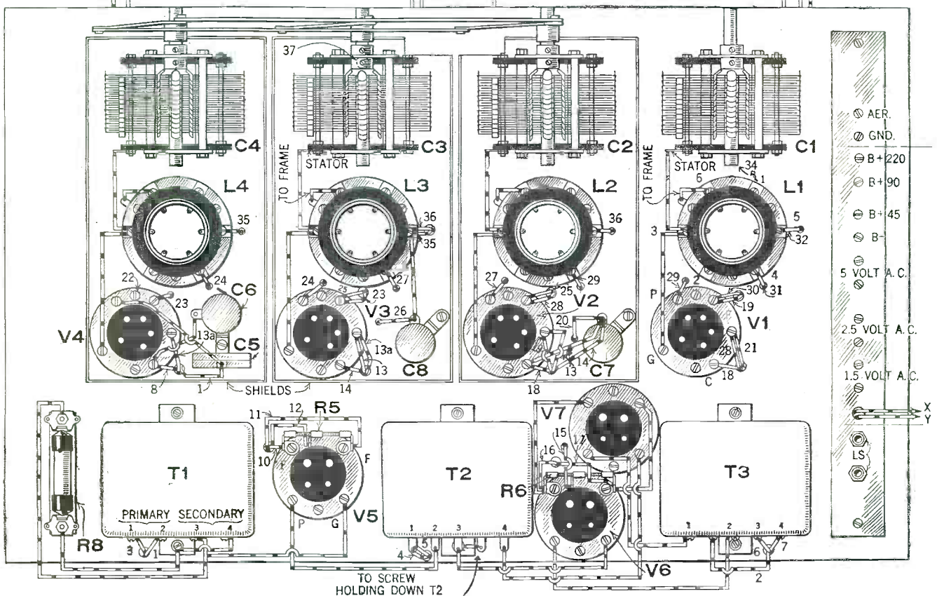
How the connections are made to the pieces of apparatus that are mounted on top of the sub-panel. The components are lettered to correspond with the other illustrations and list of parts. The link connectors for the condensers are illustrated to aid the constructor.
