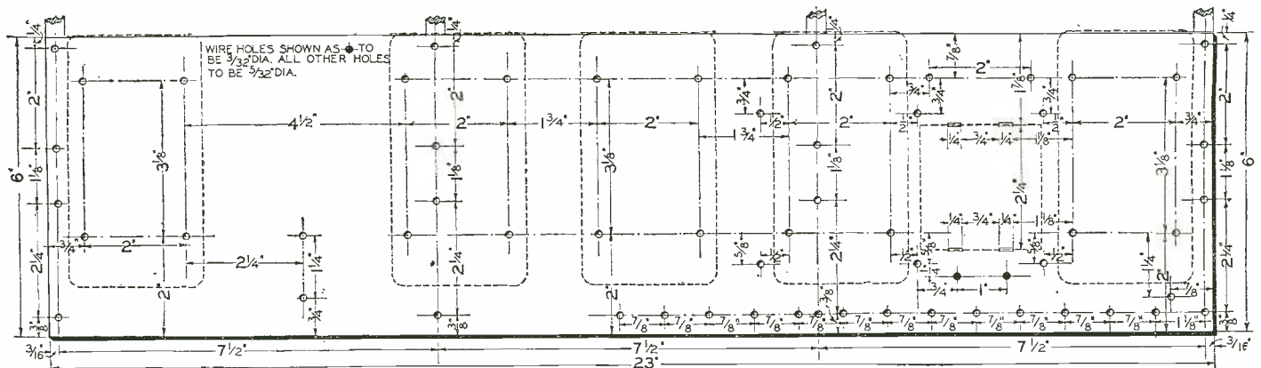
Drilling layout of the sub-panel, showing the exact location of every hole. This panel should be drilled and the fit of each part carefully tested before the instruments are mounted permanently upon it. The
