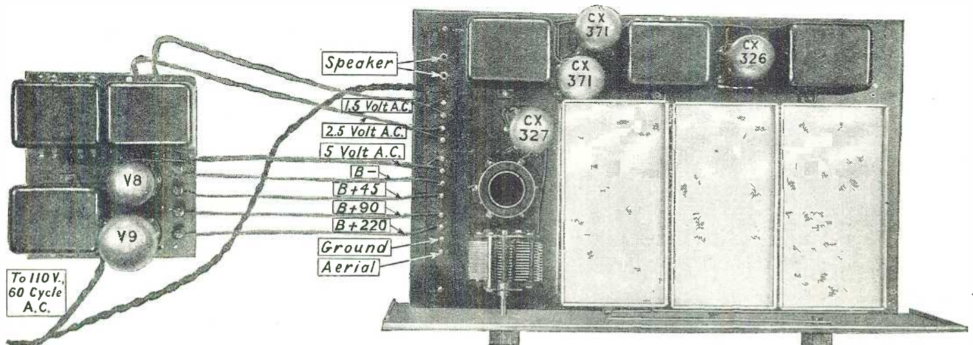
The power unit is here connected to the receiver. The connecting leads should not be more than four feet in length and may be of No. 14 lamp cord. V8 is the rectifier and V9 the voltage regulator tube.
