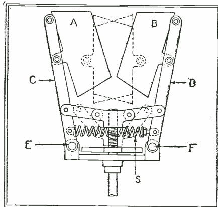
This toggle-joint mechanism is used to obtain straight-line-frequency tuning from rectangular plates in a British condenser.
