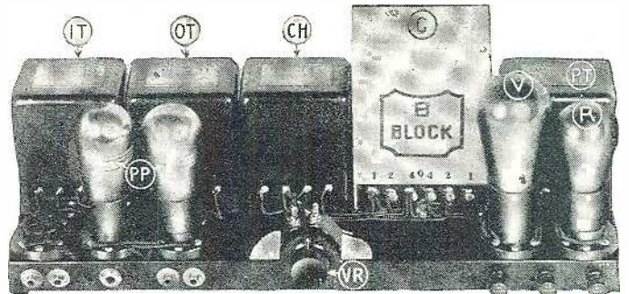
FIG. A. The picture at the right shows one of the latest push-pull power-packs, complete with a 180-volt "B" power unit and voltage-regulator tube. This compact unit is operated from the first stage of audio-frequency amplification of any standard receiving set. Photo by courtesy of Siler-Marshall, Inc.
