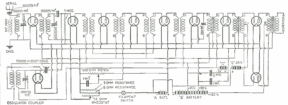
The complete hook-up of the Tyrman Ten. The set uses one stage of straight R.F. and three of intermediate-frequency amplification. The locally-generated oscillations are transferred to the "mixing" circuit of the first detector (the second tube from the left) through the .00005-mf. midget condenser.
