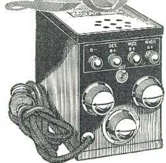
Model R-81
