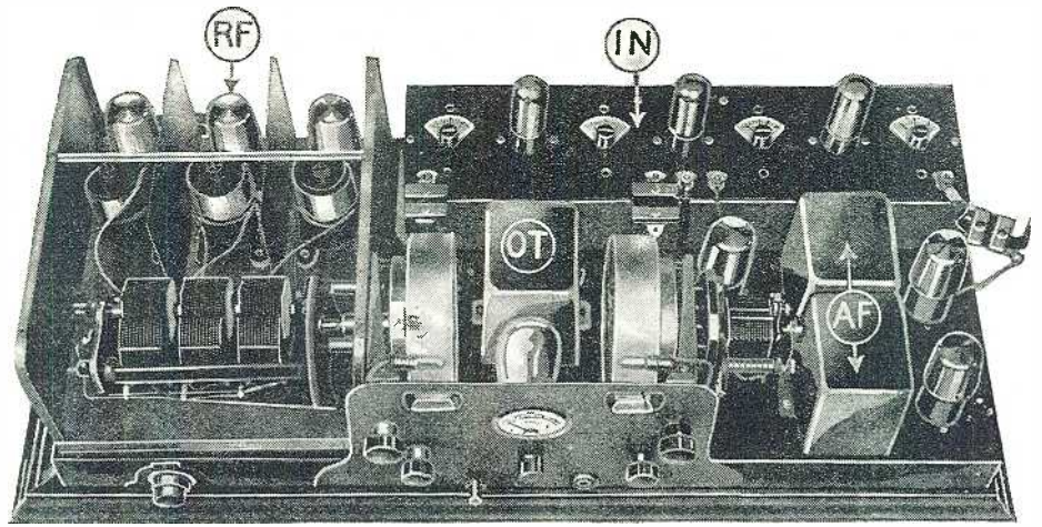
General view of the receiver, with the cabinet removed. R.F., two-stage tuned R.F. amplifier unit, with top shield removed; IN, Infradyne amplifier unit; A.F., audio transformers; O.T., output transformer. The variable condensers are controlled by illuminated dials of the edgewise-drum type.
