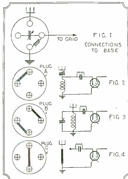
How the three plug-in switches of Mr. Baymar will effect, respectively, changes in the tuning circuit.
