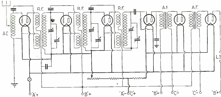
Complete schematic hook-up of the six-tube receiver. The R.F. amplifier is of the neutrodyne type, comprising two tuned and one untuned stages; while the A.F. portion uses regular transformers. AC, antenna coil; R.F., radio-frequency transformers; A.F., audio transformers; L.S., loud-speaker posts.
