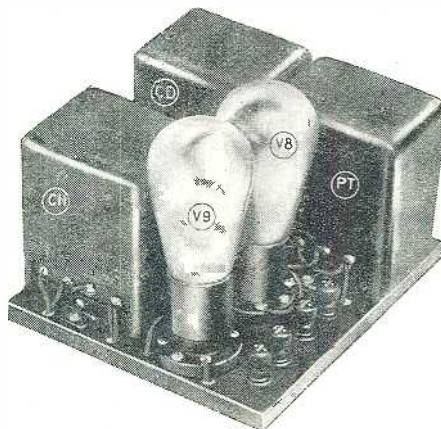
Complete power unit of the A.C.-tube light-socket receiver, showing its compactness.
