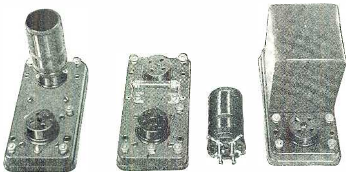
Left: R.F. unit, showing coil in place; center, detector unit, with coil alongside; right, A.F. unit. Each, with the addition of a tube, is a completely self-contained stage of a receiver. Illustrations courtesy Pilot Mfg. Co.
