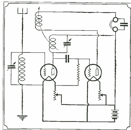
Any three-element vacuum tubes can be used in this circuit, which requires no plate ("B") battery for them.
