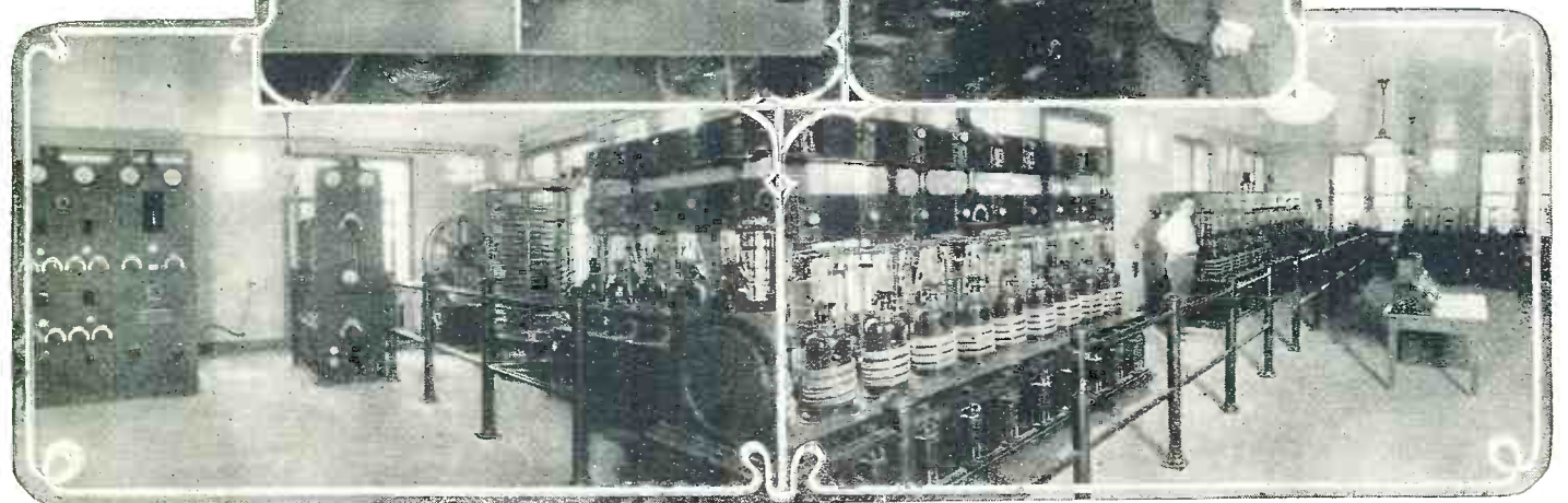
A general view of the 32 high-power radio tubes (rated at 20 kilowatts each) used in the new WEAF transmitter. The control table is shown at the right.
