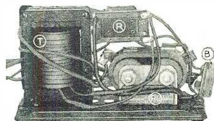
The insides of the charger. T, step-down transformer; R, switching relay; RU, rectifier unit; B, receptacle for "B" supply unit.
