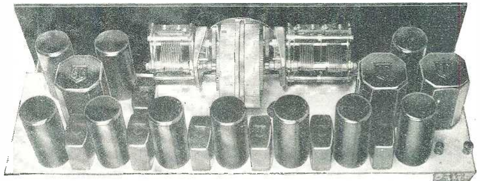
Rear view of the Tyrman Ten. The upright cylinders are individual metal shields for the tubes. The parts are so arranged that all the connections are very short and direct. The Flewelling "capacity connector" is used, eliminating most of the wiring and much of the task of the constructor.
