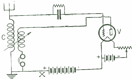
The "B+" is connected to the aerial coil, and thus also grounded. This circuit is said to be more efficient than a standard single-tube regenerative hook-up.
