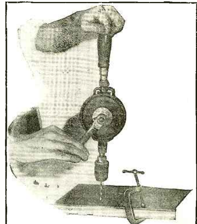
The correct way to hold the drill. Here the top of the hole is directly above the bottom of the hole and correct placement results. Note also that the work to be drilled should be clamped firmly to a bench or table so as to prevent slipping, etc.
