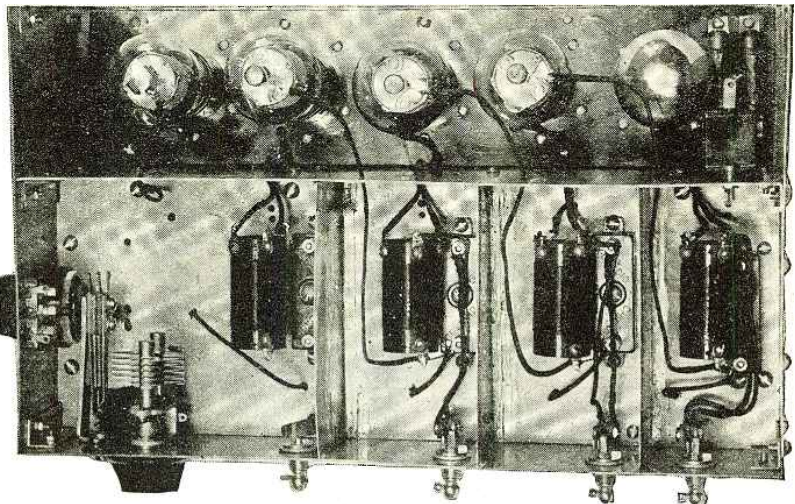
Looking down on the experimental receiver, with top removed; showing the arrangement of coils and switches for cutting in extra capacity to cover the higher wavebands
