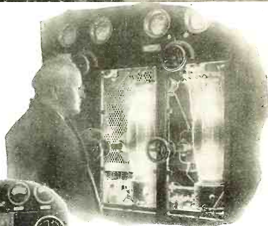
Above, operating the short-wave receiver. The 800-watt short-wave transmitter being visible in the background
