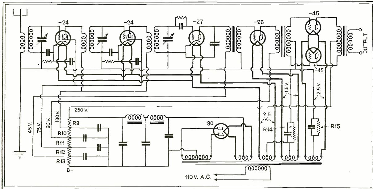
The circuit diagram below shows the application of the voltage divider circuit of Fig. 3 as incorporated in a completely a.c. operated receiver with push-pull output
