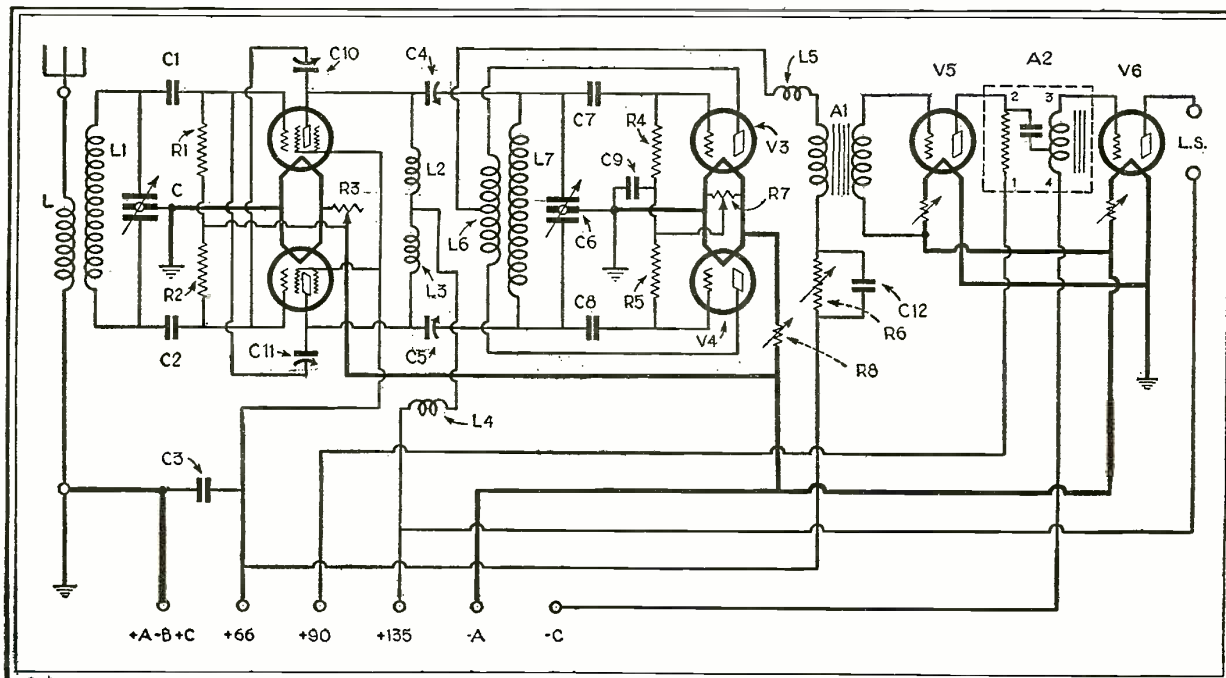
Fig. 4—The complete circuit diagram of Mr. Marshall's push-pull short-wave receiver. The coils L-1 and L6-L7 are of the plug-in type, allowing change of tuning in the wavelength bands
