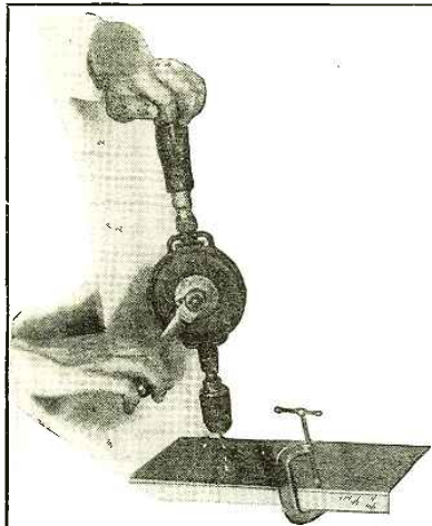
The wrong way to hold a drill. If the panel or material to be drilled is of any considerable thickness, holding the drill away from the vertical will produce a hole running diagonally through the panel and thus throw off the alignment of units to be mounted in those holes
