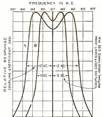
These curves illustrate the band pass filter characteristic of an inductively coupled filter with curve A having coupling coefficient of .0251 (2.5%) and B with a coupling coefficient of .0094 (.94%) and mutual inductance of 2.25 microhenries at 350 meters
