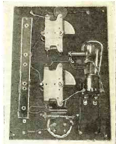
Back view of the transmitter with coils removed. The above photograph and panel layout in Fig. 7 clearly indicate the layout and placement of parts
