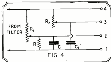
Diagram of the voltage regulator section of an eliminator. Various voltages are obtained by the use of resistances R, R-1 and R-2.
