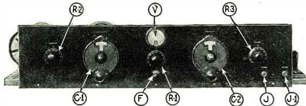
Front view of the Infradyne. V is the filament voltmeter; R-1, 30-ohm rheostat; F, the filament switch; and J and J-1 the first and second stage audio stage jacks. The other letters correspond with those in the illustration above.
