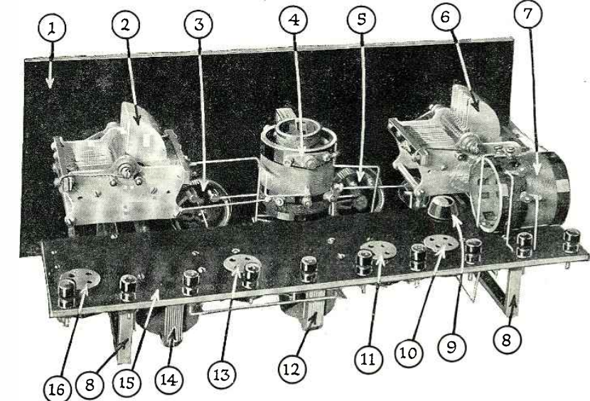
No. 1 is the 7x18 panel; 2 and 6, variable condensers; 3 and 5, rheostats; 4, 3-coil tuner; 7, antenna coil; 8, supporting brackets; 9, balancing condenser; 10, 11, 13, and 16, tube sockets; 12 and 14, A.F. transformers; and 15, 4 x 16\frac{3}{4} sub-panel.
