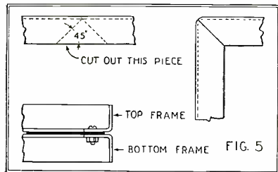
If these directions are followed for the amplifier-case construction, the finished job will be neat and the work required for its completion, a minimum.
