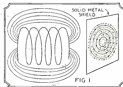
From a sketch showing eddy currents set up in solid metal shielding placed within the field of an inductance-coil.
