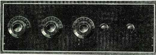
The three tuning controls have the same dial readings; this being due to the "balanced-bridge" circuit employed in the radio-frequency amplifier.
