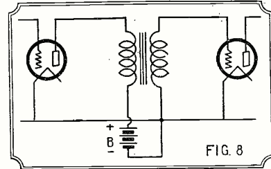
The typical transformer-coupled audio-amplifier circuit arrangement.
