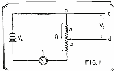
In this simple circuit the current in the resistance R is measured by the ammeter, I . The variable resistance or "voltage divider" permits the voltage, V_2 , across C and D to be varied.
