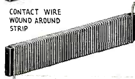
After the contact wire has been wound about the resistance strip, the wire is cut, to avoid short-circuiting the resistance. It is then assembled about a core, being held in place by a bakelite ring. The finished assembly is shown at the right.
