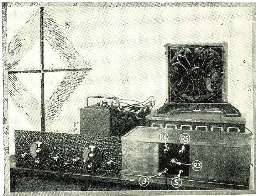
Fig. 2. All that is necessary for first-class reception of radio concerts. The amplifier and "B" eliminator on the right magnify the signals from the loop receiver on the left.
