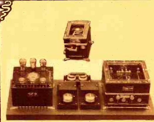
The apparatus shown above was designed to eliminate the constant human watch for SOS signals and will respond automatically to a series of four-second dashes which, it is suggested should be used as a forerunner of all SOS calls. Above is the four-second sender, which is connected to the transmitter; at the left is the receiver and at the right the selector unit for interpreting the signals and ringing the bells in the center. © Herbert Photos.
