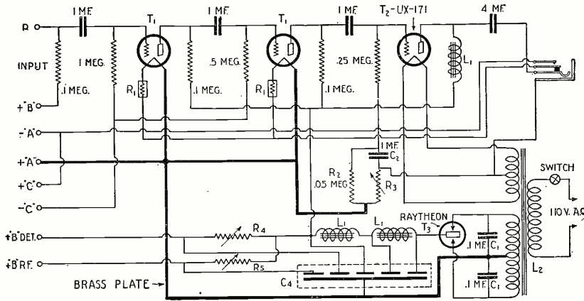
FIG. 1 The three amplifier tubes and the rectifier tube, together with the other apparatus, make this not only an excellent amplifier, but a "B" eliminator as well.
