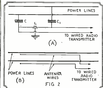
The two methods commonly employed for coupling carrier-current apparatus to power lines.
