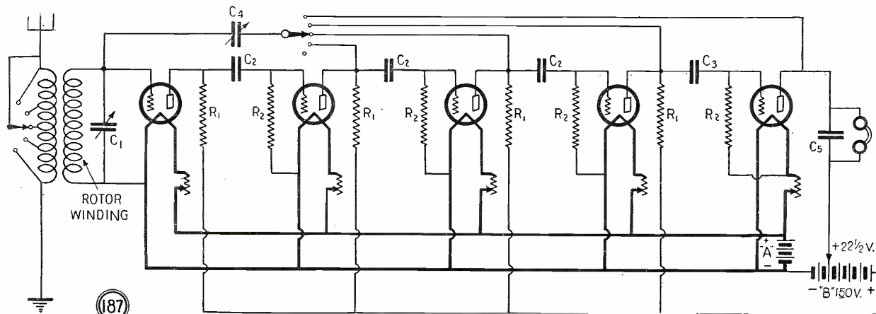
This particular type of circuit may be constructed by those desirous of reception that is free from noises. Resistance-coupled amplifiers are known for their ability to amplify without in any way contributing to the disturbance created by "atmospherics."
