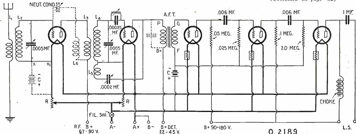
A composite 5-tube set, whose peculiar features are a combination to make up a set that will be noted for its performance. It consists of a neutralized tuned RF stage, a modified Hartley type of detector, one stage of transformer-coupled audio-frequency amplification, and two stages of resistance-coupled audio-frequency amplification.
