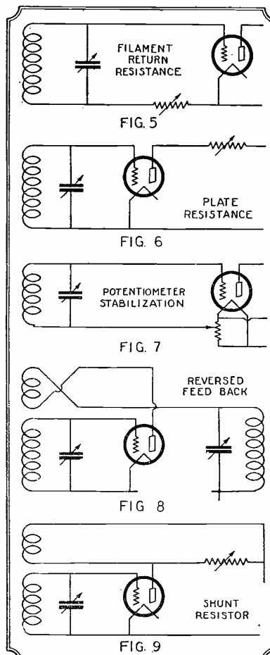
Figs. 5 and 6 show methods of controlling oscillation with variable resistances; Fig. 7, by a potentiometer; Fig. 8 by counter E.M.F.; and Fig. 9, by damping.
