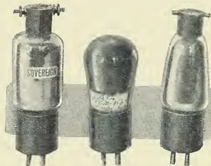
Three types of tubes, whose filaments are heated by raw alternating current.
