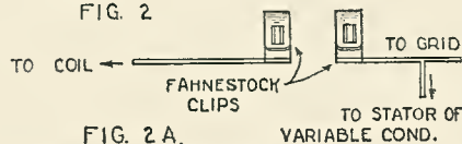
Fig. 2 shows the circuit diagram of the loop antenna for the Strobodyne; and Fig. 2A, how the connections can be easily made.
