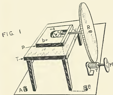
The apparatus for conducting rectifying experiments between a spherical surface and a plane. By means of the wheel M , as explained in the text, the distance between the sphere and plate can be regulated to less than a millionth of an inch.
