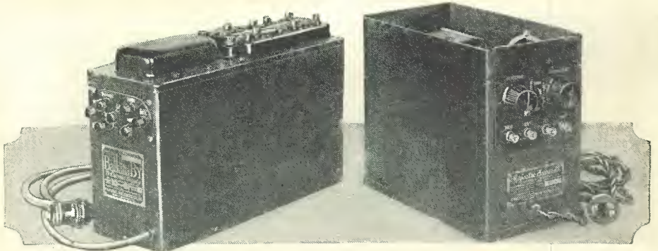
The "B" socket-power unit at the left is of the chemical type; and the other uses a rectifier tube. Photo by courtesy of Faustel Products Co. and Grigsby-Grunow-Hinds Co.
