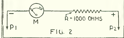
Fig. 2 shows the voltage on load. Two methods of making voltage measurements.
