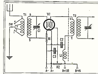
FIG. 2. THE TUNED METHOD OF ANTENNA COUPLING IS SHOWN HERE. THIS WILL IMPROVE THE SENSITIVITY OF THE SET FOR THE DX FAN, AND WILL ADD TO THE RECEIVER'S SELECTIVITY
