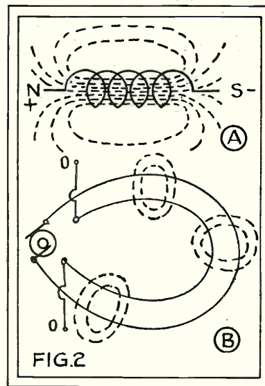
THE DOTTED LINES IN A INDICATE THE FIELD OF AN INDUCTANCE. THE THUMB RULE OF FIG. 1 ALSO HOLDS TRUE HERE. B ILLUSTRATES MUTUAL INDUCTANCE IN TWO COUPLED CIRCUITS
