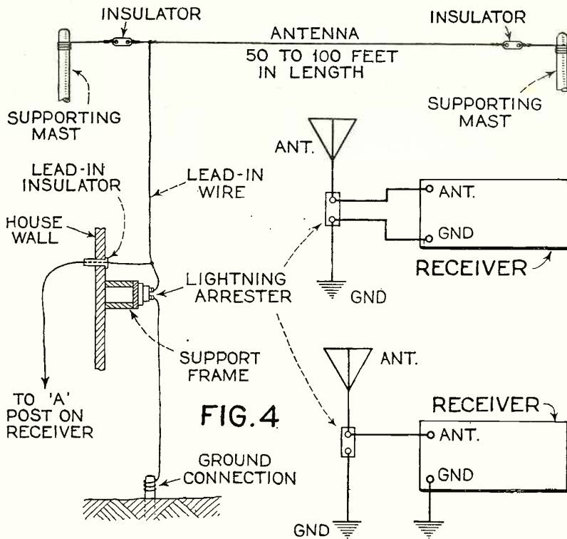
FIG. 4 THERE ARE SEVERAL WAYS IN WHICH A LIGHTNING ARRESTER CAN BE CONNECTED TO THE RECEIVER AND ANTENNA-GROUND SYSTEM. TWO ARE SHOWN ABOVE
