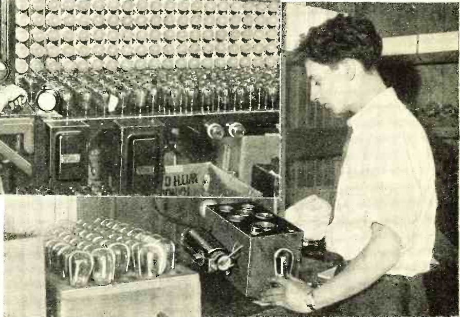
¶ Fig. 13—After “aging,” each tube is individually tested. In this particular case rectifiers of the full-wave type are being tested for possible departure from standard
