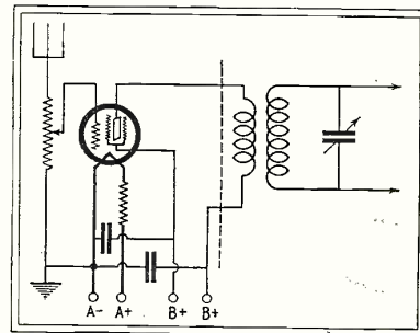
FIG. 1. THE ORIGINAL CONNECTIONS TO THE FIRST, OR ANTENNA STAGE, ARE SHOWN HERE; THE CHANGES ARE NOTED IN FIG. 2
