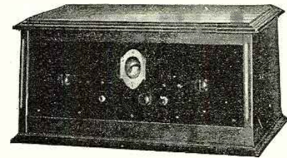
HOW THE FIVE-TUBE RECEIVER WILL LOOK WHEN FINALLY COMPLETED. ONE MAIN TUNING KNOB CONTROLS THE TUNING OF THE SET WHILE THE OTHERS CONTROL SENSITIVITY AND VOLUME
