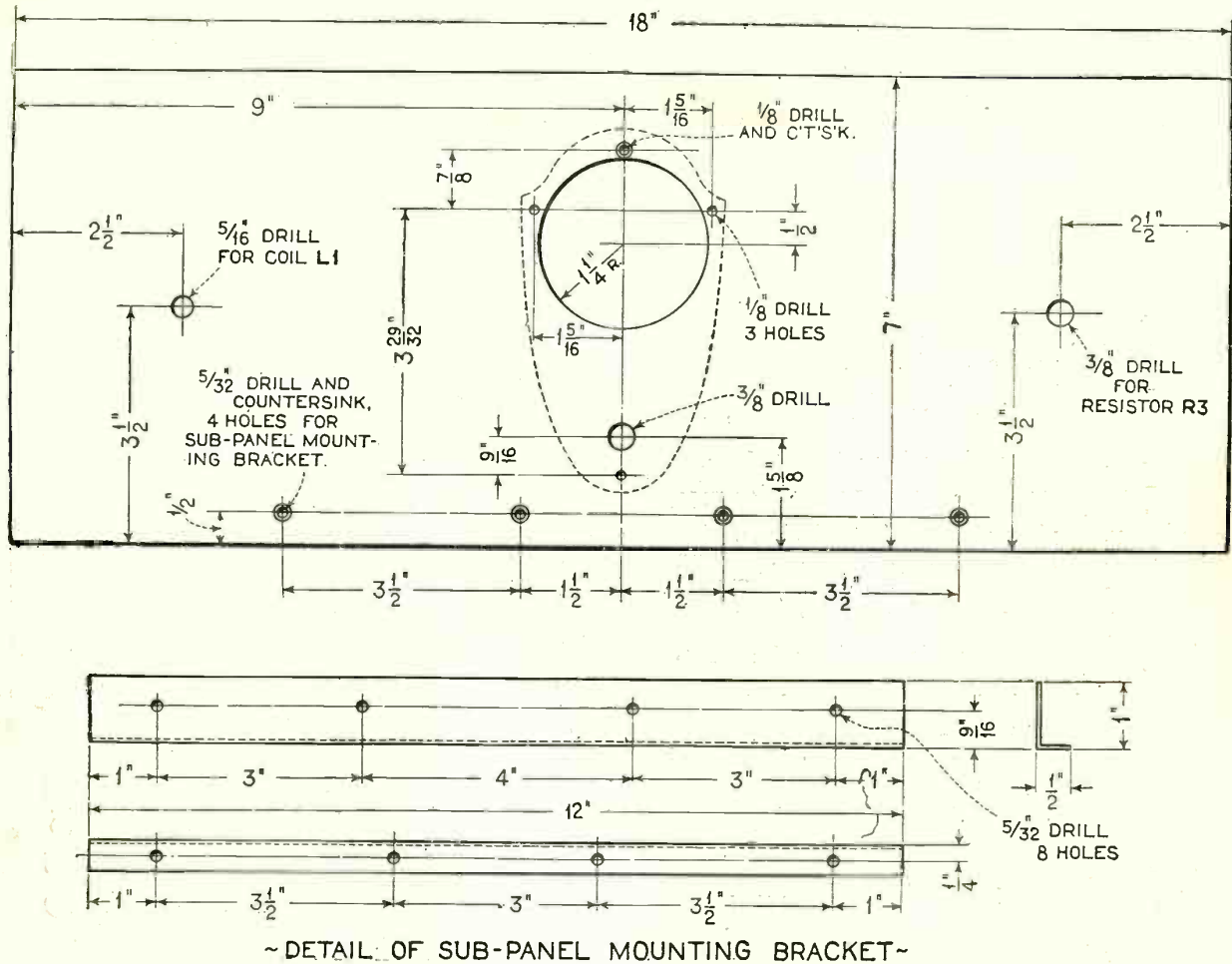
FIG. 3—THE DIMENSIONS OF THE PANEL MOUNTING BRACKET AND THE MAIN PANEL SHOULD BE CAREFULLY OBSERVED IN TRANSFERRING THE LAYOUT TO THE PANEL SO THAT THERE WILL BE NO CHANCE FOR ERROR
