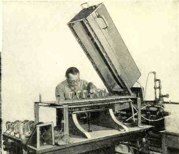
¶ Fig. 8—The Tubes are evacuated through the small glass tubing extending up inside the bulb. Evacuation is carried on with the filament lit and with heat externally applied
