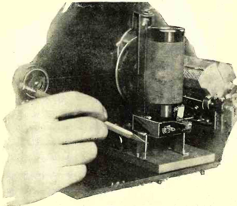
TO CENTRALLY LOCATE THE TUNING COILS WITHIN THE SHIELD CANS, THE COIL SOCKETS ARE MOUNTED ON BRACKETS, AS INDICATED HERE
