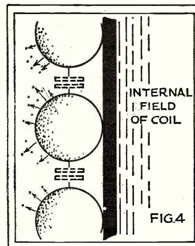
FIG. 4 THIS MAGNIFIED VIEW OF THE SIDE OF A COIL SHOWS THREE THINGS: THE INTERNAL FIELD OF THE COIL, THE CAPACITY BETWEEN THE ADJACENT TURNS AND THE SKIN EFFECT
