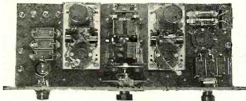
ABOVE IS THE RECEIVER HOUSED IN THE COMBINATION RADIO-PHONOGRAPH CONSOLE CABINET. FULL INSTALLATION DETAILS FOR THE COMPLETE OUTFIT WILL BE PUBLISHED IN LATER ISSUES OF RADIO NEWS
