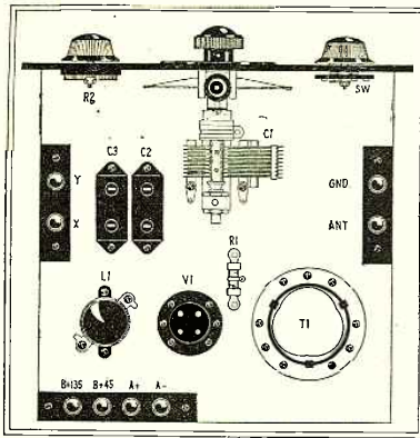
FIG. 2. THE LAYOUT OF THE PARTS IN THE ANTENNA STAGE WHICH IS ADDED TO THE ORIGINAL SET.
