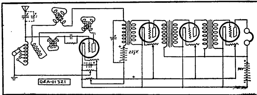
Circuit showing the A. J. Allen regenerative circuit adapted to 3-stage audio frequency amplifier. (Note: No condenser is used across phones and the 90-volt B battery may be less. Forty-five volts might be all right for UV-201, or Cunningham 301 tubes)
