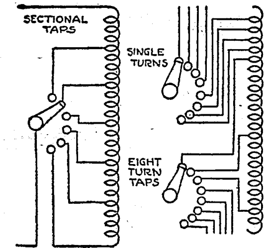
Figure 20--Two Methods of Varying Inductances with Taps
