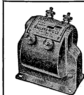
All-American Audio Frequency Transformer — comes in three ratios.
