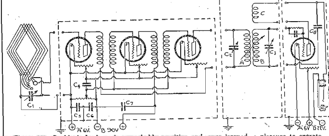
Figure 100—Gouden's hook-up is remarkably sensitive and, once learned, a pleasure to operate. next smaller size. C 2 and C 3 are .001 mfd each, as is C 4 . The leads to C 3 may have to be reversed to secure regeneration, but once determined are left alone. With two
