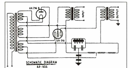
Fig. 1 - RCA AP-935 schematic
