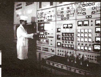
The huge Svetlana vacuum tube plant in St. Petersburg, Russia.
