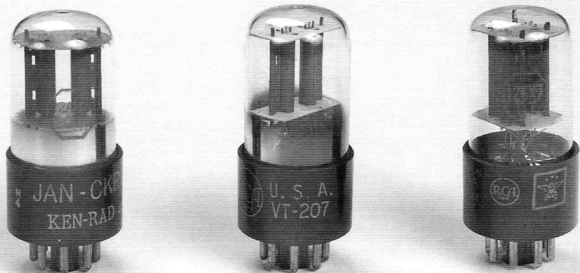
12SX7s - Ken Rad, RCA VT-207 and RCA (mid 1940s)
