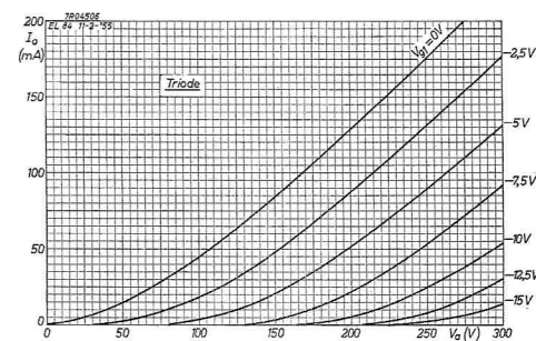
Original Philips EL84 data sheet and curves
