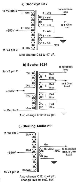
Figure 3 Output Transformer Connections
