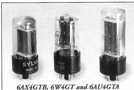
6AX4GTB, 6W4GT and 6AU4GTA
