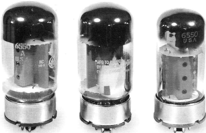
GE 6550A (1970s), GE 6550A (1992 MPD-reissue) and Philips-USA 6550 (1970s)
