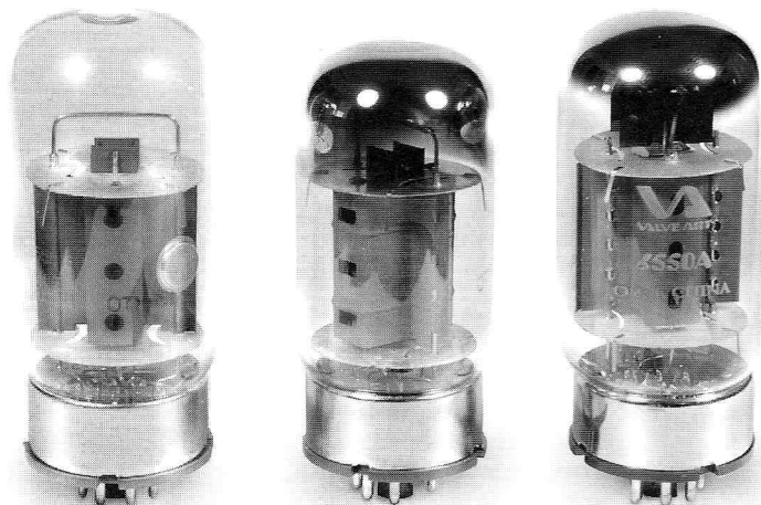
Svetlana SV6550B (early 1990s with pill getter), Svetlana SV6550C (2001) and Valve Arts Chinese 6550CA (2002)
